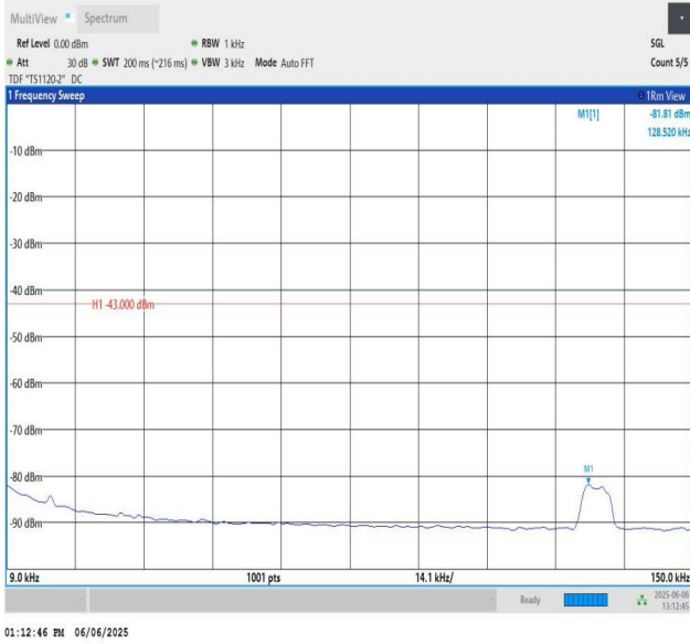
Band66-5MHz-QPSK-132647-PASS
