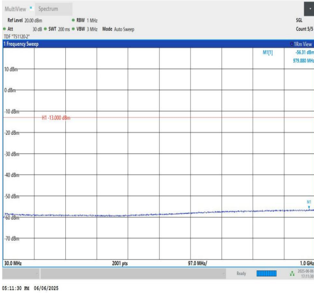
Band66-3MHz-QPSK-132657-PASS
