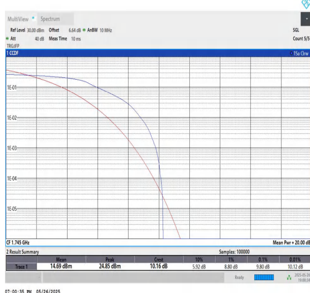
Band66-10MHz-16QAM-132322-PASS
