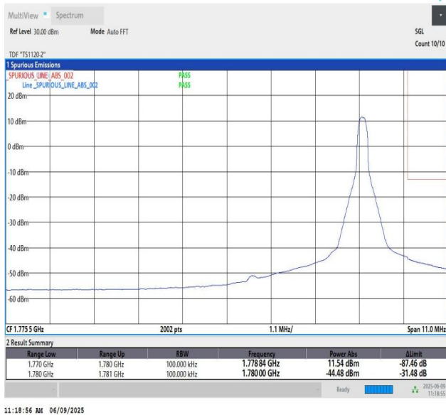
Band66_10MHz_QPSK_132622_1_High
