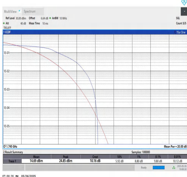
Band66-10MHz-QPSK-132322-PASS
