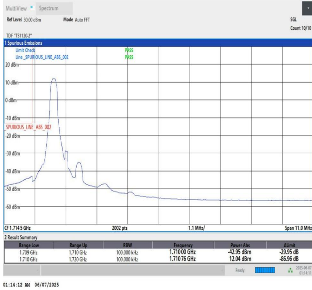
Band66_10MHz_QPSK_132022_1_Low
