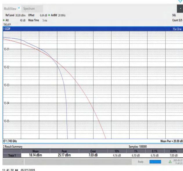
Band66-20MHz-QPSK-132322-PASS
