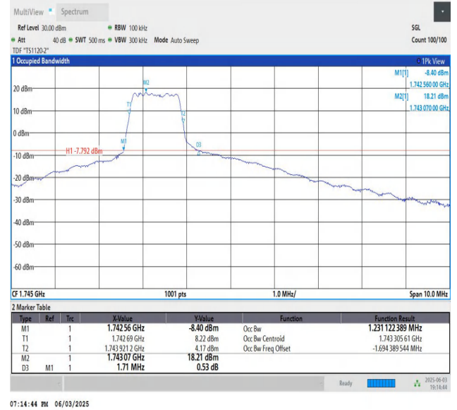
Band66-5MHz-16QAM-132322-PASS
