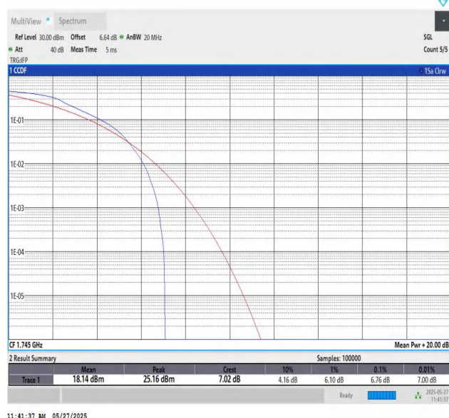
Band66-20MHz-16QAM-132322-PASS
