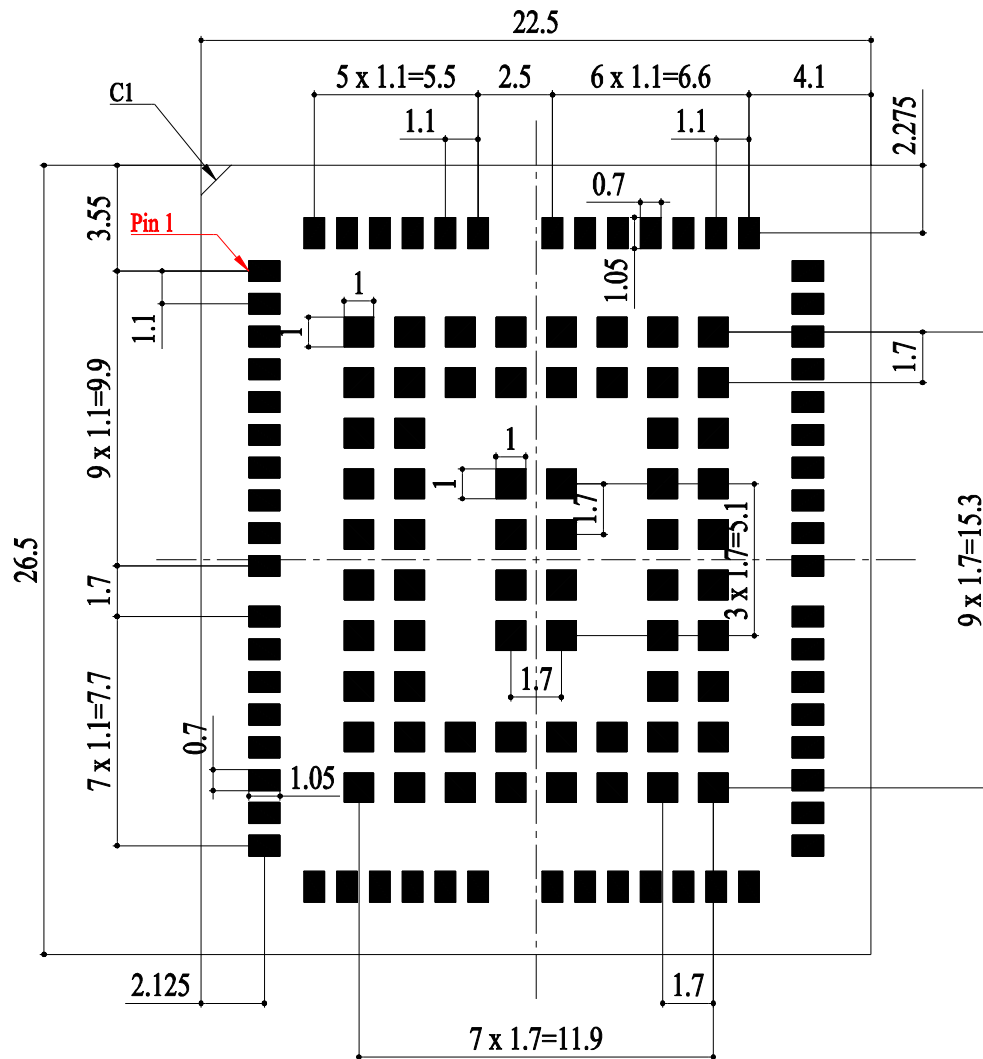
Figure 44: I4916Q-GL Recommended Footprint (Unit: mm)
