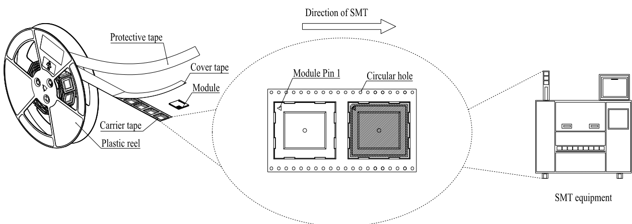
Figure 50: Mounting Direction
