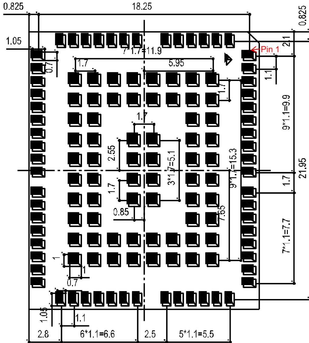
Figure 40: I4915Q Series Bottom Dimension (Bottom View, Unit: mm)
