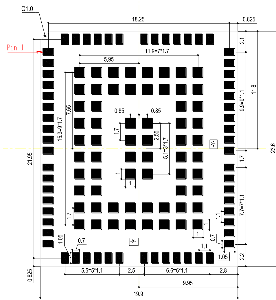
Figure 43: I4915Q Series Recommended Footprint (Unit: mm)
