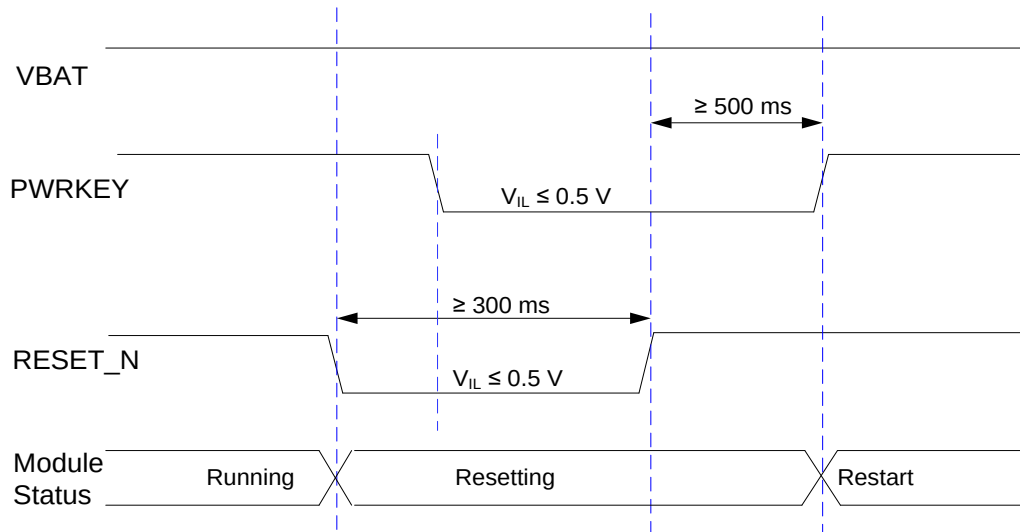
Figure 18: Reset Timing
