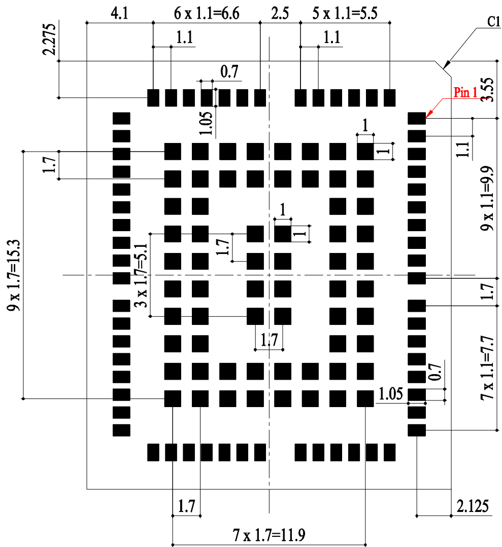
Figure 42: I4916Q-GL Bottom Dimension (Bottom View, Unit: mm)
