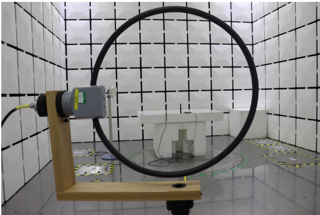
Below 30MHz
