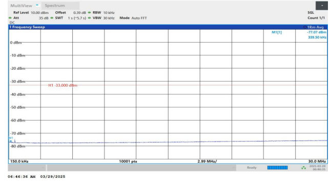
Band4-1312-3-0.15~30MHz-PASS
