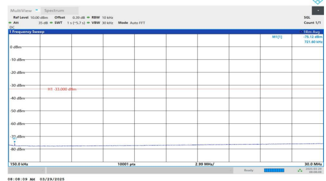
Band4-1413-1-0.15~30MHz-PASS
