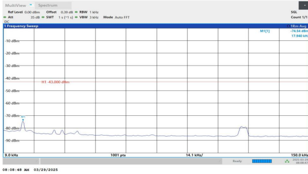
Band4-1513-1-0.009~0.15MHz-PASS
