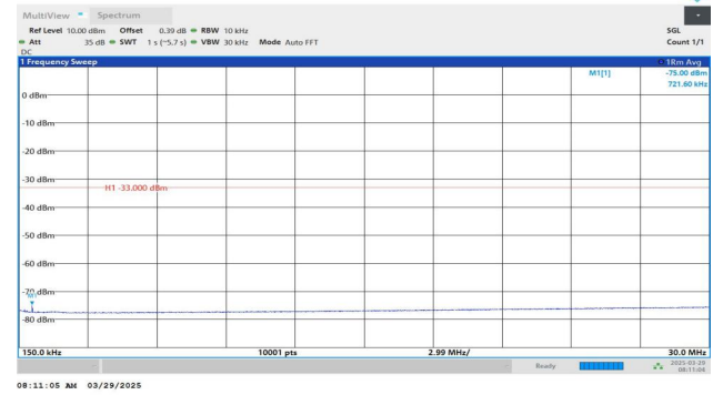
Band4-1413-2-0.15~30MHz-PASS
