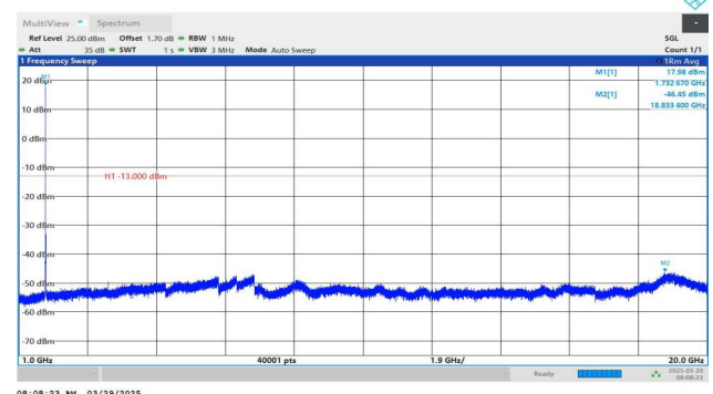
Band4-1413-1-1000~20000MHz-PASS
