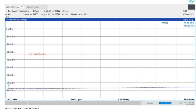
Band4-1312-2-0.15~30MHz-PASS
