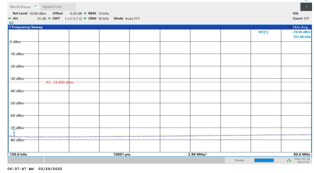
Band4-1413-1-0.15~30MHz-PASS
