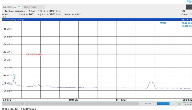
Band4-1413-5-0.009~0.15MHz-PASS
