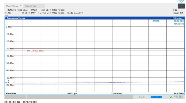
Band4-1312-4-0.15~30MHz-PASS
