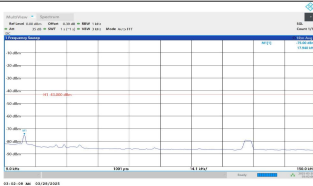
Band4-1413-0.009~0.15MHz-PASS
