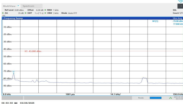
Band4-1312-4-0.009~0.15MHz-PASS
