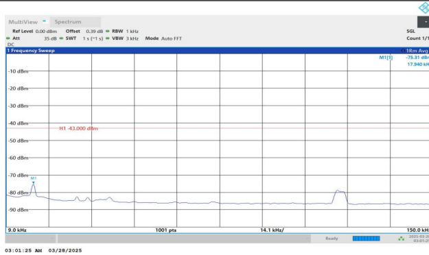
Band4-1312-0.009~0.15MHz-PASS
