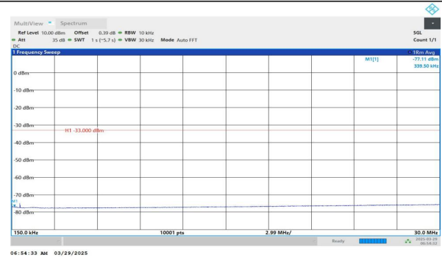
Band4-1413-4-0.15~30MHz-PASS
