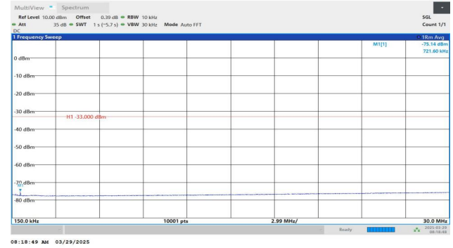
Band4-1312-5-0.15~30MHz-PASS
