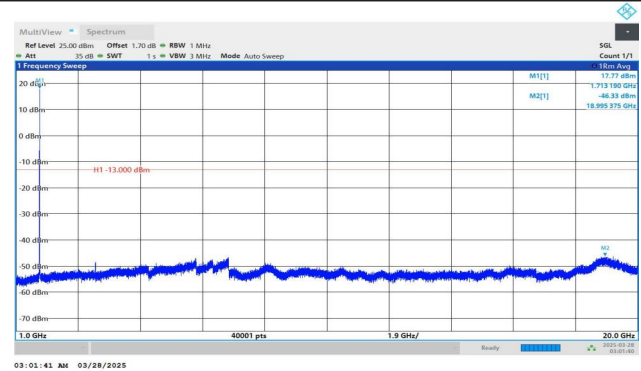
Band4-1312-1000~20000MHz-PASS
