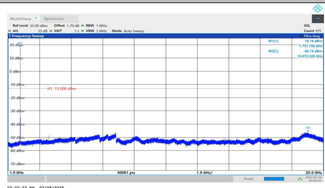
Band4-1413-1000~20000MHz-PASS
