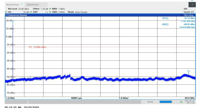
Band4-1513-2-1000~20000MHz-PASS
