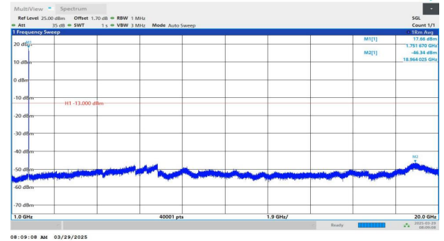
Band4-1513-1-1000~20000MHz-PASS
