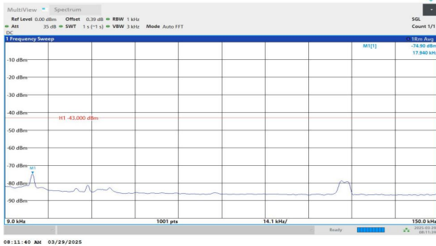
Band4-1513-2-0.009~0.15MHz-PASS
