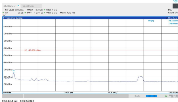
Band4-1413-3-0.009~0.15MHz-PASS
