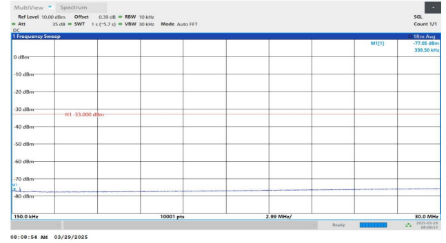
Band4-1513-1-0.15~30MHz-PASS
