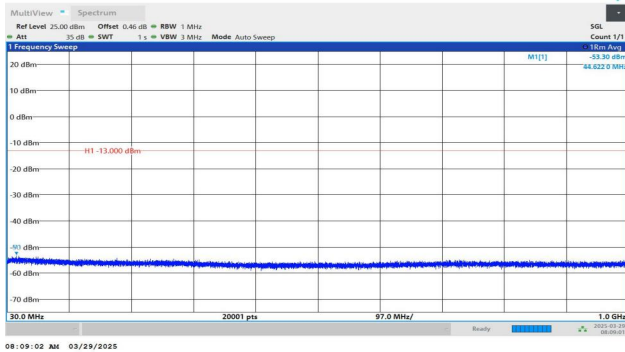
Band4-1513-1-30~1000MHz-PASS
