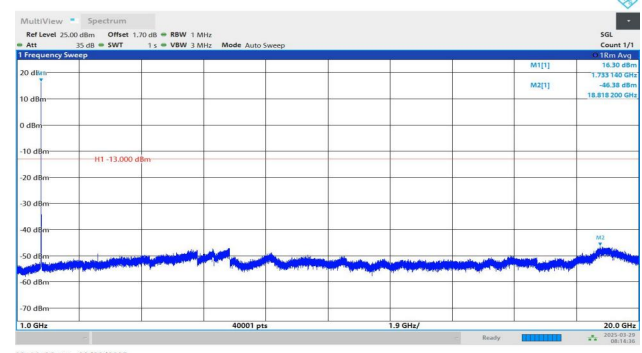
Band4-1413-3-1000~20000MHz-PASS
