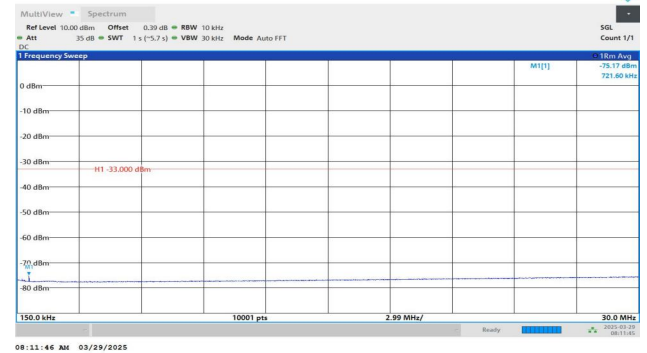
Band4-1513-2-0.15~30MHz-PASS
