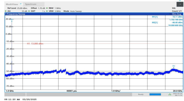
Band4-1413-2-1000~20000MHz-PASS
