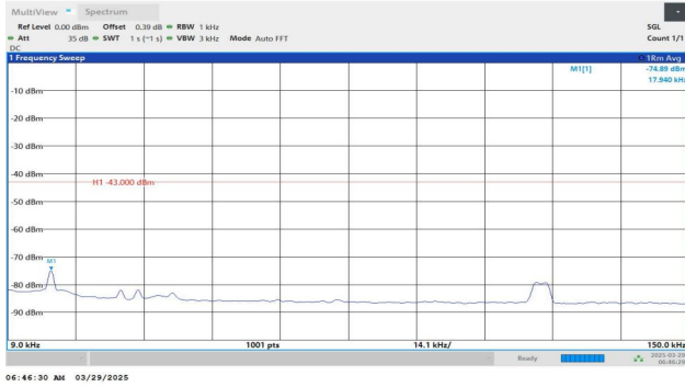
Band4-1312-3-0.009~0.15MHz-PASS
