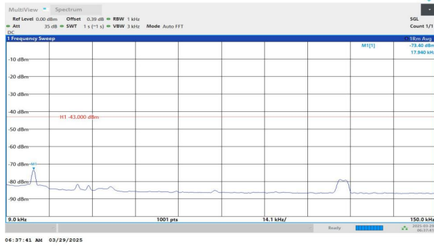
Band4-1413-1-0.009~0.15MHz-PASS
