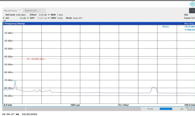
Band4-1413-4-0.009~0.15MHz-PASS
