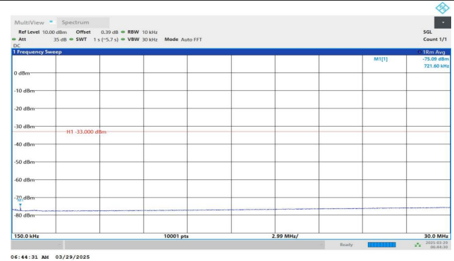
Band4-1312-2-0.15~30MHz-PASS
