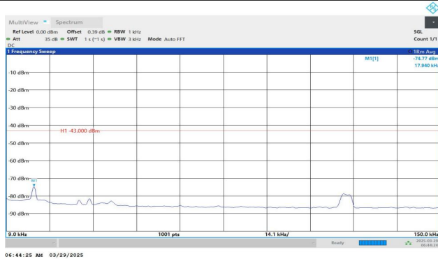
Band4-1312-2-0.009~0.15MHz-PASS
