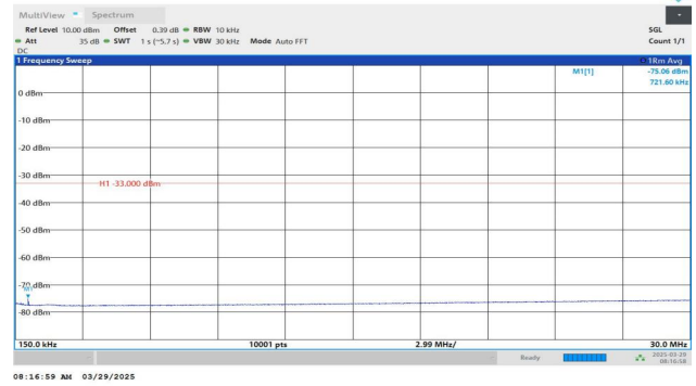
Band4-1413-4-0.15~30MHz-PASS
