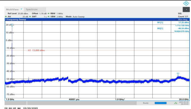
Band4-1312-2-1000~20000MHz-PASS
