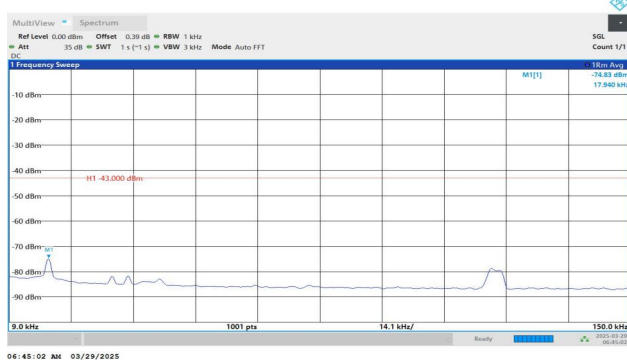
Band4-1413-2-0.009~0.15MHz-PASS
