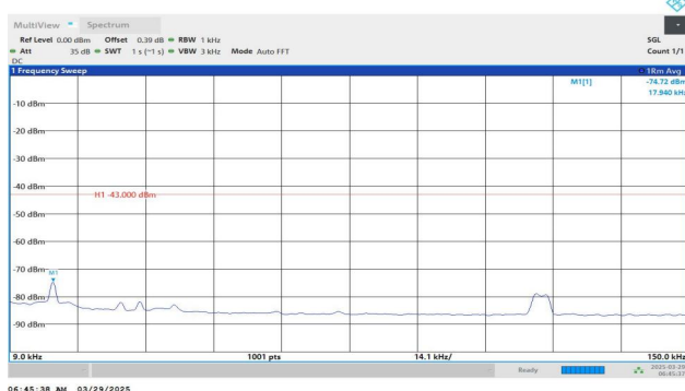
Band4-1513-2-0.009~0.15MHz-PASS
