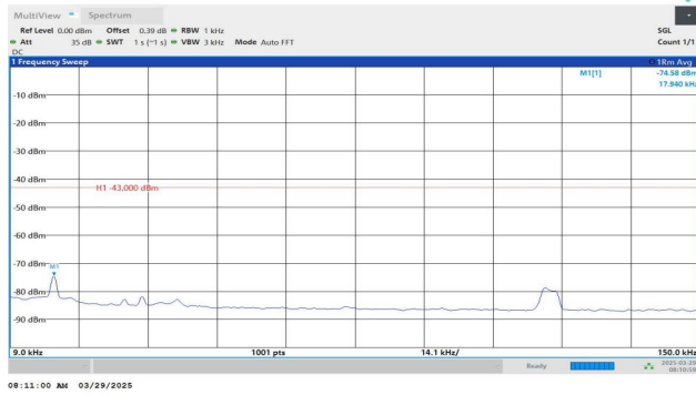
Band4-1413-2-0.009~0.15MHz-PASS
