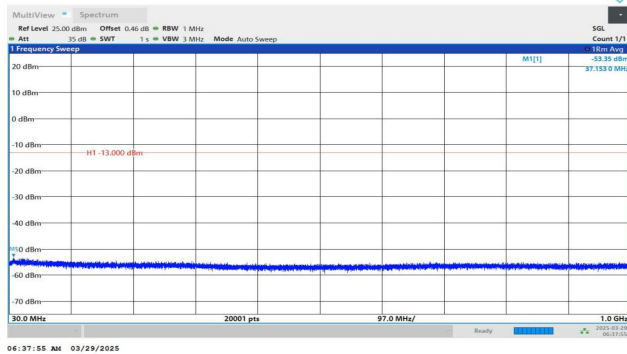
Band4-1413-1-30~1000MHz-PASS
