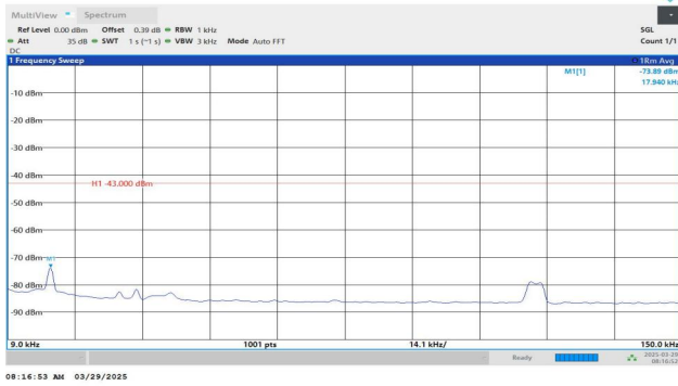
Band4-1413-4-0.009~0.15MHz-PASS
