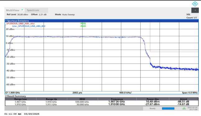
Band2-3MHz-QPSK-19185-15RB#0-PASS
