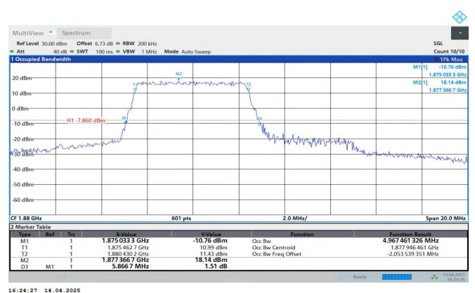
Band2-5MHz-16QAM-18900-25RB#0-PASS
