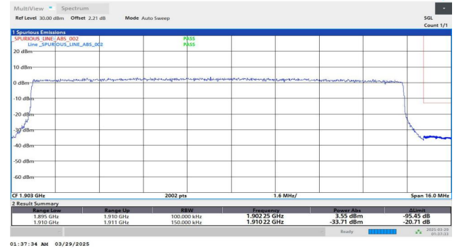
Band2-15MHz-QPSK-19125-1RB#74-PASS
