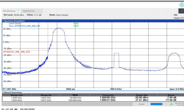
Band2-1.4MHz-QPSK-18607-1RB#0-PASS
