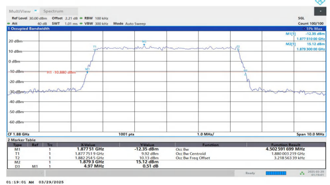
Band2-5MHz-16QAM-18900-25RB#0-PASS
