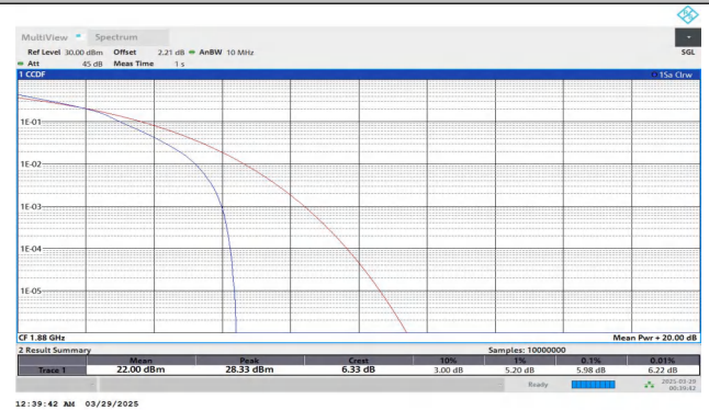
Band2-10MHz-16QAM-18900-27RB#0-PASS
