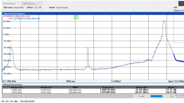
Band2-15MHz-QPSK-19125-1RB#0-PASS
