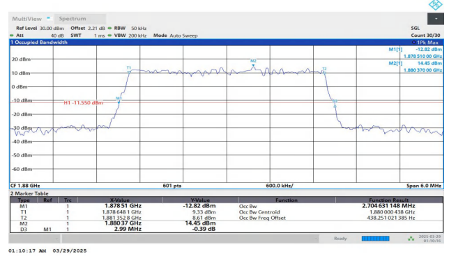
Band2-3MHz-16QAM-18900-15RB#0-PASS
