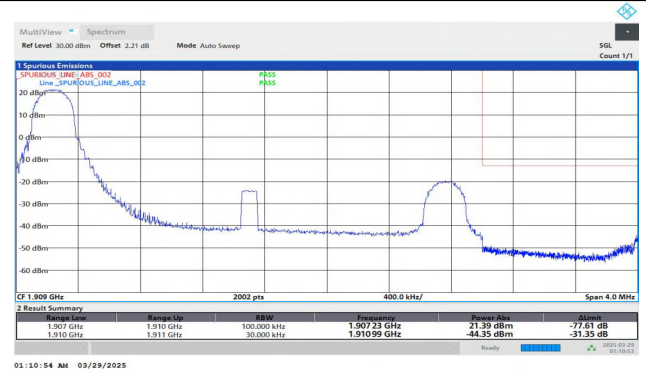
Band2-3MHz-QPSK-19185-1RB#0-PASS
