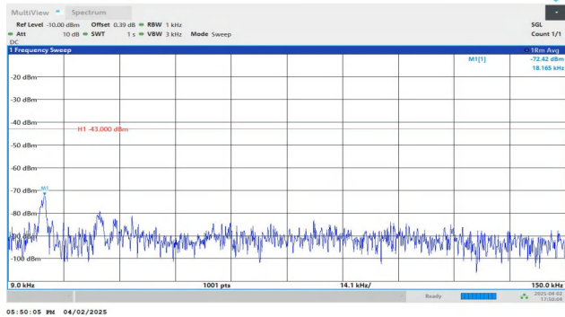
Band4-1.4MHz-QPSK-20175-1RB#0-0.009~0.15-PASS
