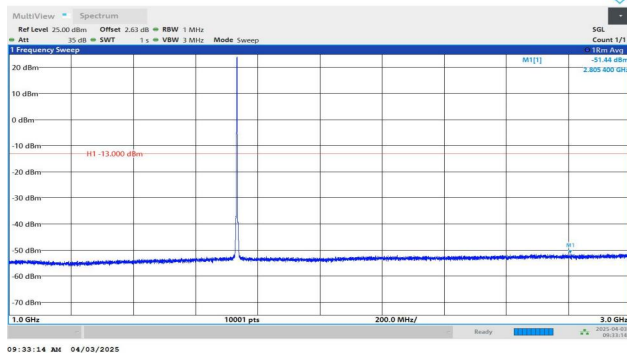
Band4-1.4MHz-QPSK-20175-1RB#5-1000~3000-PASS
