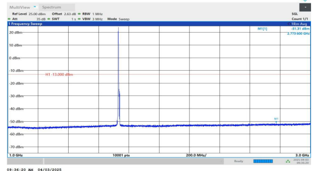
Band4-5MHz-QPSK-20175-1RB#0-1000~3000-PASS
