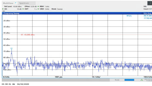
Band4-5MHz-QPSK-20375-1RB#0-0.009~0.15-PASS
