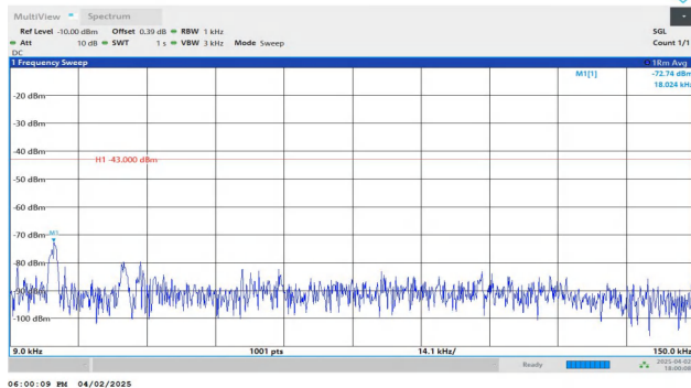
Band4-10MHz-QPSK-20000-1RB#0-0.009~0.15-PASS
