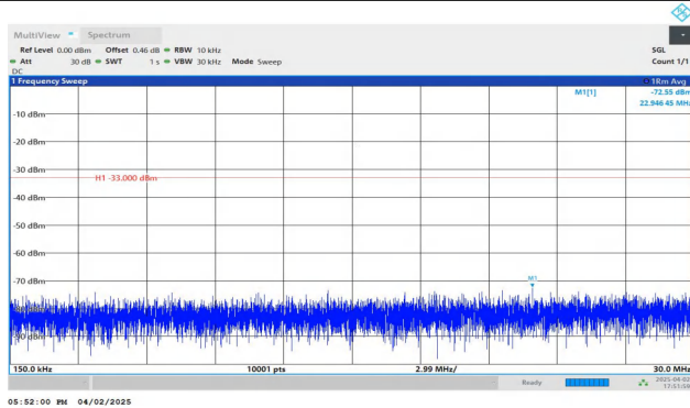
Band4-1.4MHz-QPSK-20393-1RB#5-0.15~30-PASS
