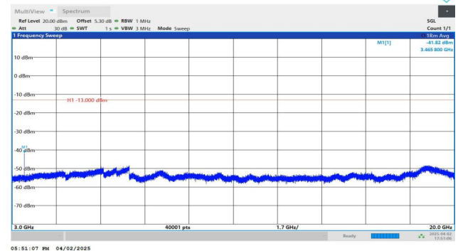
Band4-1.4MHz-QPSK-20175-1RB#5-3000~20000-PASS
