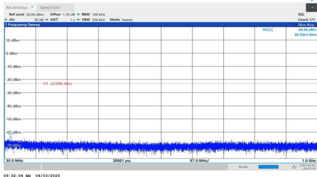
Band4-1.4MHz-QPSK-20175-1RB#0-30~1000-PASS
