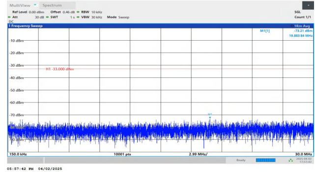
Band4-5MHz-QPSK-20175-1RB#0-0.15~30-PASS
