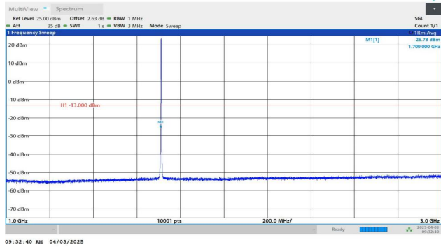
Band4-1.4MHz-QPSK-19957-1RB#5-1000~3000-PASS
