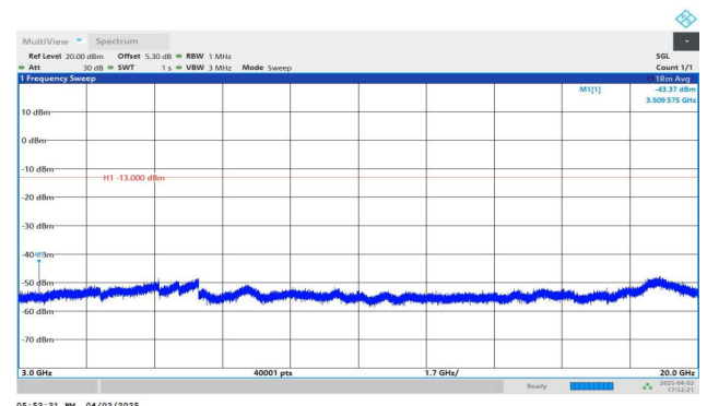
Band4-1.4MHz-QPSK-20393-1RB#5-3000~20000-PASS
