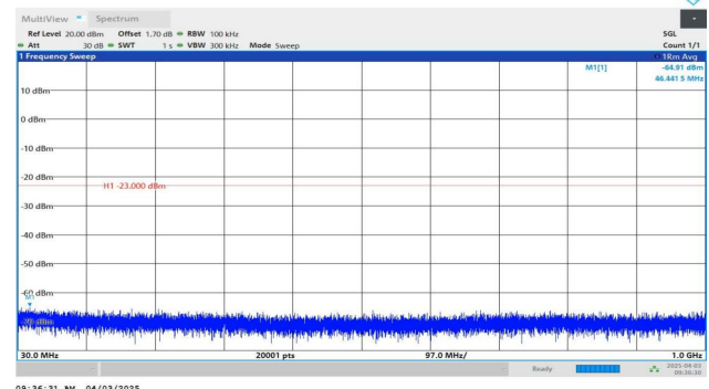
Band4-5MHz-QPSK-20175-1RB#24-30~1000-PASS
