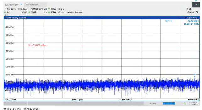
Band4-10MHz-QPSK-20000-1RB#0-0.15~30-PASS
