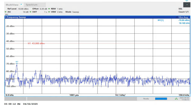
Band4-5MHz-QPSK-20175-1RB#24-0.009~0.15-PASS
