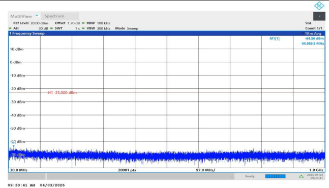
Band4-1.4MHz-QPSK-20393-1RB#5-30~1000-PASS
