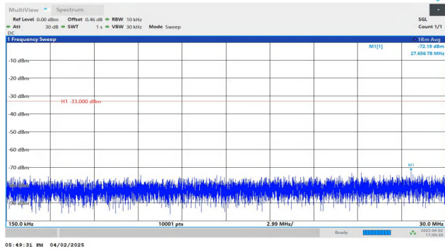
Band4-1.4MHz-QPSK-19957-1RB#5-0.15~30-PASS
