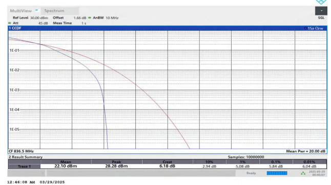
Band5-10MHz-16QAM-20525-27RB#0-PASS
