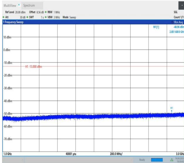
Band5-1.4MHz-QPSK-20407-1RB#5-1000~3000-PASS
