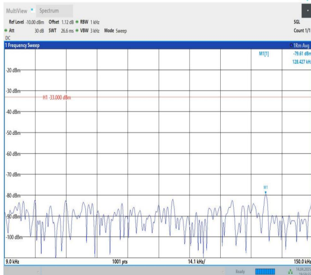
Band5-1.4MHz-QPSK-20525-1RB#0-0.009~0.15-PASS
