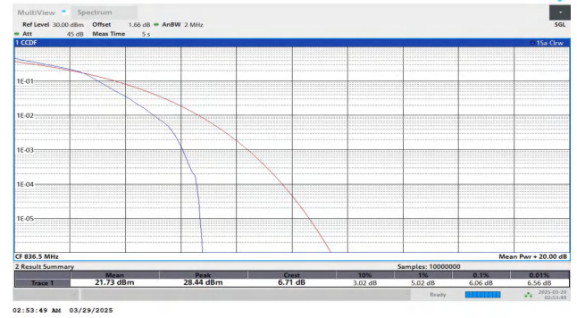
Band5-1.4MHz-16QAM-20525-6RB#0-PASS
