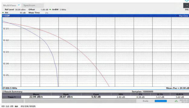
Band5-5MHz-QPSK-20525-25RB#0-PASS
