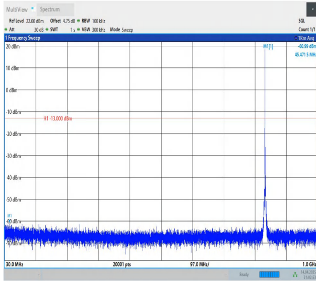
Band5-1.4MHz-QPSK-20525-1RB#0-30~1000-PASS
