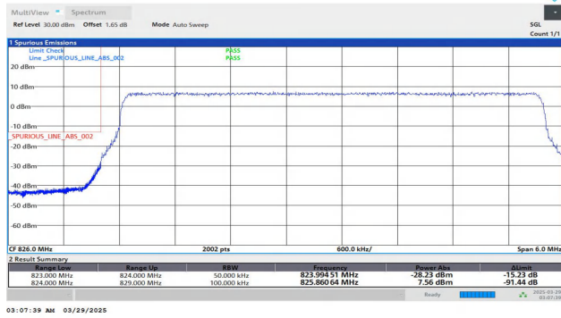
Band5-5MHz-QPSK-20425-25RB#0-PASS
