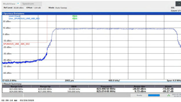
Band5-3MHz-QPSK-20415-15RB#0-PASS
