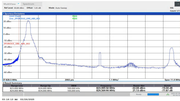
Band5-10MHz-QPSK-20450-1RB#0-PASS
