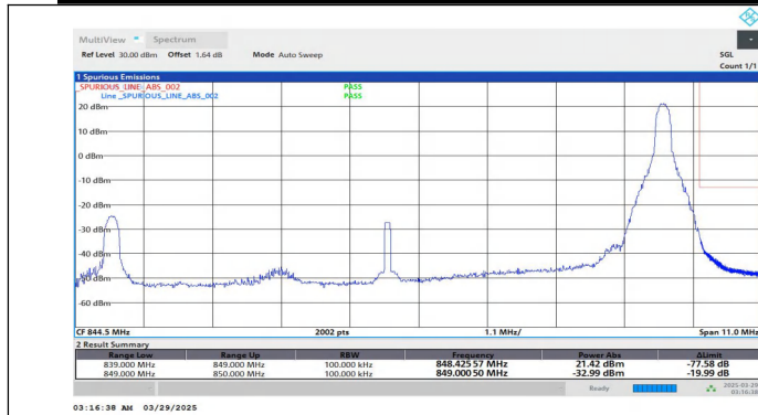
Band5-10MHz-QPSK-20600-1RB#49-PASS
