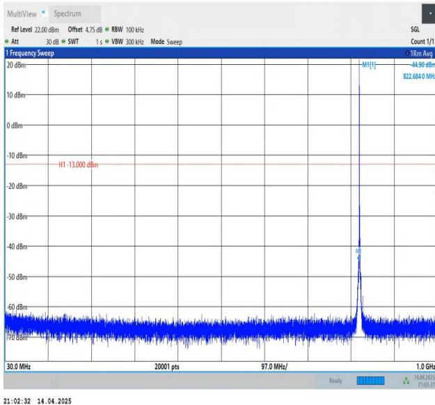
Band5-1.4MHz-QPSK-20407-1RB#0-30~1000-PASS
