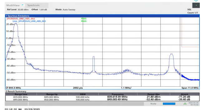
Band5-10MHz-QPSK-20600-1RB#0-PASS
