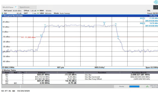
Band5-3MHz-QPSK-20525-15RB#0-PASS
