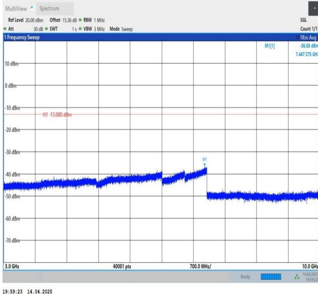
Band5-1.4MHz-QPSK-20407-1RB#0-3000~10000-PASS
