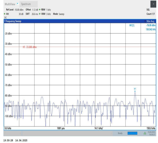
Band5-1.4MHz-QPSK-20407-1RB#5-0.009~0.15-PASS
