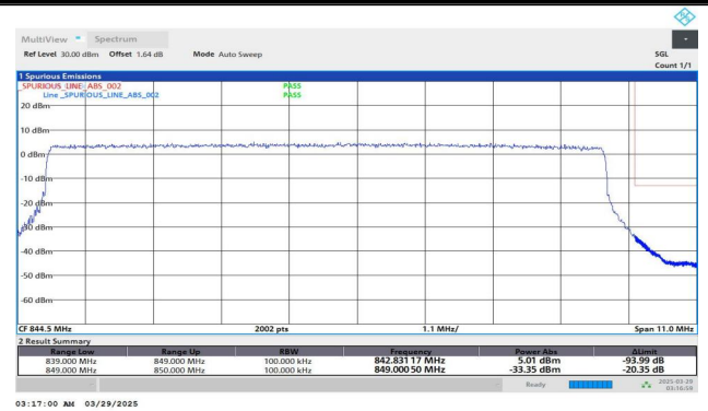
Band5-10MHz-QPSK-20600-50RB#0-PASS
