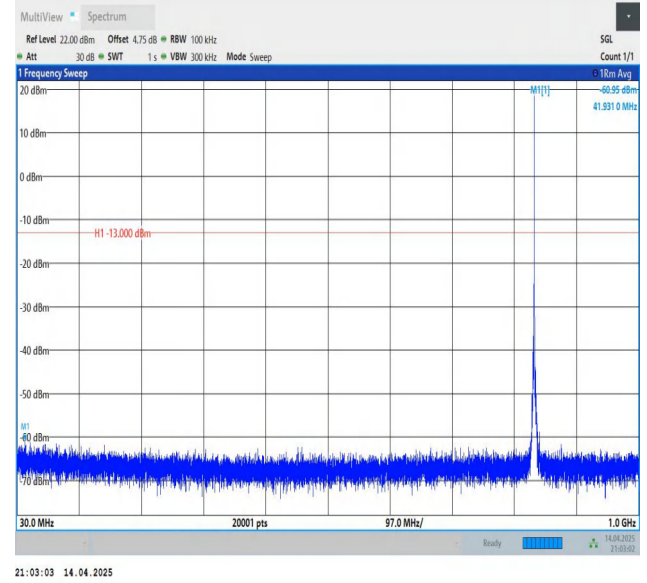
Band5-1.4MHz-QPSK-20525-1RB#5-30~1000-PASS
