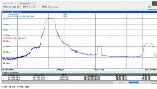
Band5-3MHz-QPSK-20415-1RB#0-PASS
