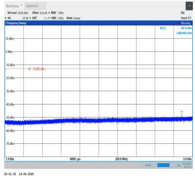
Band5-1.4MHz-QPSK-20643-1RB#0-1000~3000-PASS
