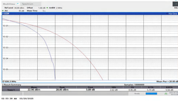
Band5-1.4MHz-QPSK-20525-6RB#0-PASS
