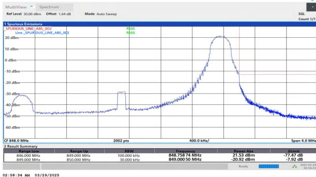
Band5-3MHz-QPSK-20635-1RB#14-PASS
