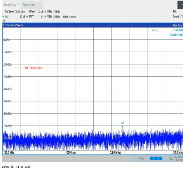
Band5-1.4MHz-QPSK-20525-1RB#5-0.15~30-PASS
