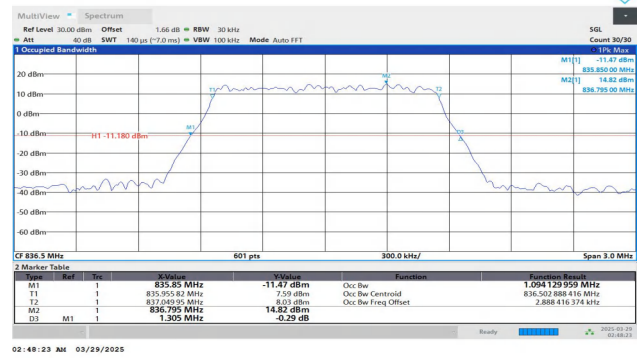
Band5-1.4MHz-16QAM-20525-6RB#0-PASS
