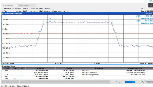
Band5-5MHz-QPSK-20525-25RB#0-PASS
