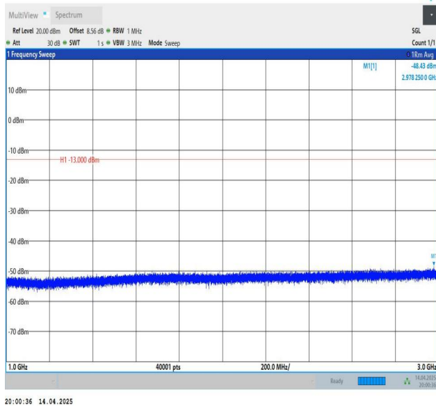
Band5-1.4MHz-QPSK-20525-1RB#5-1000~3000-PASS
