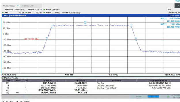
Band5-10MHz-QPSK-20525-50RB#0-PASS
