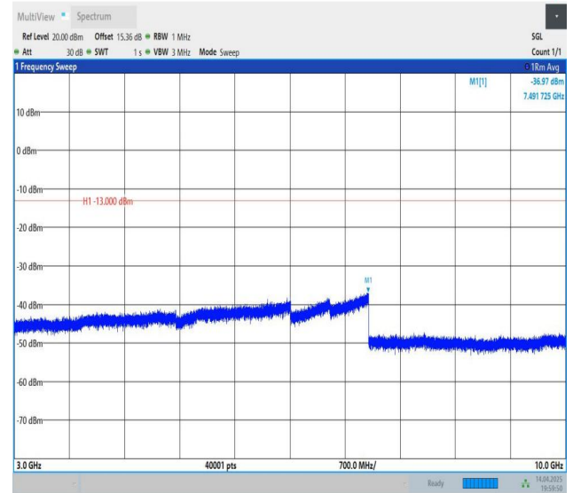
Band5-1.4MHz-QPSK-20407-1RB#5-3000~10000-PASS
