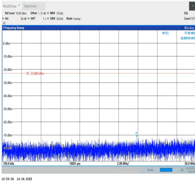
Band5-1.4MHz-QPSK-20407-1RB#5-0.15~30-PASS
