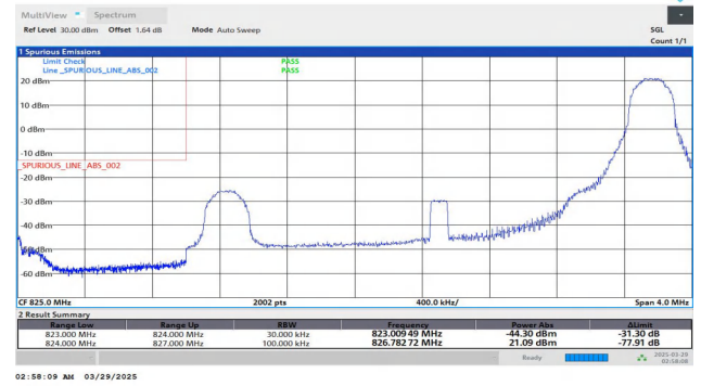
Band5-3MHz-QPSK-20415-1RB#14-PASS
