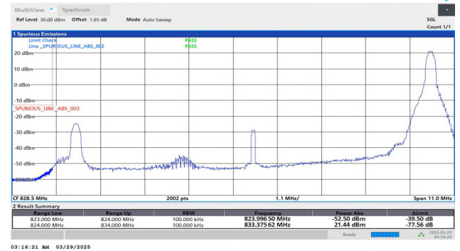
Band5-10MHz-QPSK-20450-1RB#49-PASS
