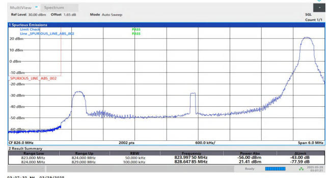
Band5-5MHz-QPSK-20425-1RB#24-PASS
