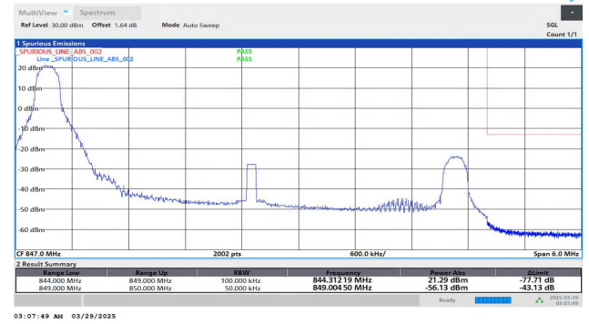
Band5-5MHz-QPSK-20625-1RB#0-PASS
