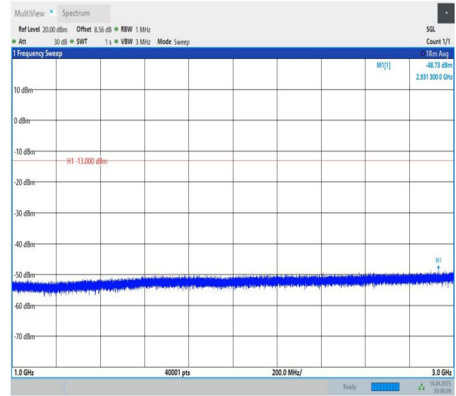
Band5-1.4MHz-QPSK-20525-1RB#0-1000~3000-PASS
