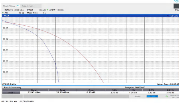
Band5-10MHz-QPSK-20525-50RB#0-PASS
