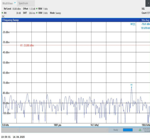
Band5-1.4MHz-QPSK-20407-1RB#0-0.009~0.15-PASS
