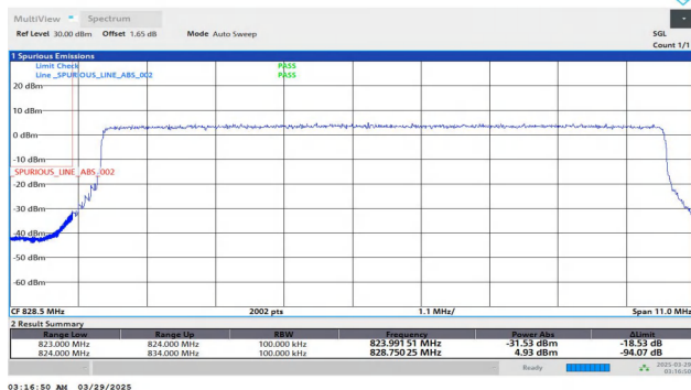
Band5-10MHz-QPSK-20450-50RB#0-PASS
