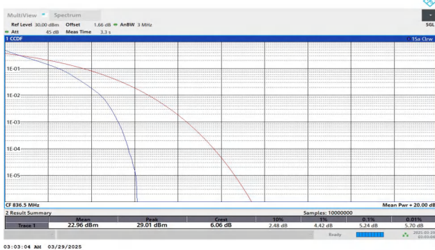
Band5-3MHz-QPSK-20525-15RB#0-PASS
