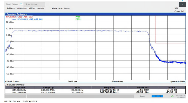
Band5-5MHz-QPSK-20625-25RB#0-PASS
