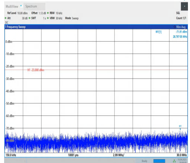
Band5-1.4MHz-QPSK-20525-1RB#0-0.15~30-PASS
