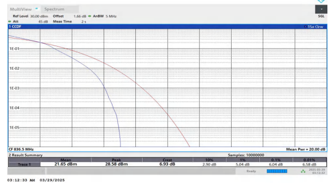
Band5-5MHz-16QAM-20525-25RB#0-PASS
