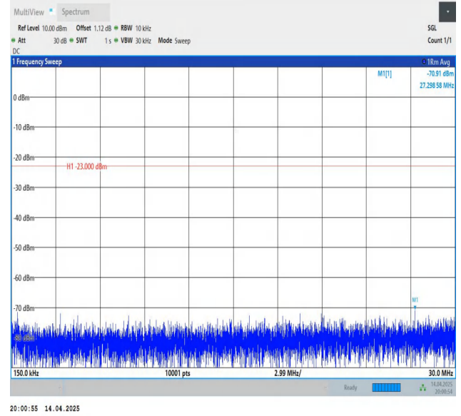
Band5-1.4MHz-QPSK-20643-1RB#0-0.15~30-PASS
