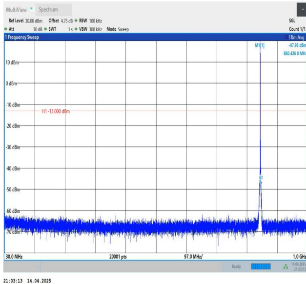
Band5-1.4MHz-QPSK-20643-1RB#0-30~1000-PASS
