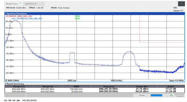
Band5-3MHz-QPSK-20635-1RB#0-PASS
