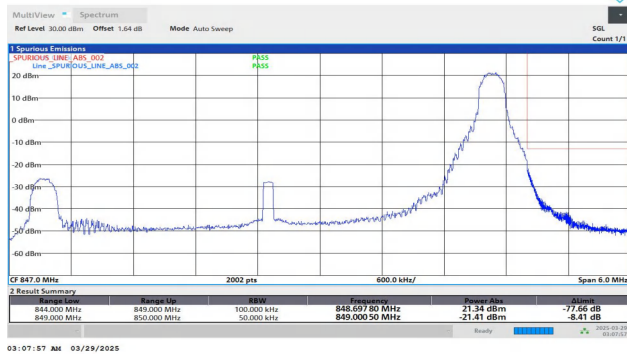
Band5-5MHz-QPSK-20625-1RB#24-PASS
