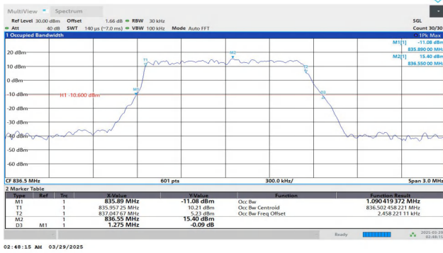
Band5-1.4MHz-QPSK-20525-6RB#0-PASS
