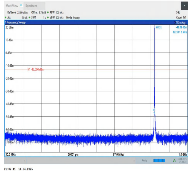
Band5-1.4MHz-QPSK-20407-1RB#5-30~1000-PASS
