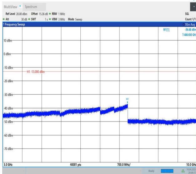
Band5-1.4MHz-QPSK-20525-1RB#0-3000~10000-PASS
