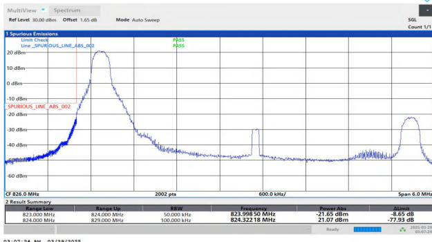
Band5-5MHz-QPSK-20425-1RB#0-PASS
