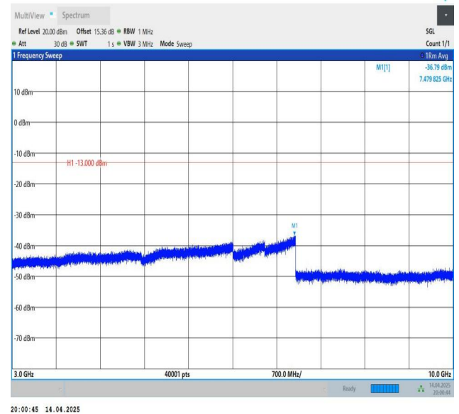
Band5-1.4MHz-QPSK-20525-1RB#5-3000~10000-PASS
