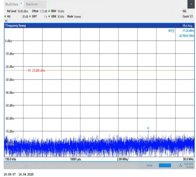
Band5-1.4MHz-QPSK-20407-1RB#0-0.15~30-PASS
