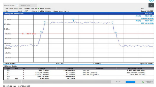
Band5-5MHz-16QAM-20525-25RB#0-PASS
