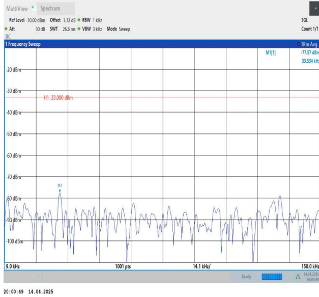
Band5-1.4MHz-QPSK-20643-1RB#0-0.009~0.15-PASS
