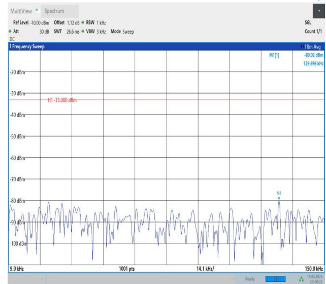
Band5-1.4MHz-QPSK-20525-1RB#5-0.009~0.15-PASS
