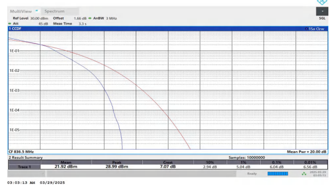
Band5-3MHz-16QAM-20525-15RB#0-PASS
