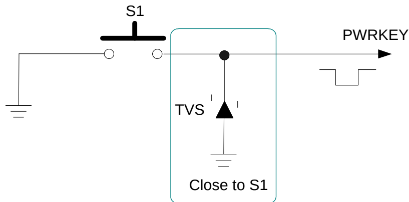
Figure 10: Turn On the Module Using a Button
