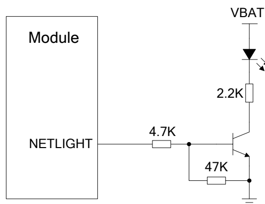
Figure 25: Reference Circuit of Network Status Indication
