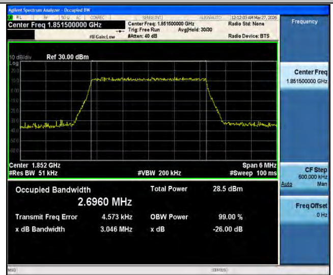
Band25-3MHz-256QAM-26055-15RB#0-PASS
