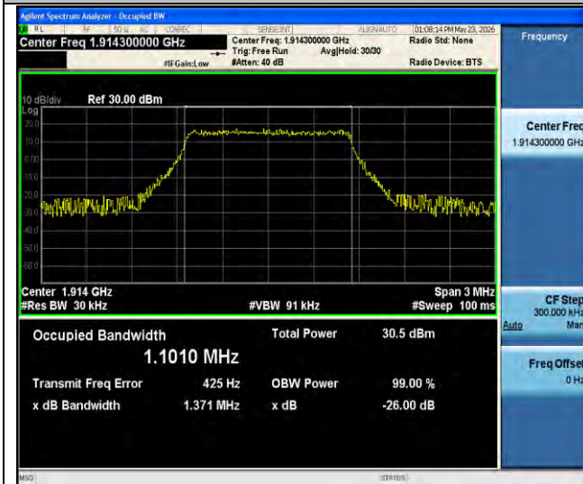
Band25-1.4MHz-64QAM-26683-6RB#0-PASS
