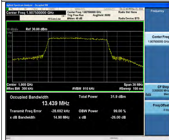
Band25-15MHz-64QAM-26615-75RB#0-PASS
