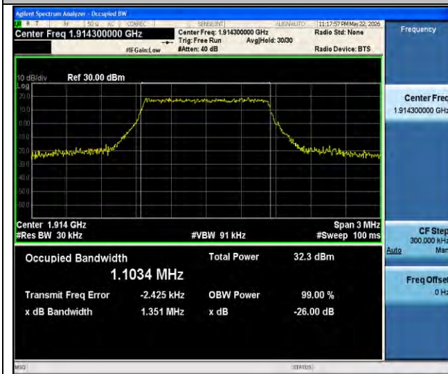
Band25-1.4MHz-QPSK-26683-6RB#0-PASS
