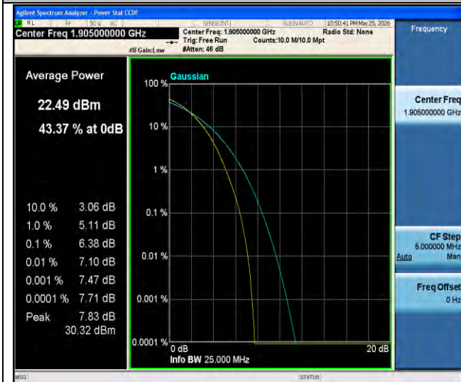
Band25-20MHz-64QAM-26590-100RB#0-PASS
