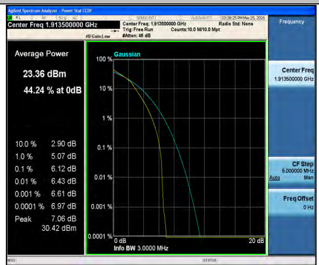
Band25-3MHz-16QAM-26675-15RB#0-PASS
