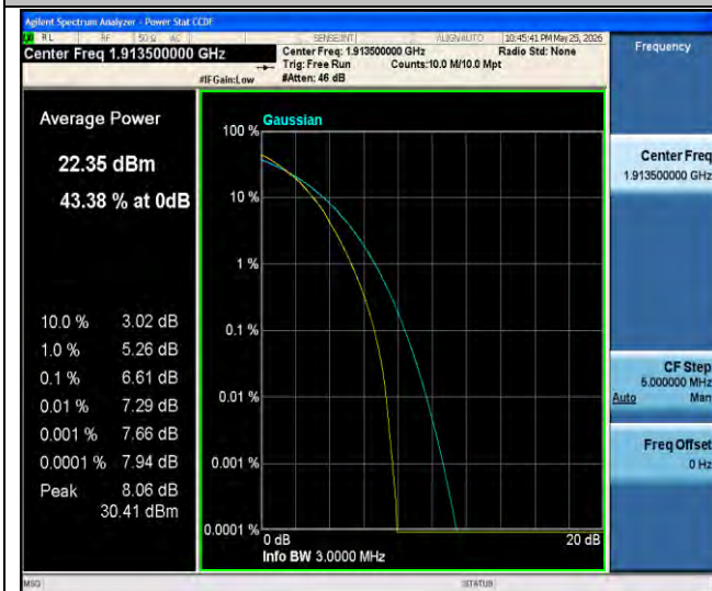
Band25-3MHz-64QAM-26675-15RB#0-PASS
