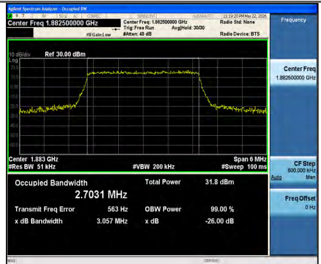
Band25-3MHz-16QAM-26365-15RB#0-PASS
