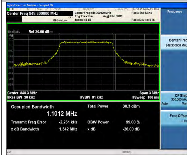
Band26(824-849)-1.4MHz-64QAM-27033-6RB#0-PASS
