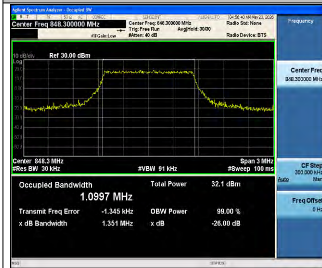
Band26(824-849)-1.4MHz-QPSK-27033-6RB#0-PASS
