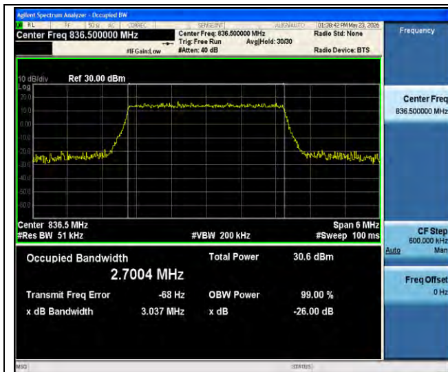
Band26(824-849)-3MHz-64QAM-26915-15RB#0-PASS
