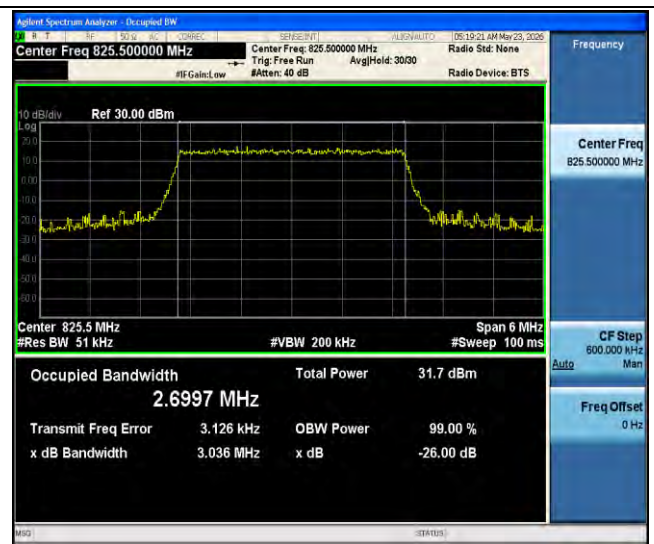
Band26(824-849)-3MHz-16QAM-26805-15RB#0-PASS
