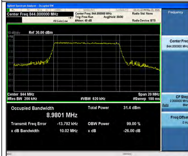
Band26(824-849)-10MHz-64QAM-26990-50RB#0-PASS
