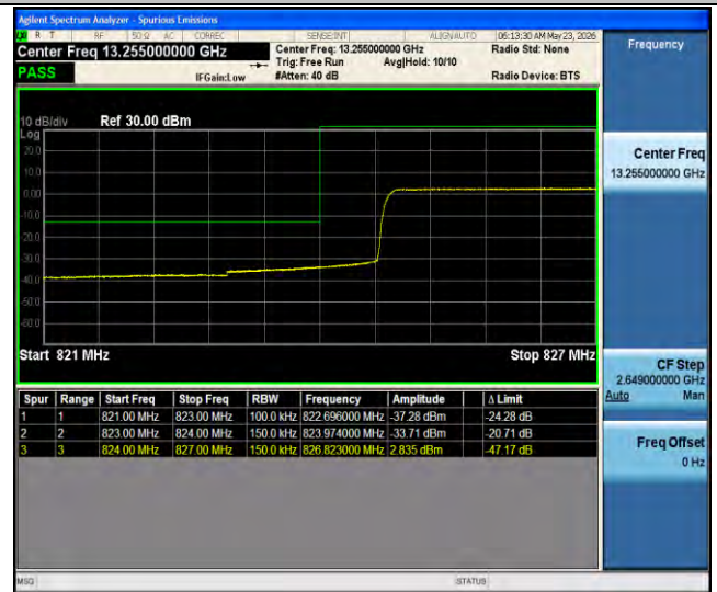
Band26(824-849)-15MHz-QPSK-26865-75RB#0-PASS
