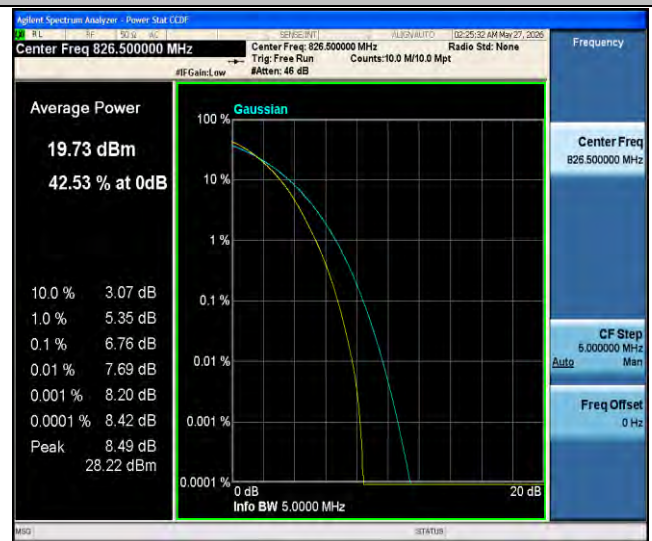
Band26(824-849)-5MHz-256QAM-26815-25RB#0-PASS
