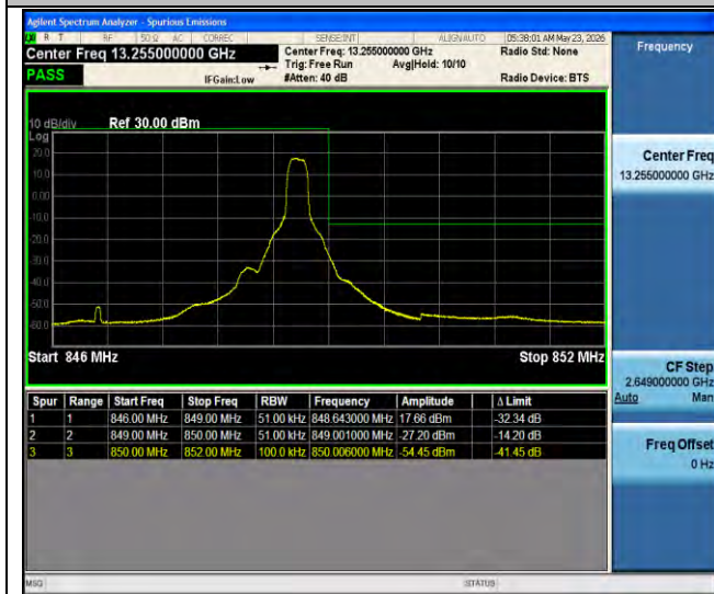
Band26(824-849)-5MHz-QPSK-27015-1RB#24-PASS
