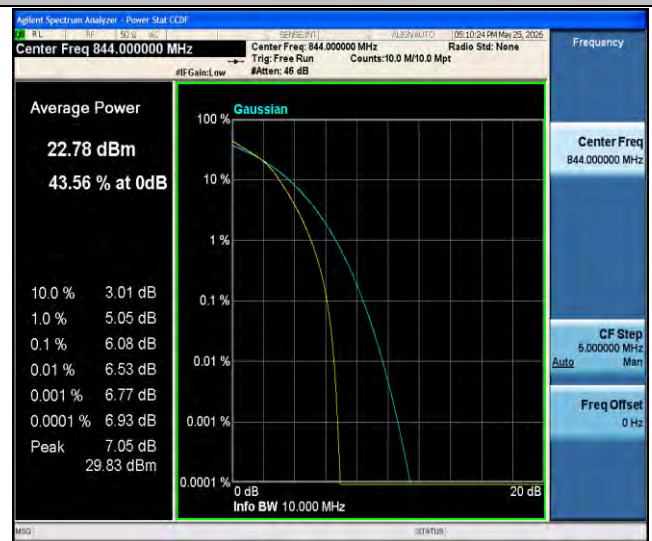
Band26(824-849)-10MHz-16QAM-26990-50RB#0-PASS
