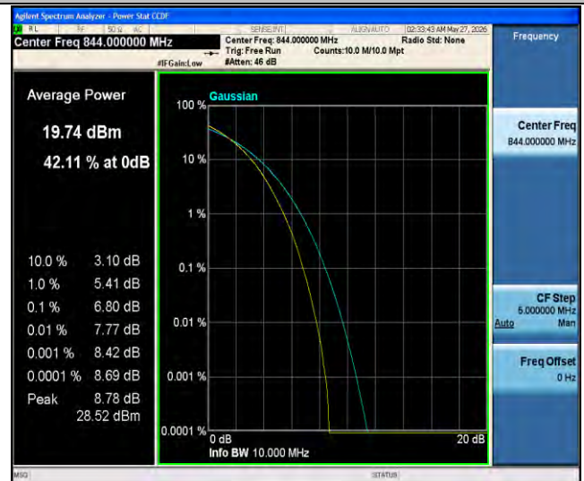
Band26(824-849)-10MHz-256QAM-26990-50RB#0-PASS
