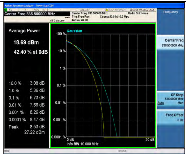
Band26(824-849)-10MHz-256QAM-26915-50RB#0-PASS
