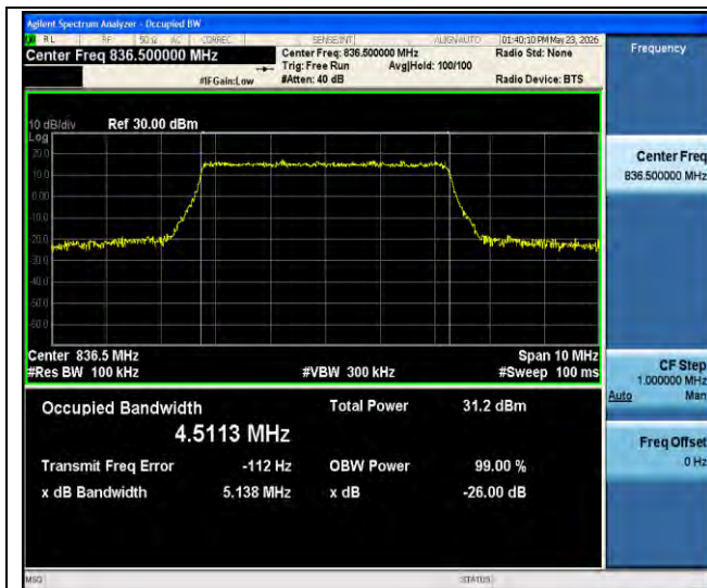
Band26(824-849)-5MHz-64QAM-26915-25RB#0-PASS
