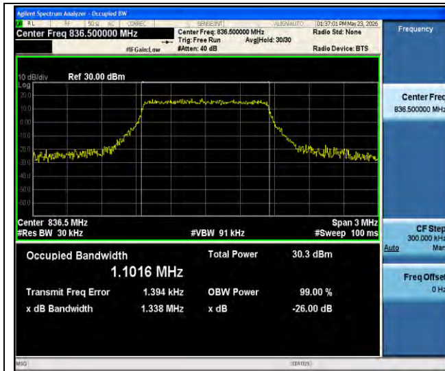
Band26(824-849)-1.4MHz-64QAM-26915-6RB#0-PASS
