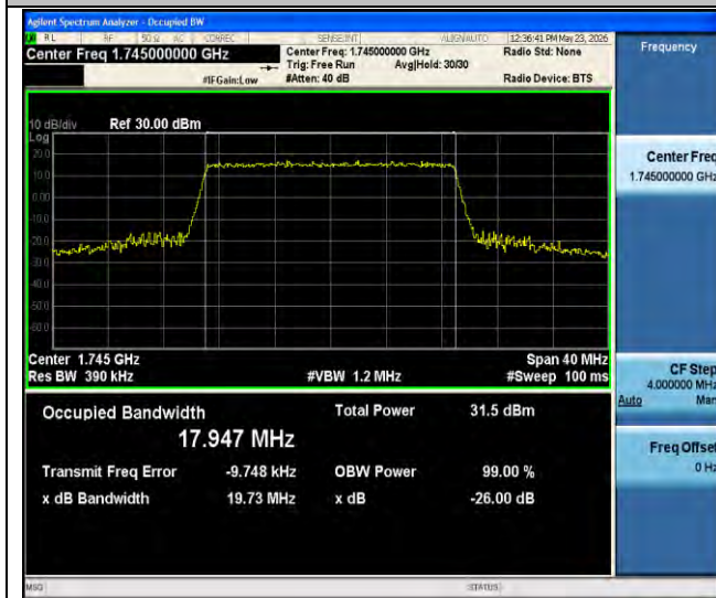
Band4-20MHz-64QAM-20300-100RB#0-PASS
