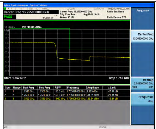
Band4-15MHz-QPSK-20325-75RB#0-PASS
