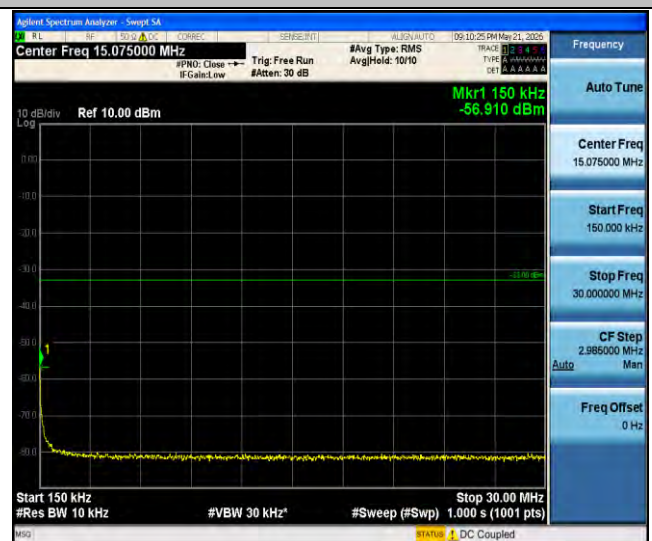
Band4-20MHz-QPSK-20300-1RB#0-0.15~30-PASS
