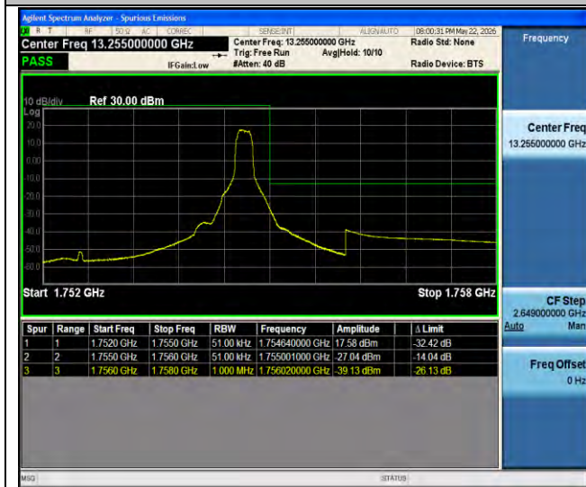
Band4-5MHz-QPSK-20375-1RB#24-PASS
