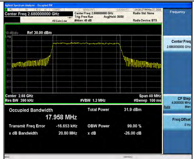
Band41-20MHz-256QAM-41490-100RB#0-PASS
