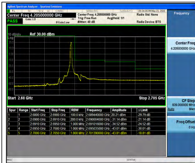
Band41-10MHz-QPSK-41540-1RB#49-PASS
