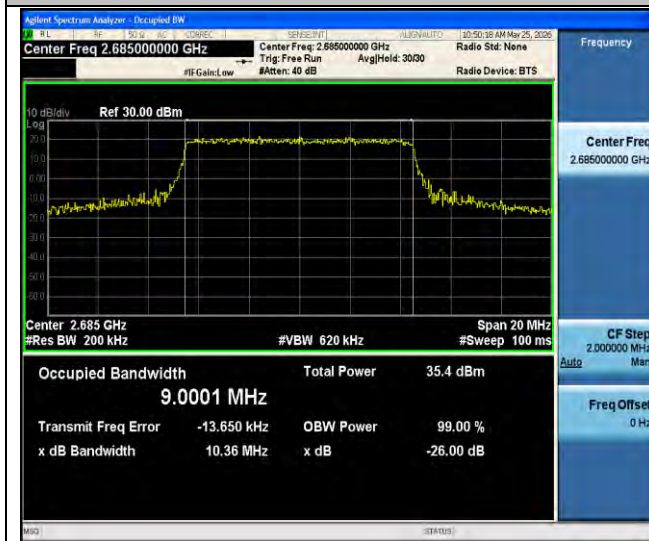
Band41-10MHz-QPSK-41540-50RB#0-PASS
