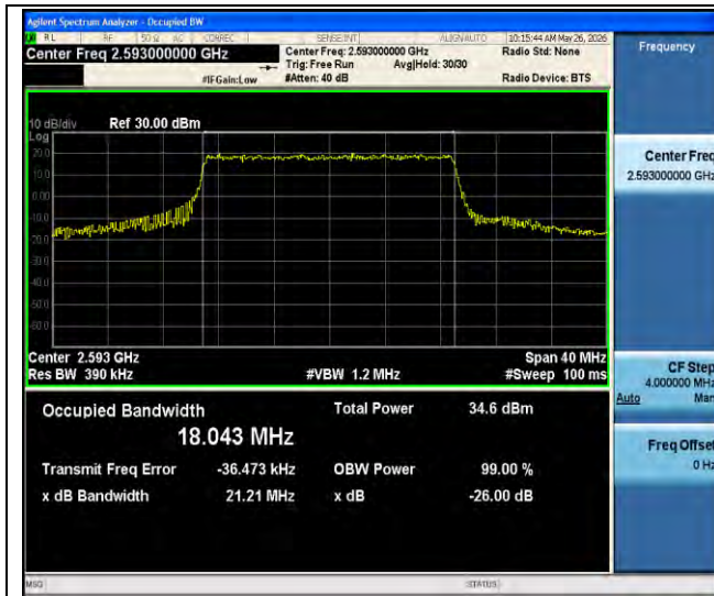
Band41-20MHz-64QAM-40620-100RB#0-PASS
