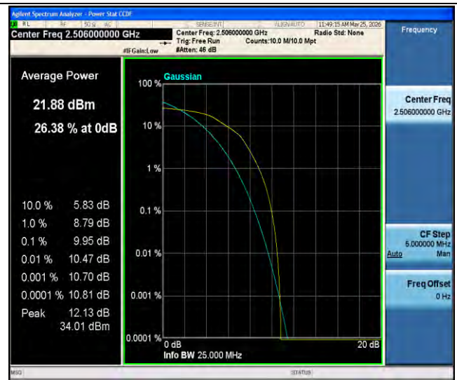
Band41-20MHz-16QAM-39750-100RB#0-PASS
