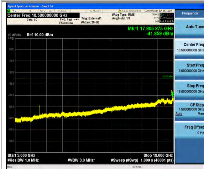
Band41-20MHz-QPSK-41490-1RB#0-3000~18000-PASS
