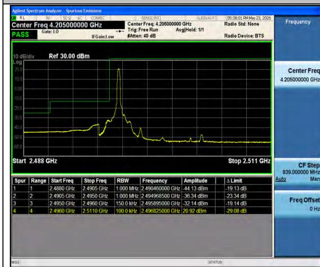
Band41-15MHz-QPSK-39725-1RB#0-PASS
