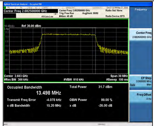
Band41-15MHz-256QAM-41515-75RB#0-PASS
