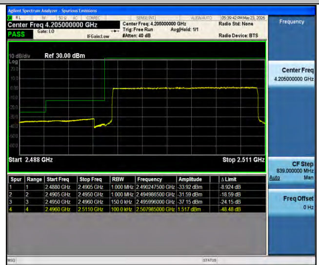
Band41-15MHz-QPSK-39725-75RB#0-PASS
