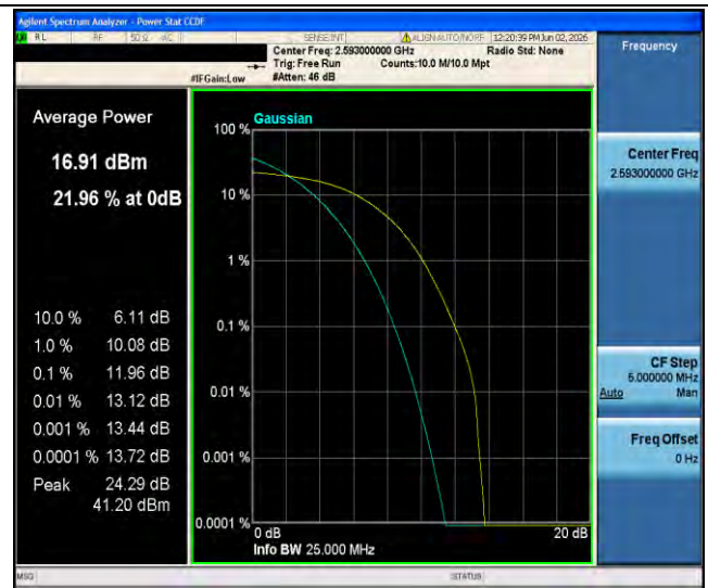
Band41-20MHz-256QAM-40620-100RB#0-PASS
