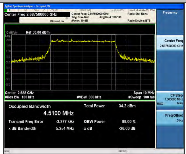
Band41-5MHz-16QAM-41565-25RB#0-PASS
