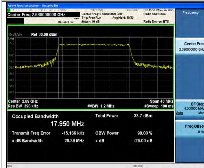
Band41-20MHz-64QAM-41490-100RB#0-PASS
