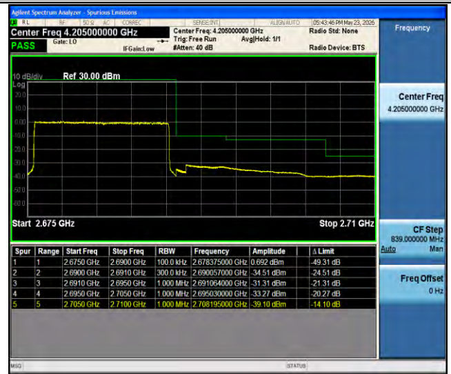
Band41-15MHz-QPSK-41515-75RB#0-PASS
