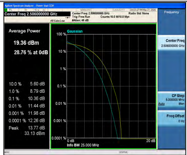
Band41-20MHz-256QAM-39750-100RB#0-PASS
