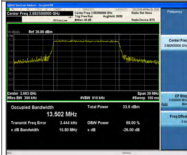
Band41-15MHz-64QAM-41515-75RB#0-PASS
