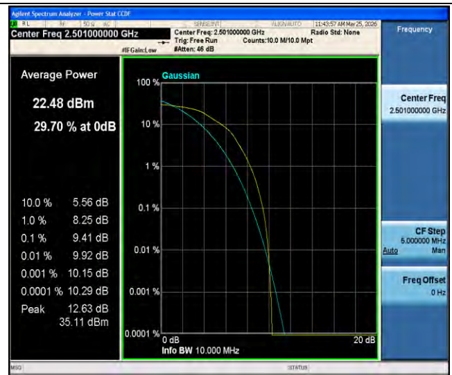
Band41-10MHz-16QAM-39700-50RB#0-PASS
