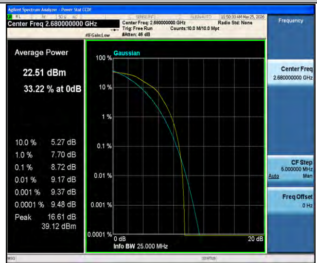
Band41-20MHz-16QAM-41490-100RB#0-PASS
