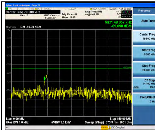
Band41-20MHz-QPSK-41490-1RB#0-0.009~0.15-PASS
