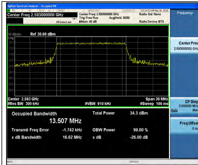
Band41-15MHz-64QAM-40620-75RB#0-PASS
