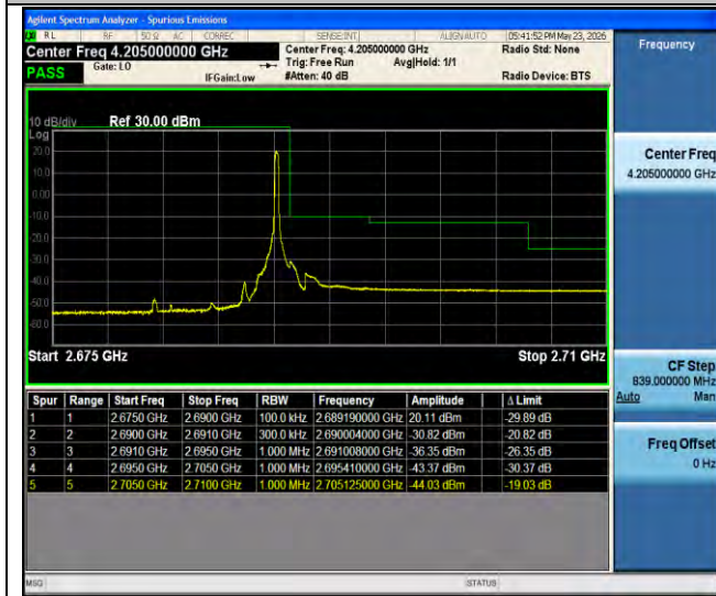
Band41-15MHz-QPSK-41515-1RB#74-PASS
