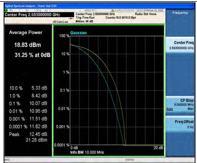
Band41-10MHz-256QAM-40620-50RB#0-PASS
