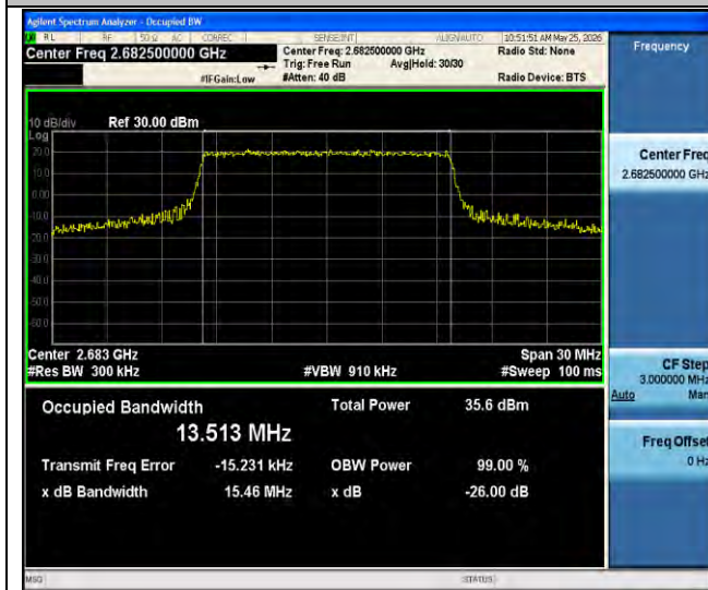
Band41-15MHz-QPSK-41515-75RB#0-PASS
