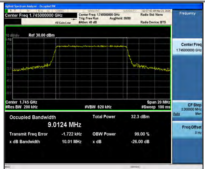
Band66-10MHz-16QAM-132322-50RB#0-PASS
