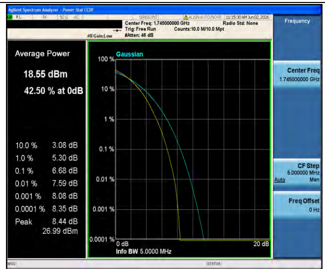
Band66-5MHz-256QAM-132322-25RB#0-PASS
