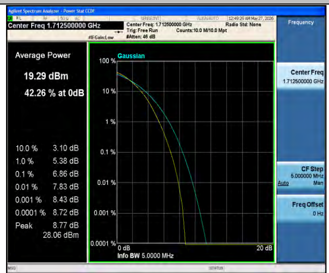
Band66-5MHz-256QAM-131997-25RB#0-PASS
