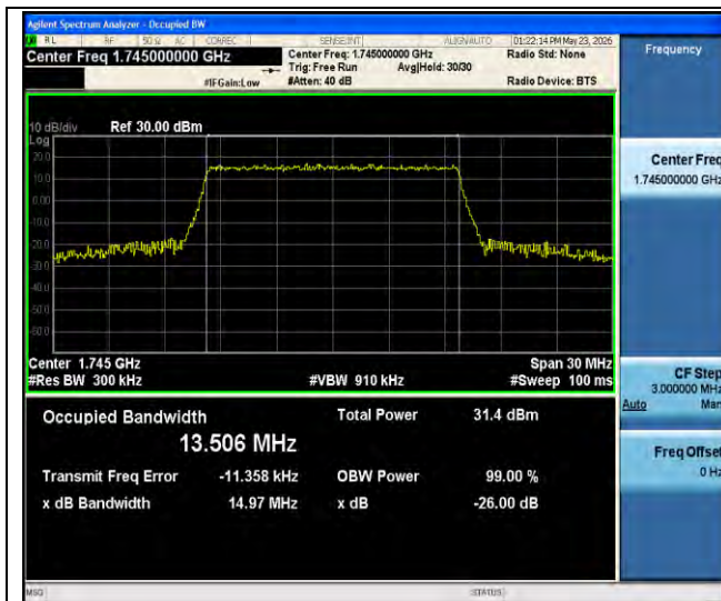
Band66-15MHz-64QAM-132322-75RB#0-PASS
