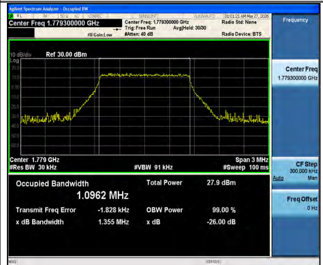
Band66-1.4MHz-256QAM-132665-6RB#0-PASS
