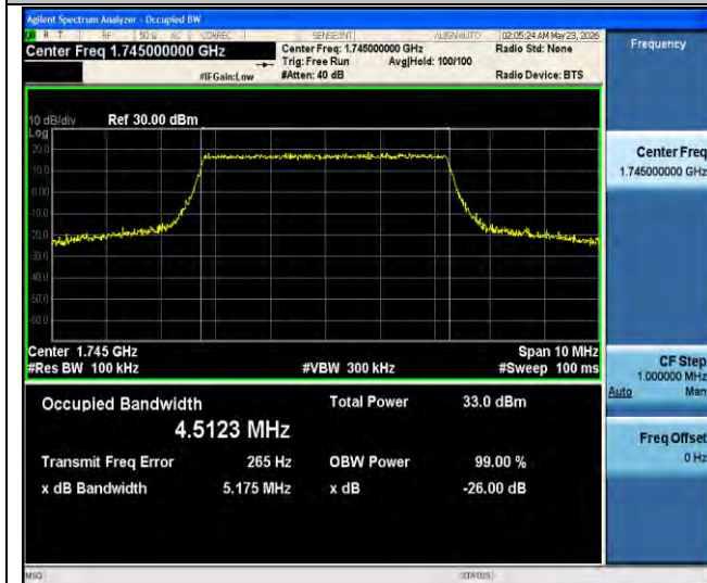
Band66-5MHz-QPSK-132322-25RB#0-PASS
