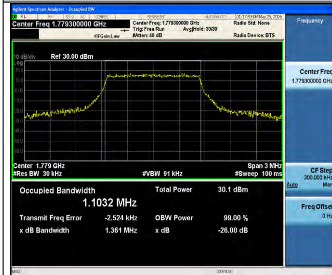
Band66-1.4MHz-64QAM-132665-6RB#0-PASS
