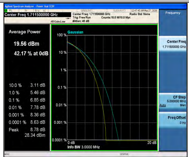
Band66-3MHz-256QAM-131987-15RB#0-PASS
