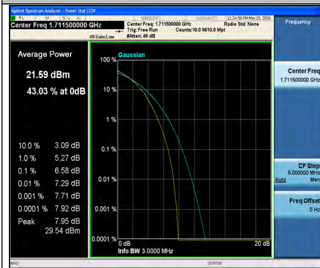
Band66-3MHz-64QAM-131987-15RB#0-PASS
