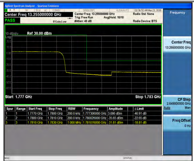
Band66-20MHz-QPSK-132572-100RB#0-PASS
