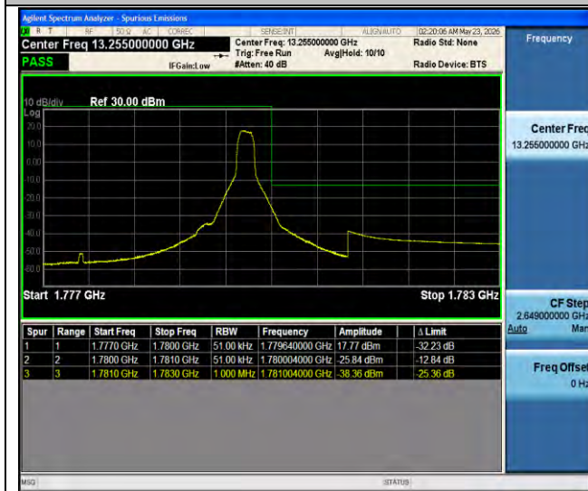
Band66-5MHz-QPSK-132647-1RB#24-PASS
