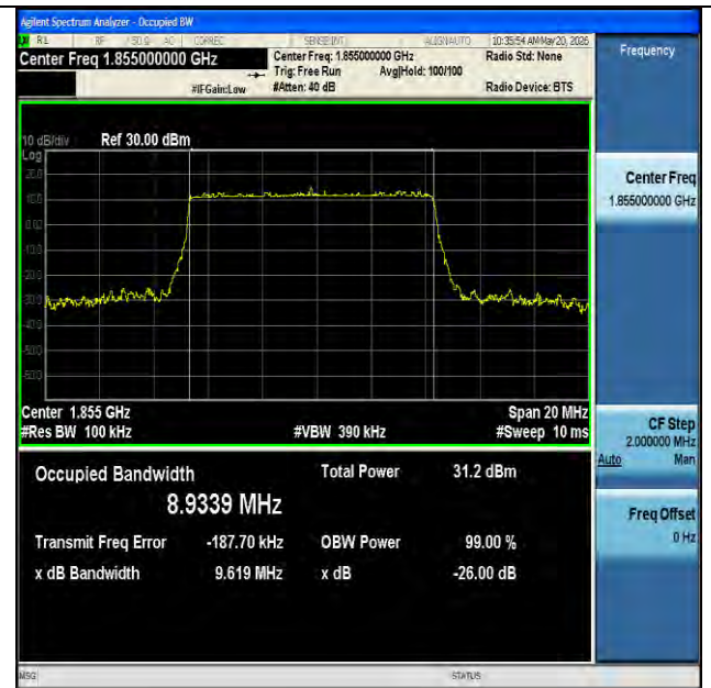
NTNV-n2-PC3-15-10-L-DFT-16QAM-Outer_Full-Ant1-PASS
