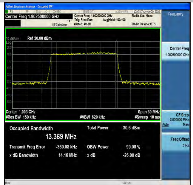
NTNV-n2-PC3-15-15-H-DFT-64QAM-Outer_Full-Ant1-PASS
