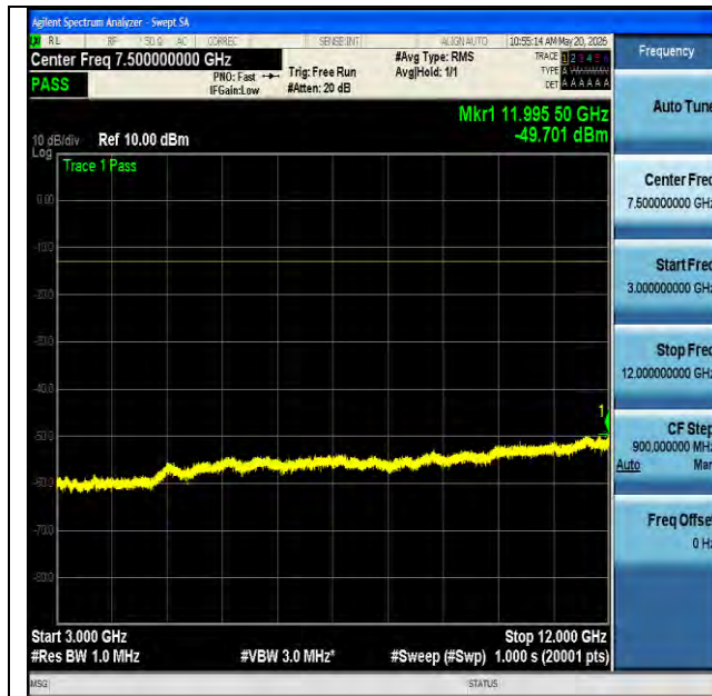
NTVN-n2-PC3-15-20-L-DFT-BPSK-Edge_1RB_Left-3000-12000- PASS
