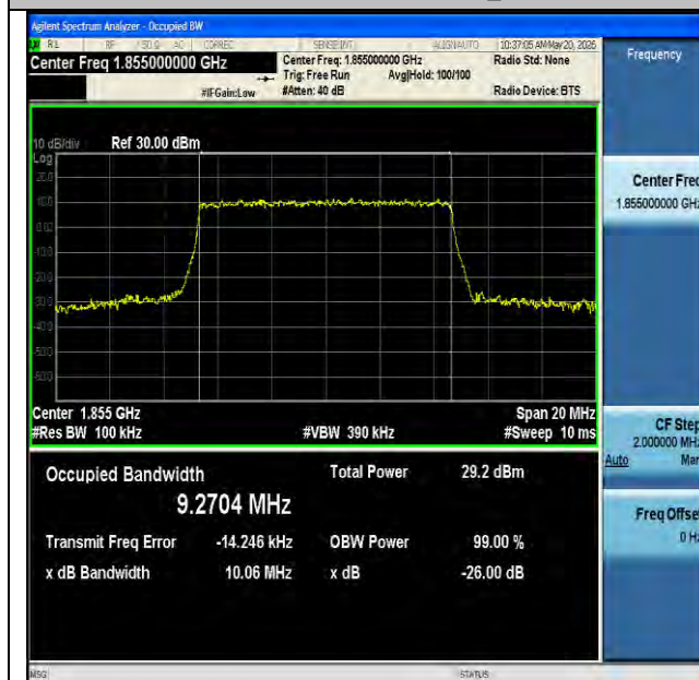
NTNV-n2-PC3-15-10-L-CP-64QAM-Outet_Full-Ant1-PASS
