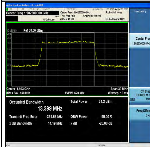
NTNV-n2-PC3-15-15-H-DFT-16QAM-Outer_Full-Ant1-PASS
