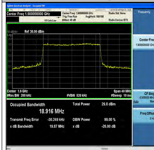
NTVN-n2-PC3-15-20-H-CP-64QAM-Outer_Full-Ant1-PASS
