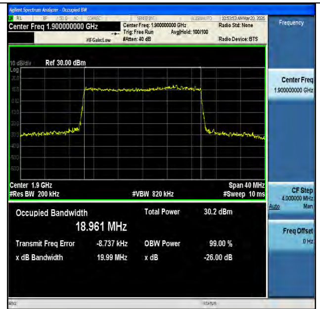
NTVN-n2-PC3-15-20-H-CP-16QAM-Outer_Full-Ant1-PASS
