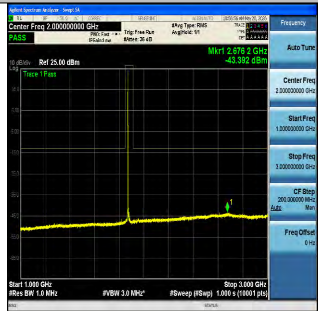
NTNV-n2-PC3-15-20-M-DFT-BPSK-Edge_1RB_Left-1000-3000- PASS
