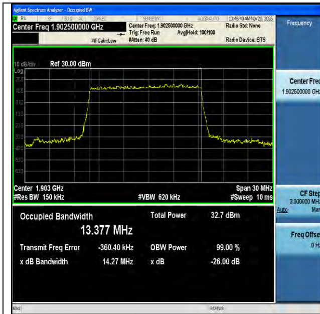
NTNV-n2-PC3-15-15-H-DFT-BPSK-Outer_Full-Ant1-PASS
