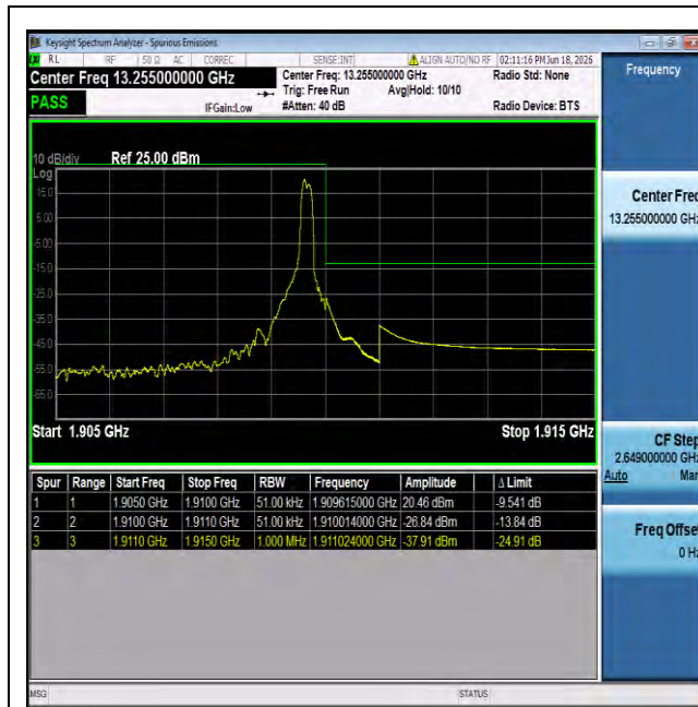
NTNV-n2-PC3-15-5-H-DFT-BPSK-Edge_1RB_Right-PASS
