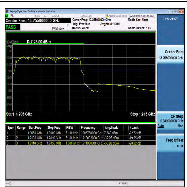
NTNV-n2-PC3-15-5-H-DFT-BPSK-Outer_Full-PASS
