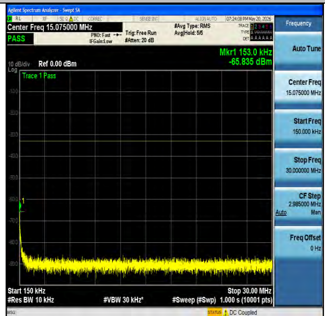
NTNV-n25-PC3-15-20-M-CP-QPSK-Edge_1RB_Left-0.15-30-PASS
