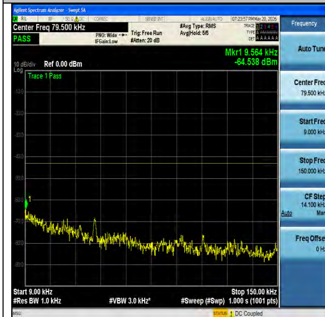
NTNV-n25-PC3-15-20-M-CP-QPSK-Edge_1RB_Left-0.009-0.15-PASS
