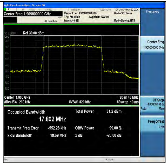
NTNV-n25-PC3-15-20-H-DFT-16QAM-Outet_Full-Ant1-PASS
