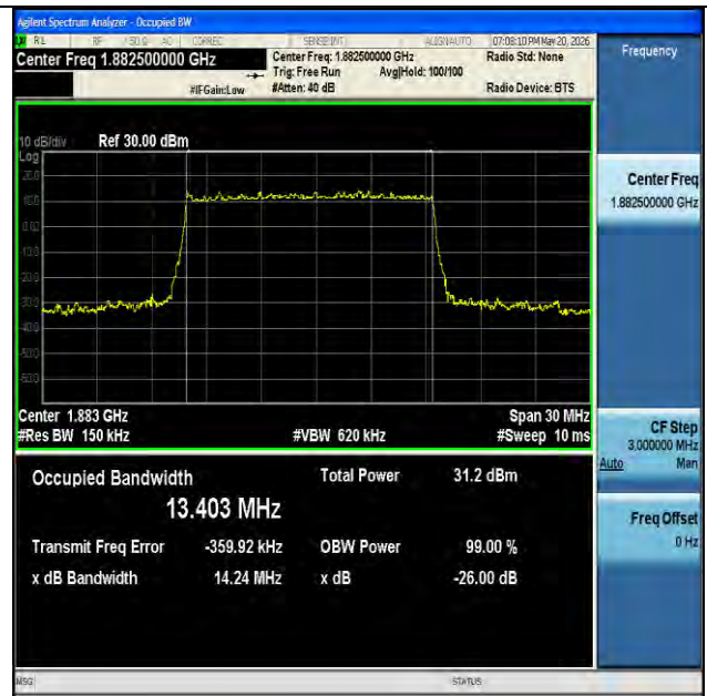
NTNV-n25-PC3-15-15-M-DFT-16QAM-Outer_Full-Ant1-PASS
