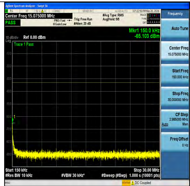
NTNV-n25-PC3-15-20-M-DFT-BPSK-Edge_1RB_Left-0.15-30- PASS
