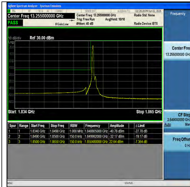
NTNV-n25-PC3-15-15-L-DFT-BPSK-Edge_1RB_Left-PASS
