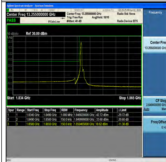
NTNV-n25-PC3-15-15-L-CP-QPSK-Edge_1RB_Left-PASS
