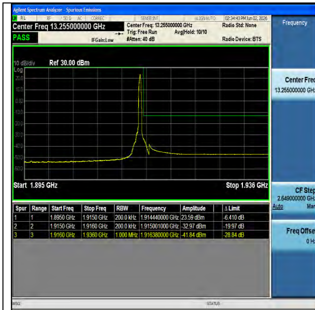
NTNV-n25-PC3-15-20-H-DFT-BPSK-Edge_1RB_Right-PASS
