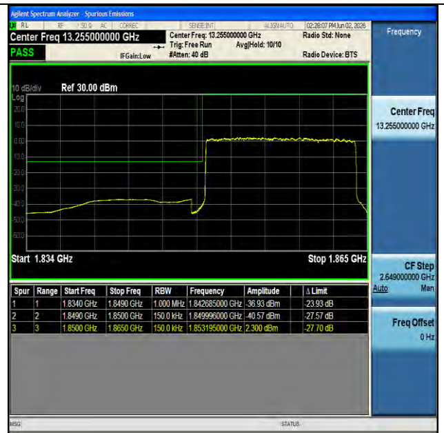
NTNV-n25-PC3-15-15-L-DFT-BPSK-Outer_Full-PASS
