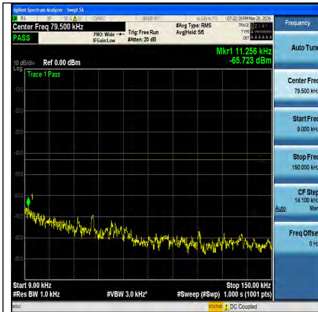
NTNV-n25-PC3-15-20-M-DFT-BPSK-Edge_1RB_Left-0.009-0.15- PASS
