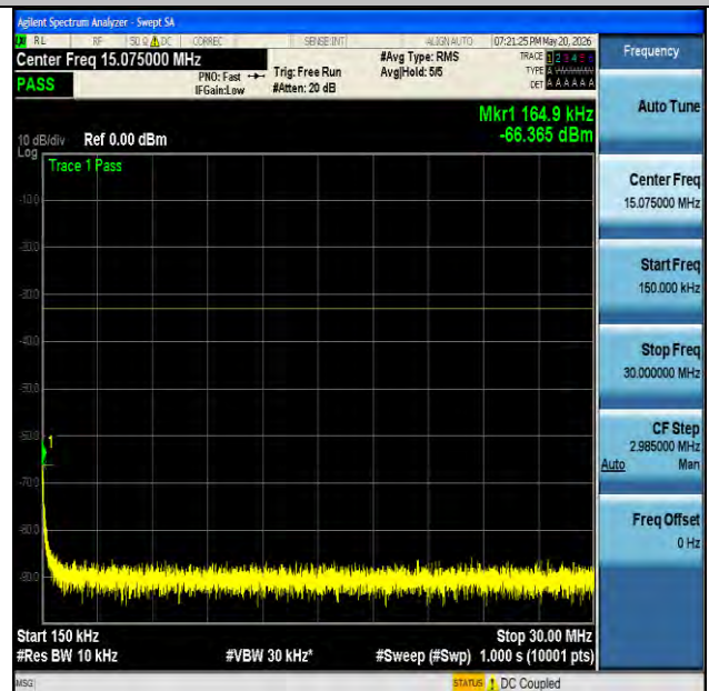
NTNV-n25-PC3-15-20-L-CP-QPSK-Edge_1RB_Left-0.15-30- PASS
