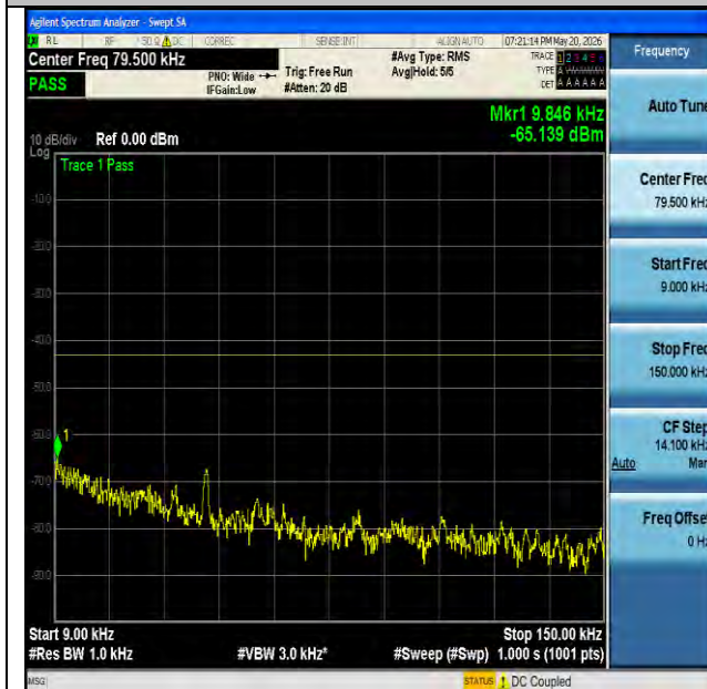
NTNV-n25-PC3-15-20-L-CP-QPSK-Edge_1RB_Left-0.009-0.15- PASS
