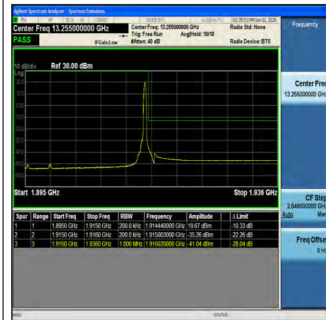
NTNV-n25-PC3-15-20-H-CP-QPSK-Edge_1RB_Right-PASS
