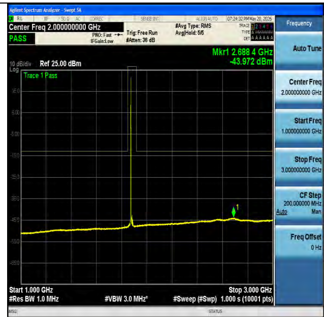
NTNV-n25-PC3-15-20-M-CP-QPSK-Edge_1RB_Left-1000-3000- PASS
