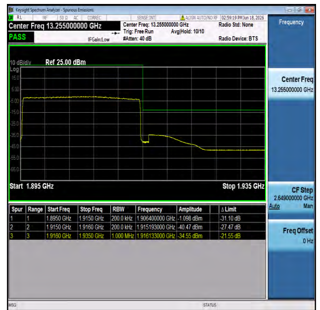
NTNV-n25-PC3-15-20-H-CP-QPSK-Outer_Full-PASS
