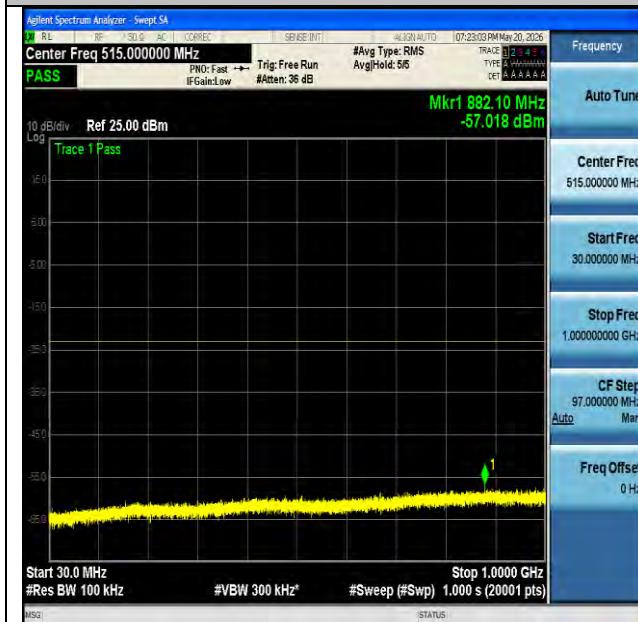
NTNV-n25-PC3-15-20-M-DFT-BPSK-Edge_1RB_Left-30-1000- PASS
