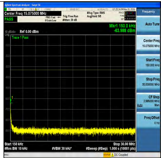
NTNV-n25-PC3-15-20-H-DFT-BPSK-Edge_1RB_Left-0.15-30- PASS
