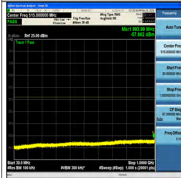
NTNV-n25-PC3-15-20-H-DFT-BPSK-Edge_1RB_Left-30-1000- PASS
