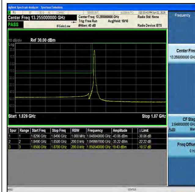
NTNV-n25-PC3-15-20-L-CP-QPSK-Edge_1RB_Left-PASS
