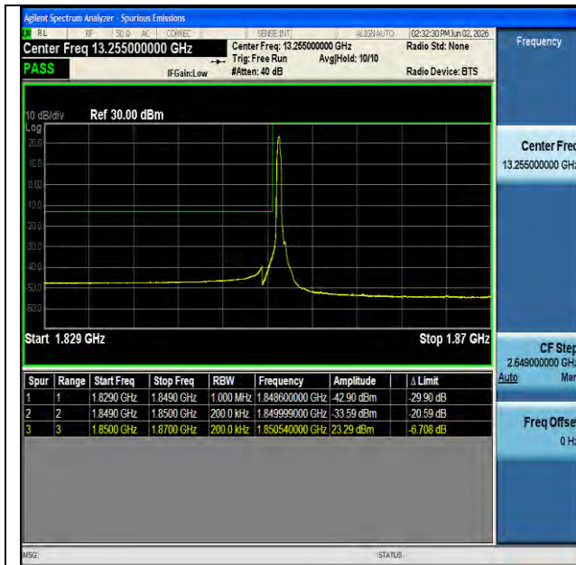
NTNV-n25-PC3-15-20-L-DFT-BPSK-Edge_1RB_Left-PASS
