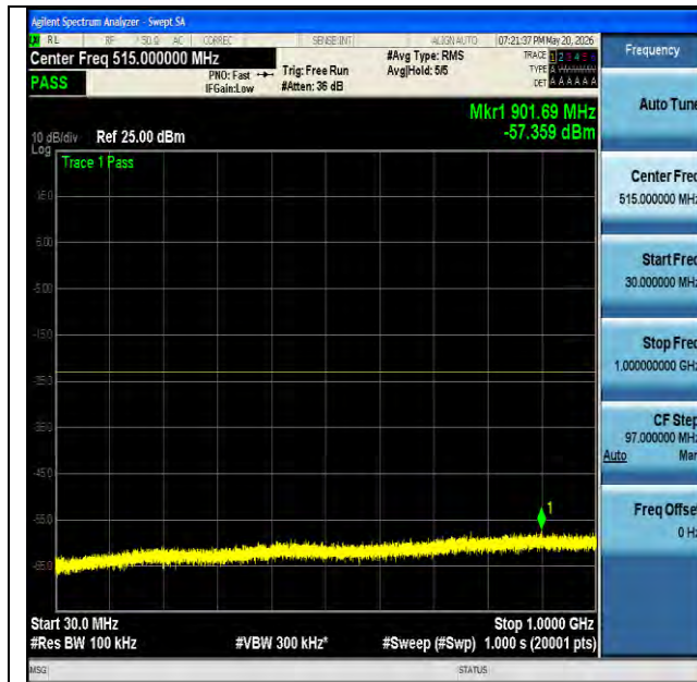
NTNV-n25-PC3-15-20-L-CP-QPSK-Edge_1RB_Left-30-1000- PASS
