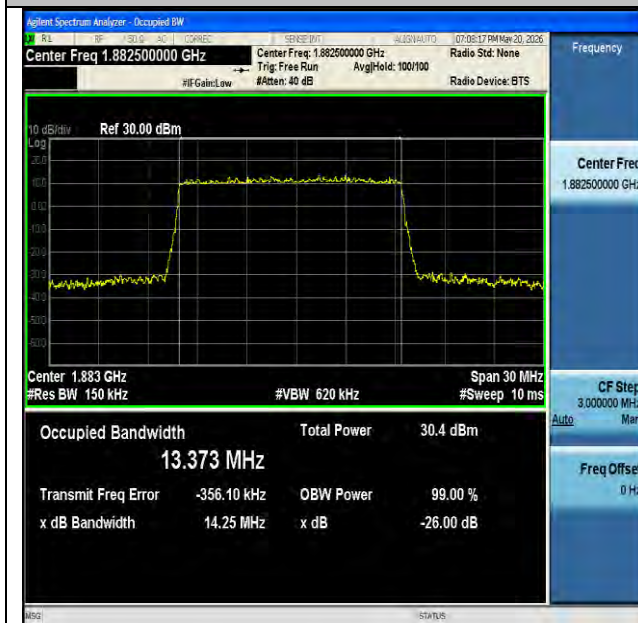
NTNV-n25-PC3-15-15-M-DFT-64QAM-Outer_Full-Ant1-PASS
