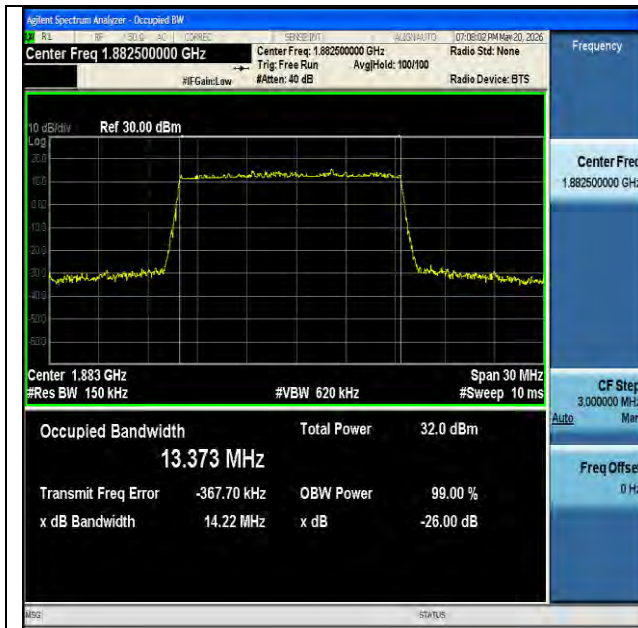
NTNV-n25-PC3-15-15-M-DFT-QPSK-Outer_Full-Ant1-PASS
