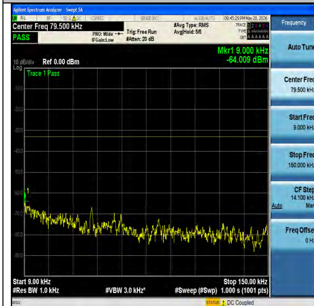
NTNV-n26(824-849)-PC3-15-20-L-CP-QPSK-Edge_1RB_Left- 0.009-0.15-PASS
