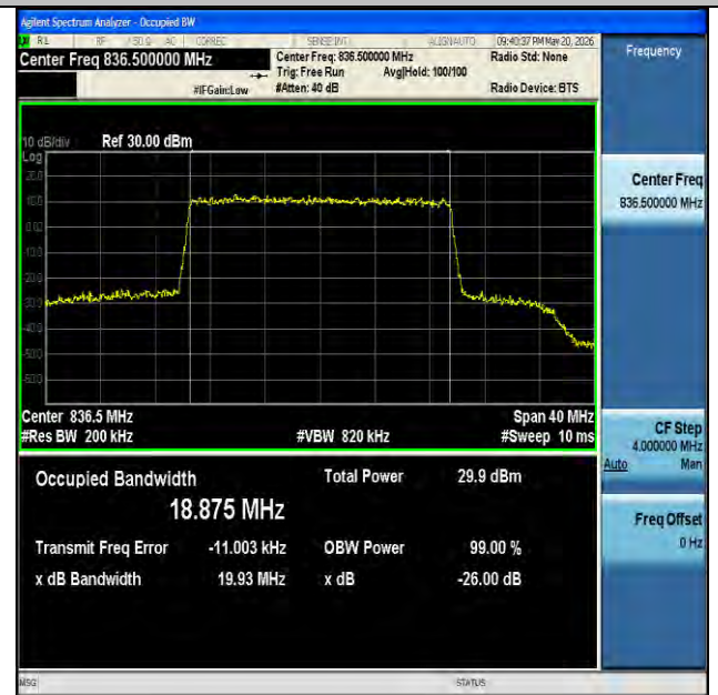
NTNV-n26(824-849)-PC3-15-20-M-CP-QPSK-Outer_Full-Ant1- PASS
