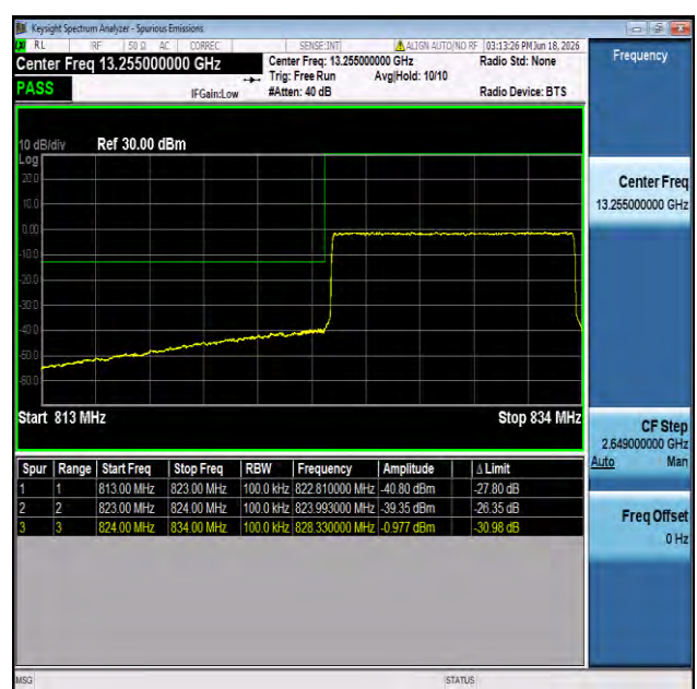
NTNV-n26(824-849)-PC3-15-10-L-CP-QPSK-Outer_Full-PASS
