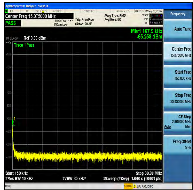
NTNV-n26(824-849)-PC3-15-20-H-DFT-BPSK-Edge_1RB_Left- 0.15-30-PASS
