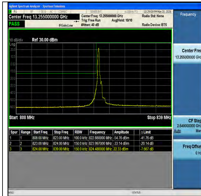
NTVN-n26(824-849)-PC3-15-15-L-DFT-BPSK-Edge_1RB_Left-PASS
