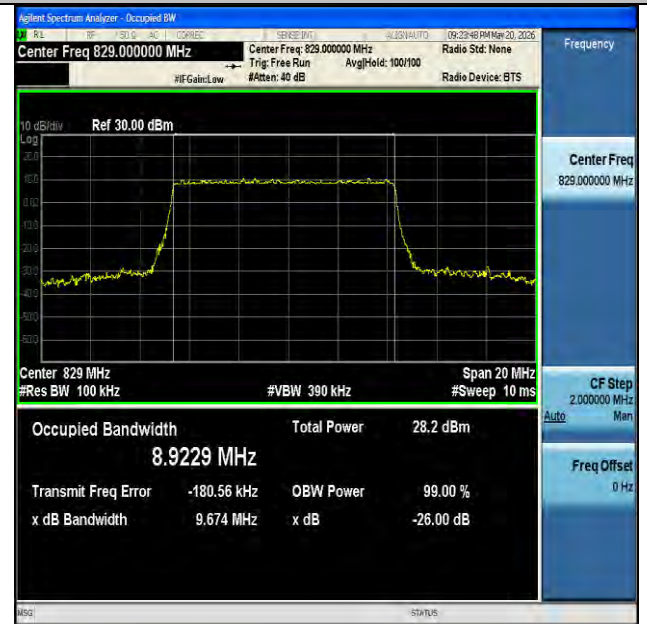
NTNV-n26(824-849)-PC3-15-10-L-DFT-256QAM-Outer_Full-Ant1- PASS
