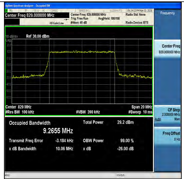
NTNV-n26(824-849)-PC3-15-10-L-CP-16QAM-Outer_Full-Ant1- PASS
