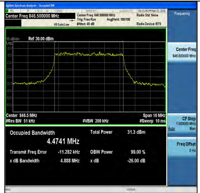
NTNV-n26(824-849)-PC3-15-5-H-DFT-QPSK-Outer_Full-Ant1- PASS
