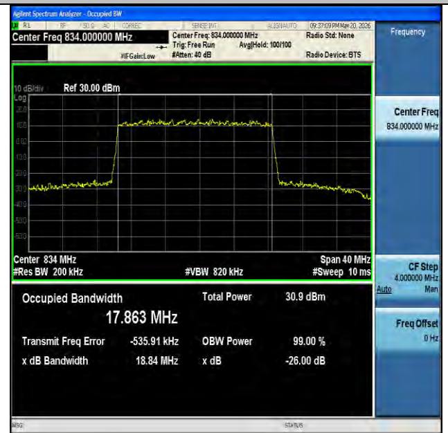
NTNV-n26(824-849)-PC3-15-20-L-DFT-16QAM-Outer_Full-Ant1- PASS
