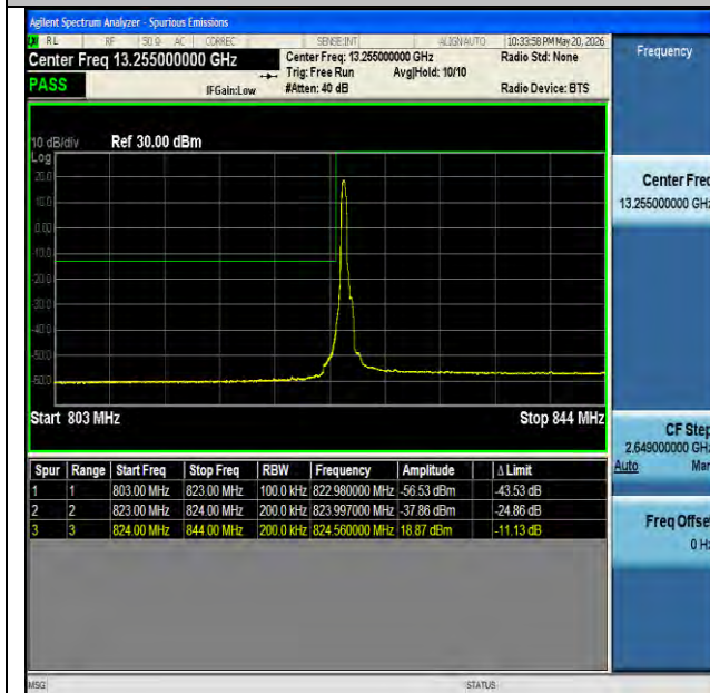
NTNV-n26(824-849)-PC3-15-20-L-CP-QPSK-Edge_1RB_Left-PASS
