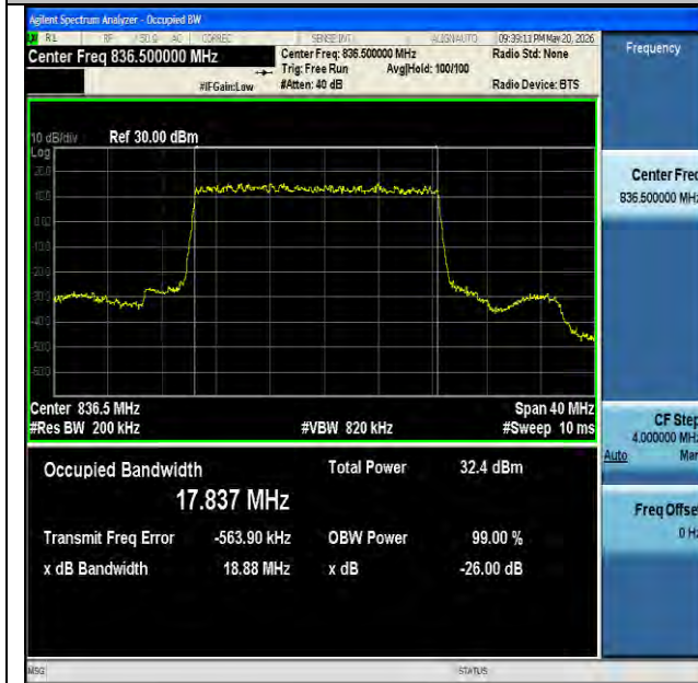
NTNV-n26(824-849)-PC3-15-20-M-DFT-BPSK-Outer_Full-Ant1- PASS
