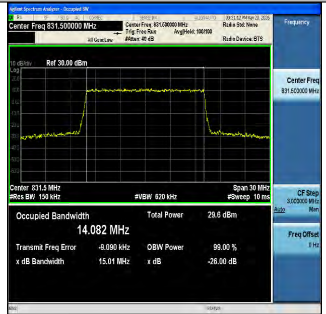
NTNV-n26(824-849)-PC3-15-15-L-CP-QPSK-Outer_Full-Ant1- PASS
