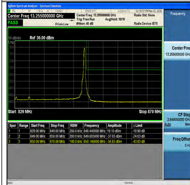
NTNV-n26(824-849)-PC3-15-20-H-CP-QPSK-Edge_1RB_Right-PASS
