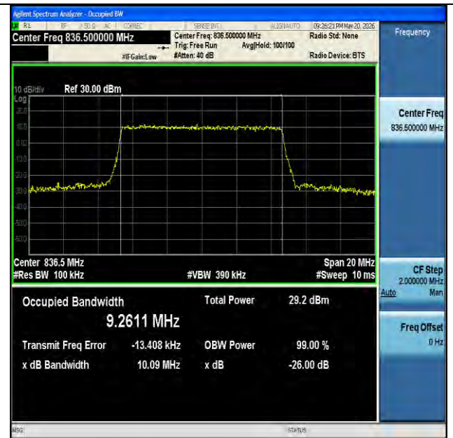
NTVN-n26(824-849)-PC3-15-10-M-CP-QPSK-Outer_Full-Ant1-PASS
