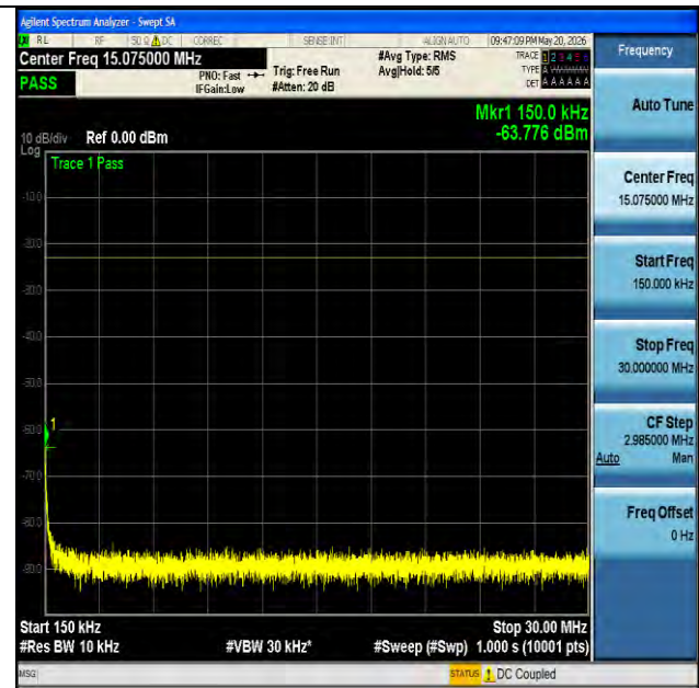
NTNV-n26(824-849)-PC3-15-20-M-DFT-BPSK-Edge_1RB_Left- 0.15-30-PASS
