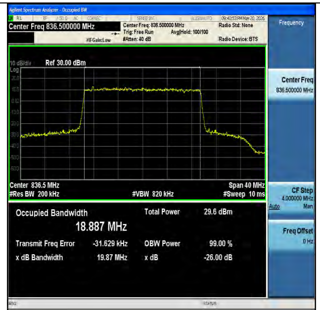
NTNV-n26(824-849)-PC3-15-20-M-CP-64QAM-Outer_Full-Ant1- PASS
