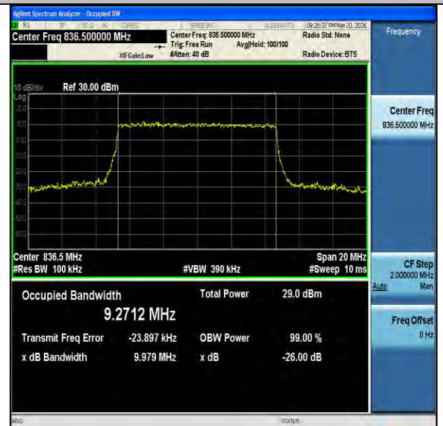
NTVN-n26(824-849)-PC3-15-10-M-CP-64QAM-Outer_Full-Ant1-PASS
