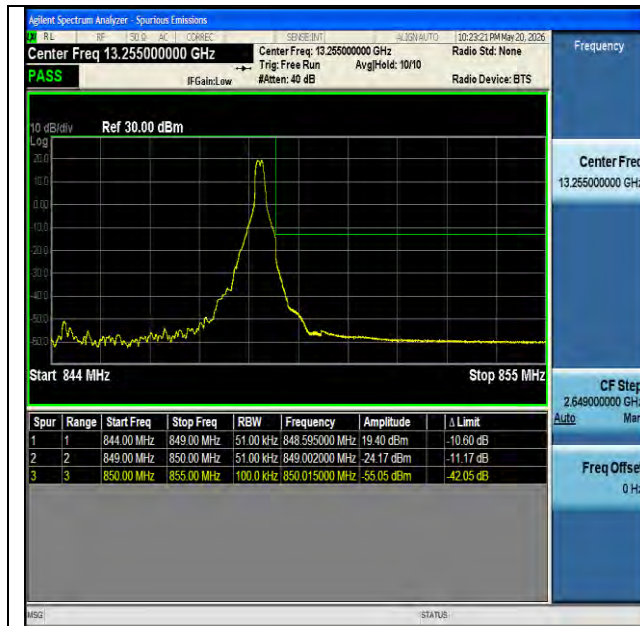
NTVN-n26(824-849)-PC3-15-5-H-DFT-BPSK-Edge_1RB_Right-PASS
