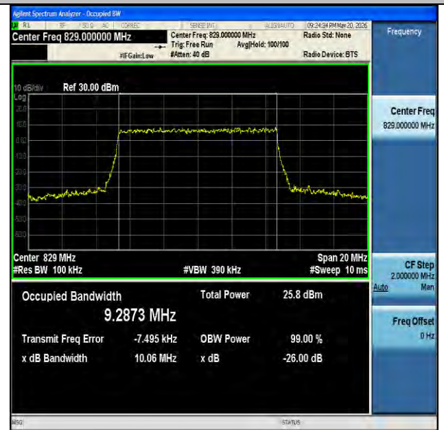
NTNV-n26(824-849)-PC3-15-10-L-CP-256QAM-Outer_Full-Ant1- PASS
