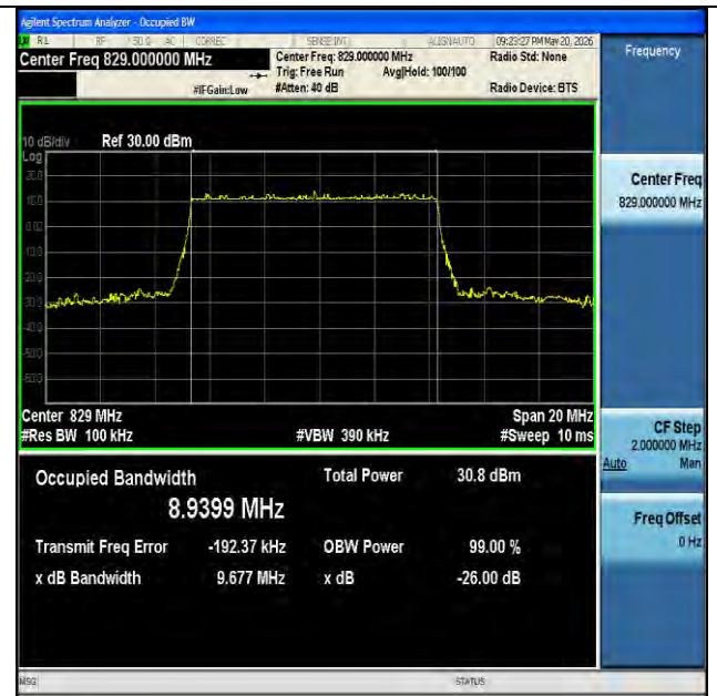
NTNV-n26(824-849)-PC3-15-10-L-DFT-16QAM-Outer_Full-Ant1- PASS
