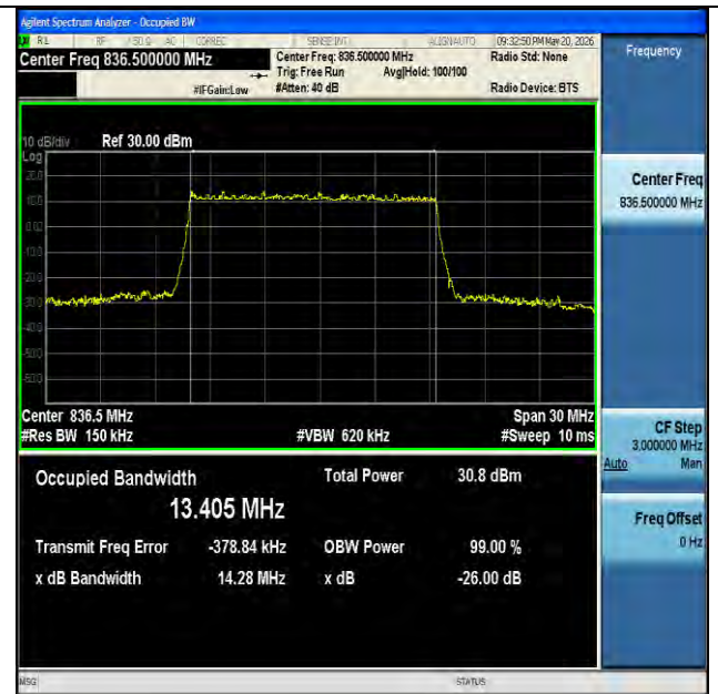
NTNV-n26(824-849)-PC3-15-15-M-DFT-16QAM-Outer_Full-Ant1- PASS
