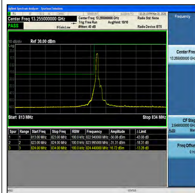
NTNV-n26(824-849)-PC3-15-10-L-CP-QPSK-Edge_1RB_Left-PASS
