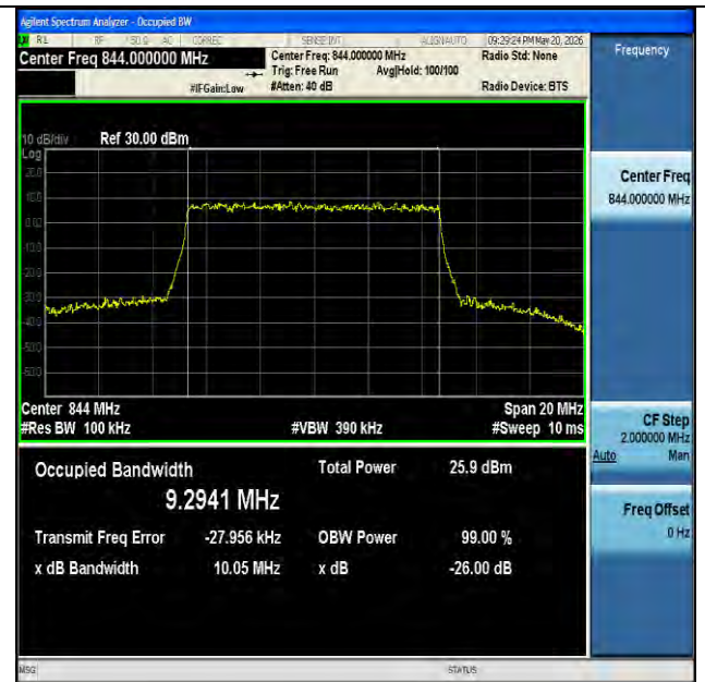
NTNV-n26(824-849)-PC3-15-10-H-CP-256QAM-Outer_Full-Ant1- PASS
