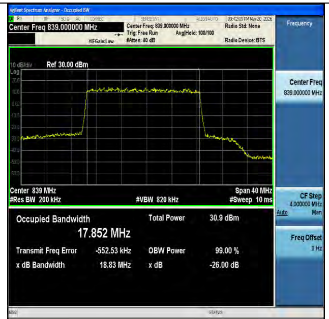
NTNV-n26(824-849)-PC3-15-20-H-DFT-16QAM-Outer_Full-Ant1- PASS
