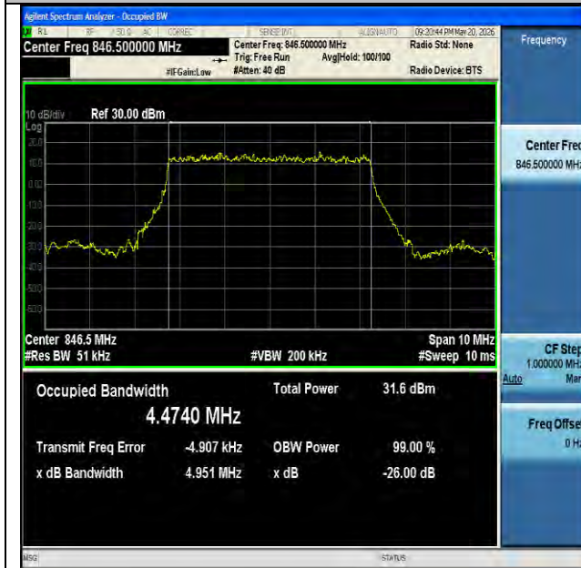
NTNV-n26(824-849)-PC3-15-5-H-DFT-BPSK-Outer_Full-Ant1- PASS
