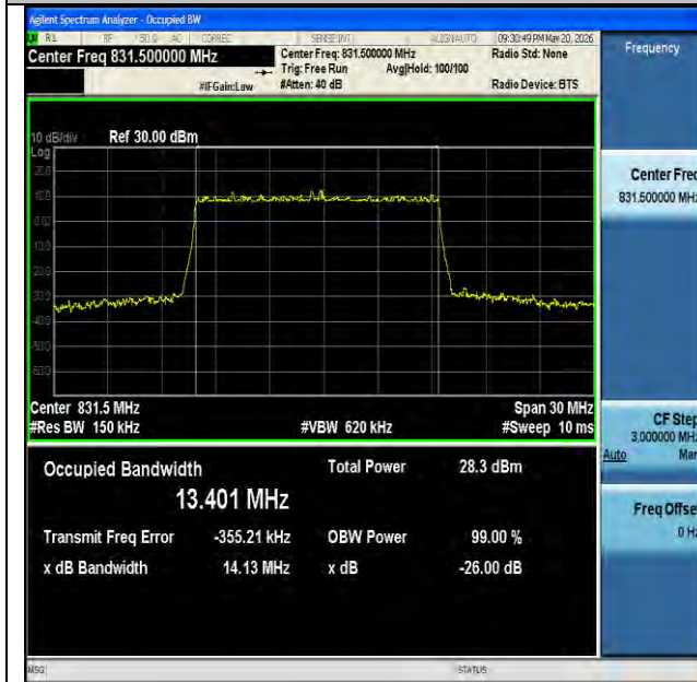
NTNV-n26(824-849)-PC3-15-15-L-DFT-256QAM-Outer_Full-Ant1- PASS
