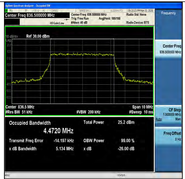
NTNV-n26(824-849)-PC3-15-5-M-CP-256QAM-Outer_Full-Ant1- PASS
