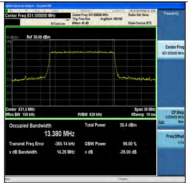
NTNV-n26(824-849)-PC3-15-15-L-DFT-64QAM-Outer_Full-Ant1- PASS
