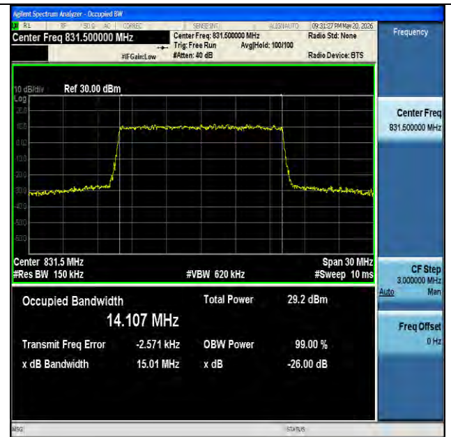
NTVN-n26(824-849)-PC3-15-15-L-CP-64QAM-Outer_Full-Ant1- PASS
