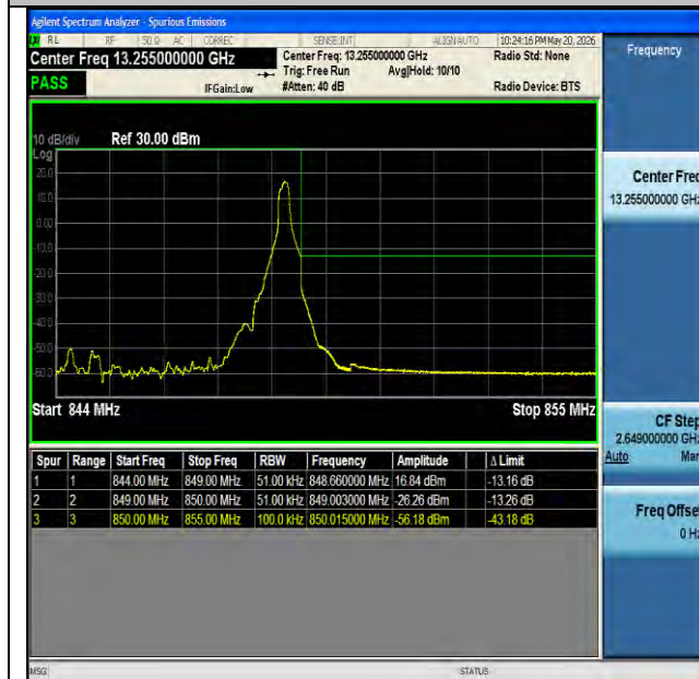
NTVN-n26(824-849)-PC3-15-5-H-CP-QPSK-Edge_1RB_Right-PASS
