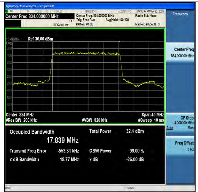
NTNV-n26(824-849)-PC3-15-20-L-DFT-BPSK-Outer_Full-Ant1- PASS
