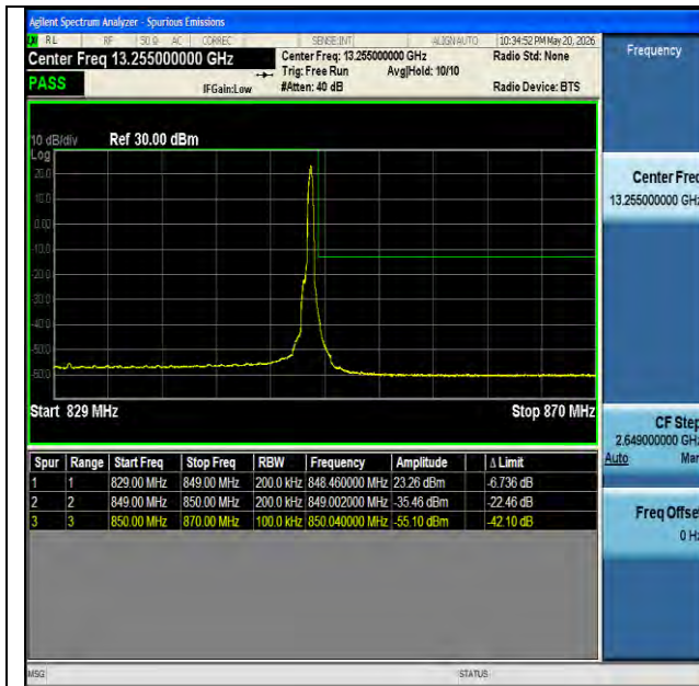
NTNV-n26(824-849)-PC3-15-20-H-DFT-BPSK-Edge_1RB_Right-PASS
