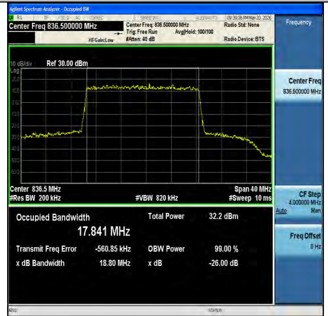
NTNV-n26(824-849)-PC3-15-20-M-DFT-QPSK-Outer_Full-Ant1- PASS
