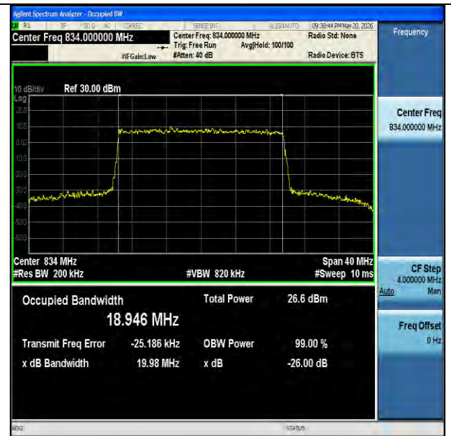
NTNV-n26(824-849)-PC3-15-20-L-CP-256QAM-Outer_Full-Ant1- PASS
