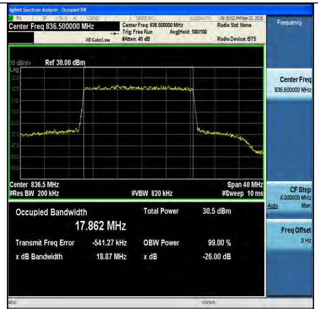
NTNV-n26(824-849)-PC3-15-20-M-DFT-64QAM-Outer_Full-Ant1- PASS
