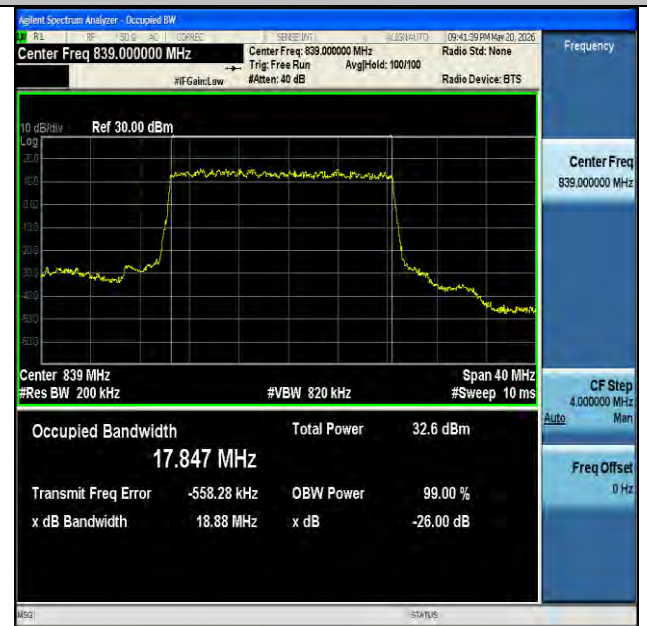
NTNV-n26(824-849)-PC3-15-20-H-DFT-BPSK-Outer_Full-Ant1- PASS
