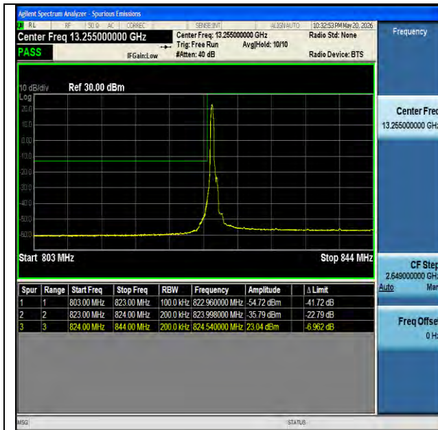
NTNV-n26(824-849)-PC3-15-20-L-DFT-BPSK-Edge_1RB_Left-PASS
