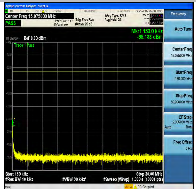
NTNV-n26(824-849)-PC3-15-20-L-CP-QPSK-Edge_1RB_Left- 0.15-30-PASS
