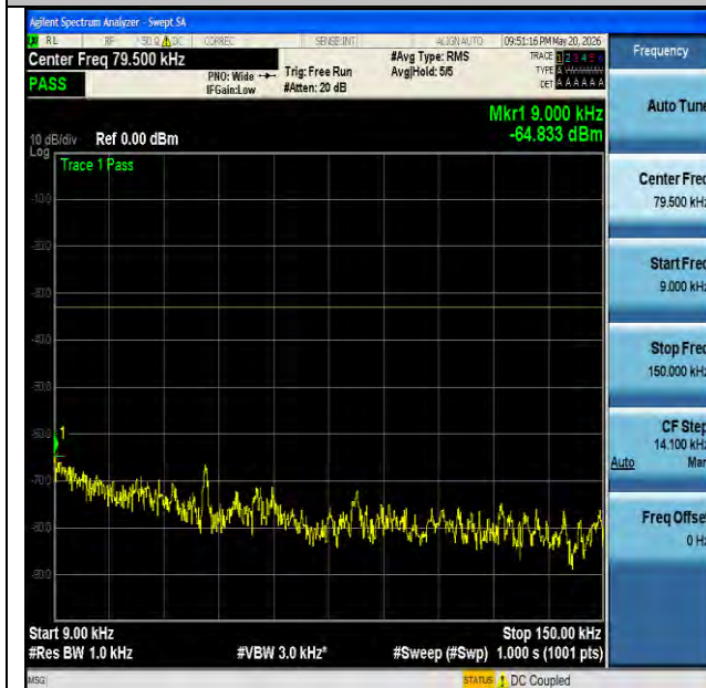
NTNV-n26(824-849)-PC3-15-20-H-CP-QPSK-Edge_1RB_Left- 0.009-0.15-PASS
