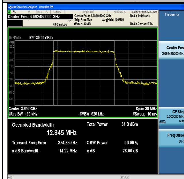
NTNV-n48-PC3-30-15-H-DFT-QPSK-Outer_Full-Ant1-PASS
