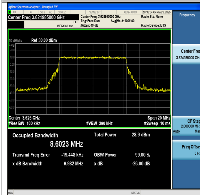
NTNV-n48-PC3-30-10-M-CP-QPSK-Outer_Full-Ant1-PASS
