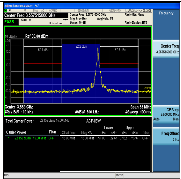
NTNV-n48-PC3-30-15-L-CP-QPSK-Edge_1RB_Right-PASS
