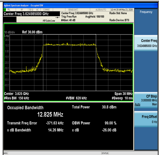
NTNV-n48-PC3-30-15-M-DFT-64QAM-Outer_Full-Ant1-PASS
