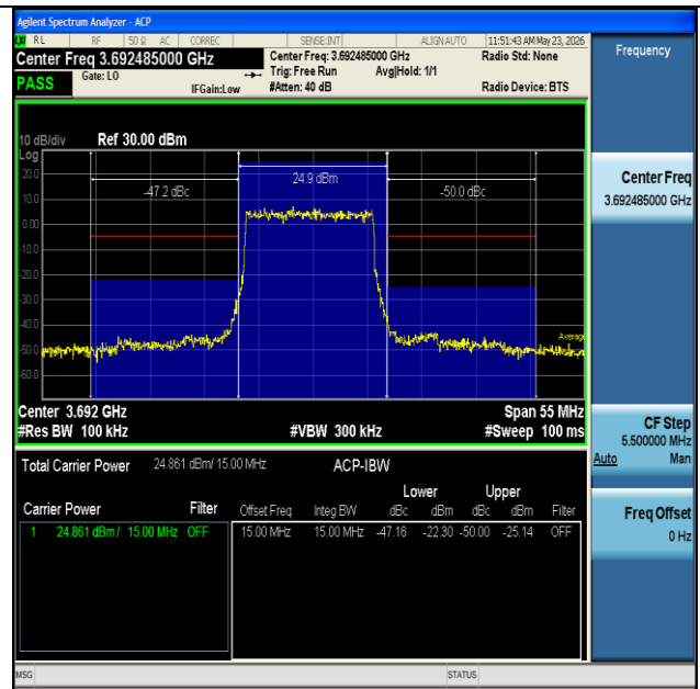
NTNV-n48-PC3-30-15-H-DFT-BPSK-Outer_Full-PASS
