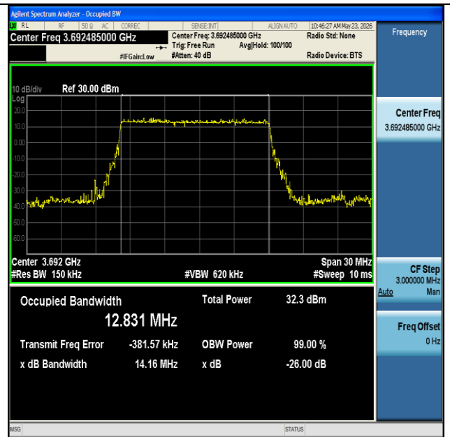
NTNV-n48-PC3-30-15-H-DFT-BPSK-Outer_Full-Ant1-PASS
