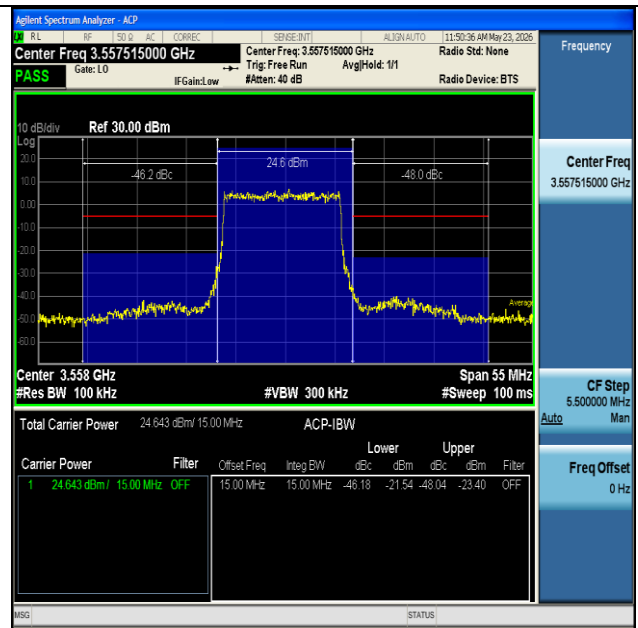
NTNV-n48-PC3-30-15-L-DFT-BPSK-Outer_Full-PASS
