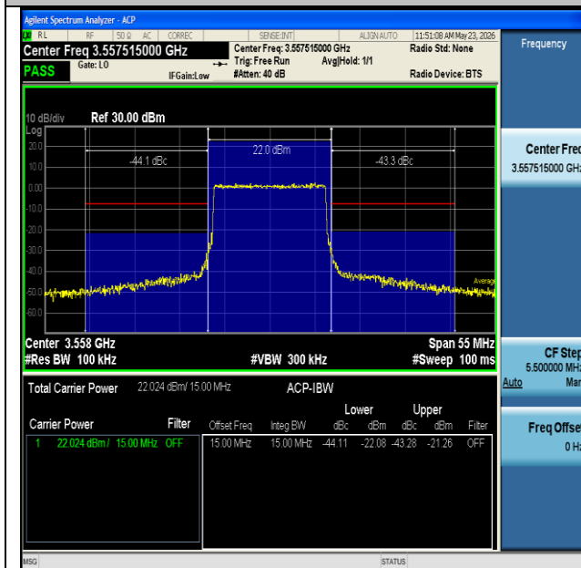
NTNV-n48-PC3-30-15-L-CP-QPSK-Outer_Full-PASS
