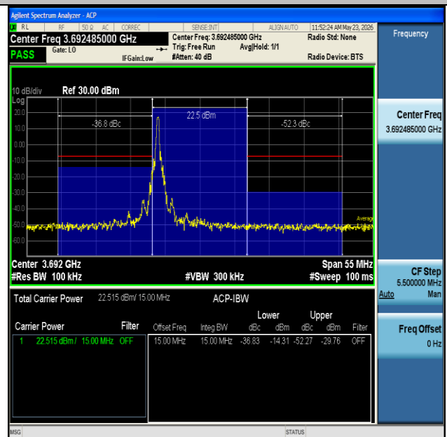
NTNV-n48-PC3-30-15-H-CP-QPSK-Edge_1RB_Left-PASS
