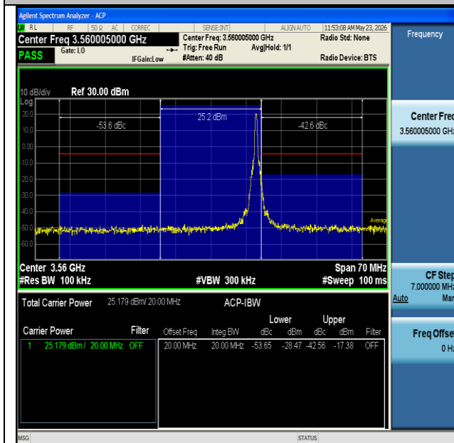
NTNV-n48-PC3-30-20-L-DFT-BPSK-Edge_1RB_Right-PASS
