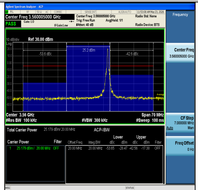
NTNV-n48-PC3-30-20-L-DFT-BPSK-Edge_1RB_Right-PASS
