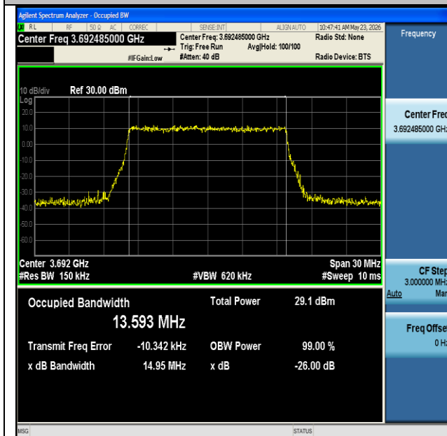
NTNV-n48-PC3-30-15-H-CP-QPSK-Outer_Full-Ant1-PASS
