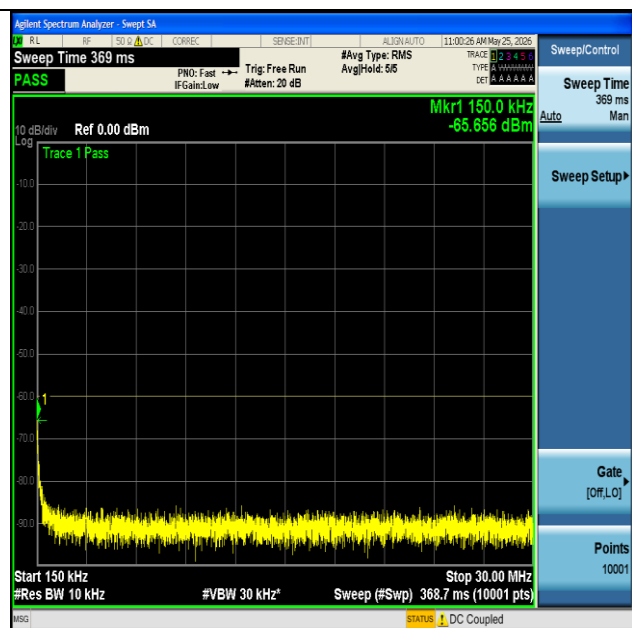
NTNV-n48-PC3-30-20-H-DFT-BPSK-Edge_1RB_Left-0.15-30- PASS
