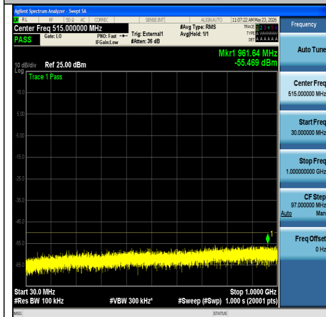
NTNV-n48-PC3-30-20-H-CP-QPSK-Edge_1RB_Left-30-1000- PASS
