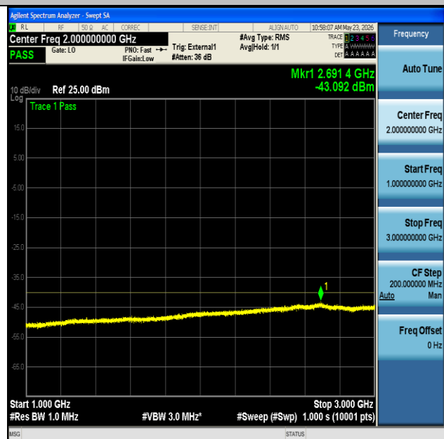
NTNV-n48-PC3-30-20-L-CP-QPSK-Edge_1RB_Left-1000-3000- PASS
