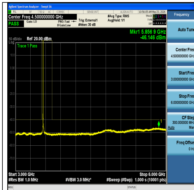
NTNV-n48-PC3-30-20-L-DFT-BPSK-Edge_1RB_Left-3000-6000- PASS
