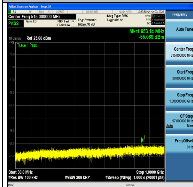
NTNV-n48-PC3-30-20-L-CP-QPSK-Edge_1RB_Left-30-1000- PASS
