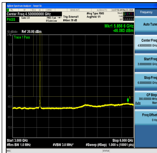
NTNV-n48-PC3-30-20-H-CP-QPSK-Edge_1RB_Left-3000-6000-PASS
