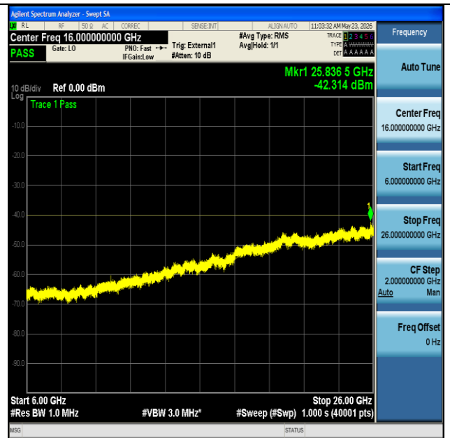
NTNV-n48-PC3-30-20-M-CP-QPSK-Edge_1RB_Left-6000-26000- PASS
