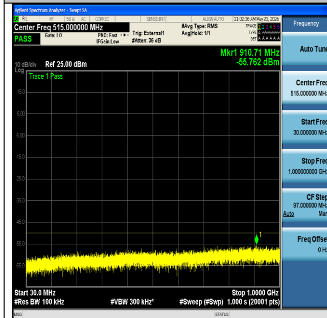
NTNV-n48-PC3-30-20-M-CP-QPSK-Edge_1RB_Left-30-1000- PASS
