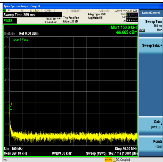
NTNV-n48-PC3-30-20-H-CP-QPSK-Edge_1RB_Left-0.15-30- PASS
