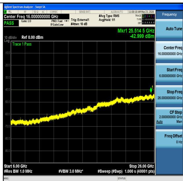
NTNV-n48-PC3-30-20-H-CP-QPSK-Edge_1RB_Left-6000-26000-PASS
