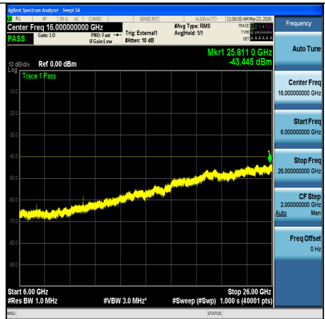
NTNV-n48-PC3-30-20-H-DFT-BPSK-Edge_1RB_Left-6000- 26000-PASS
