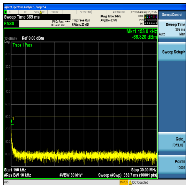
NTNV-n48-PC3-30-20-L-CP-QPSK-Edge_1RB_Left-0.15-30- PASS
