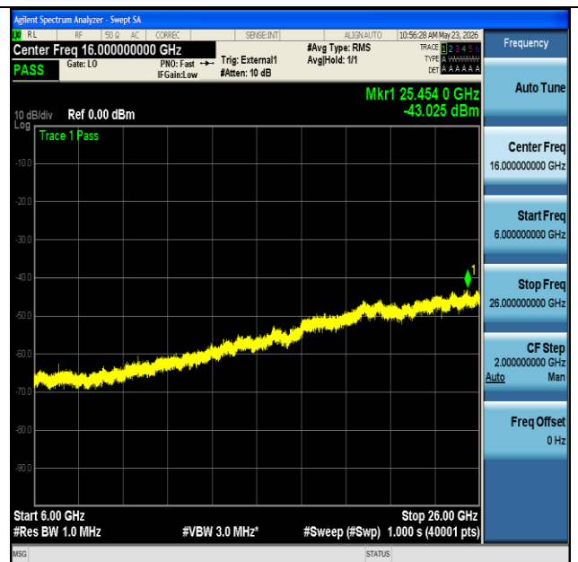
NTNV-n48-PC3-30-20-L-DFT-BPSK-Edge_1RB_Left-6000-26000- PASS
