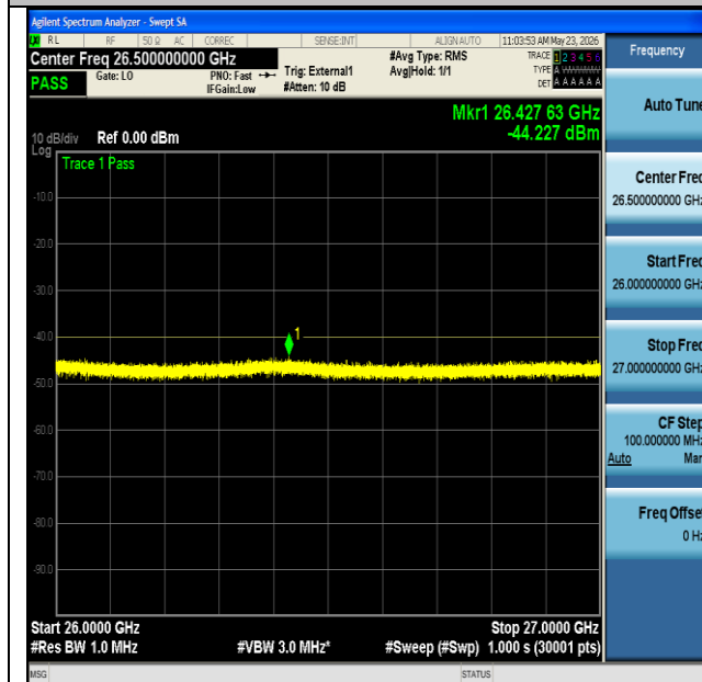
NTNV-n48-PC3-30-20-M-CP-QPSK-Edge_1RB_Left-26000- 27000-PASS
