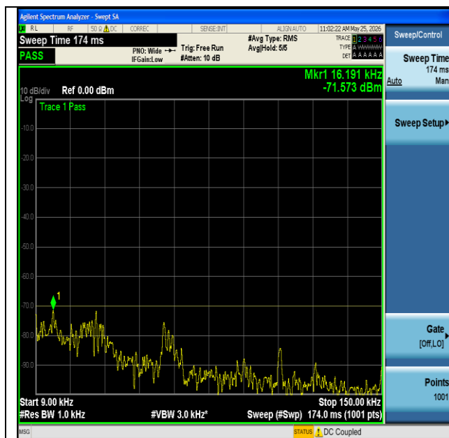
NTNV-n48-PC3-30-20-H-CP-QPSK-Edge_1RB_Left-0.009-0.15- PASS
