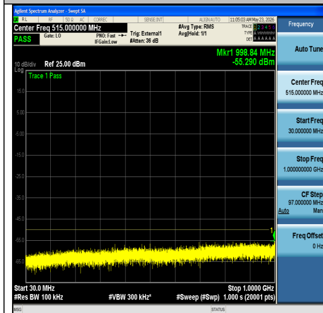
NTNV-n48-PC3-30-20-H-DFT-BPSK-Edge_1RB_Left-30-1000- PASS
