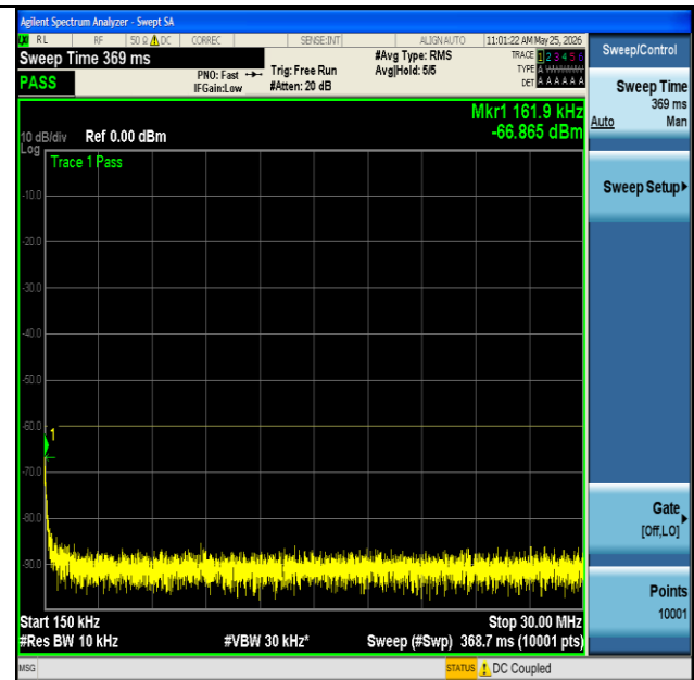
NTNV-n48-PC3-30-20-M-CP-QPSK-Edge_1RB_Left-0.15-30- PASS
