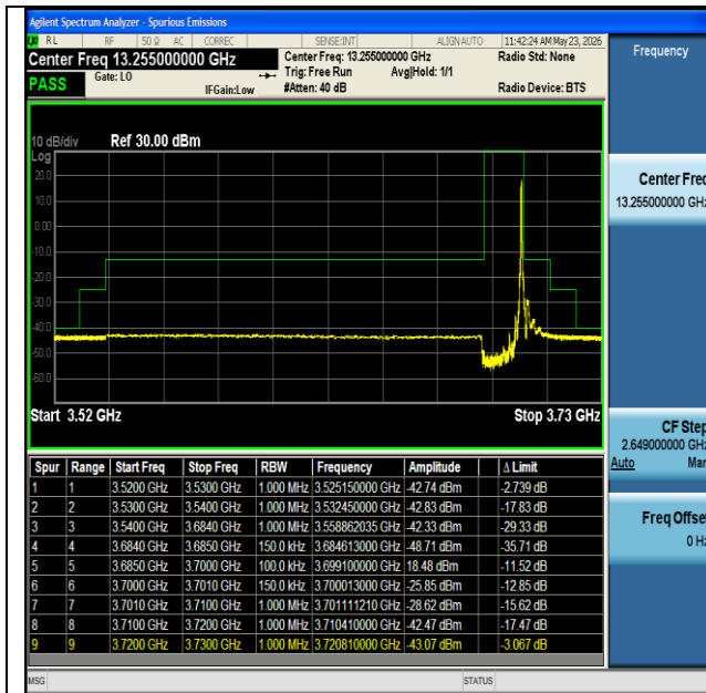
NTNV-n48-PC3-30-15-H-DFT-BPSK-Edge_1RB_Right-PASS
