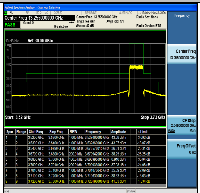
NTNV-n48-PC3-30-20-H-CP-QPSK-Outer_Full-PASS
