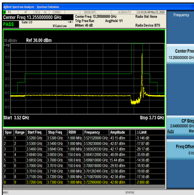
NTNV-n48-PC3-30-15-H-CP-QPSK-Edge_1RB_Right-PASS
