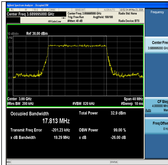
NTNV-n48-PC3-30-20-H-DFT-BPSK-Outer_Full-Ant1-PASS
