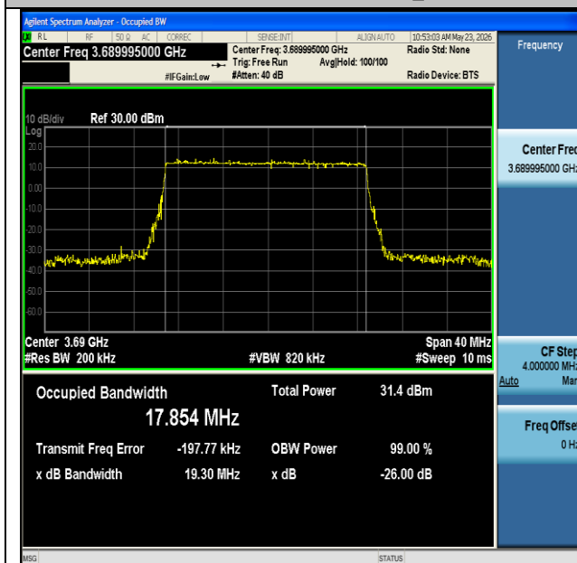
NTNV-n48-PC3-30-20-H-DFT-16QAM-Outer_Full-Ant1-PASS
