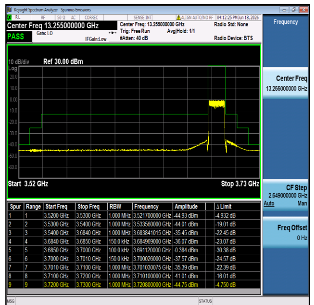
NTNV-n48-PC3-30-15-H-CP-QPSK-Outer_Full-PASS
