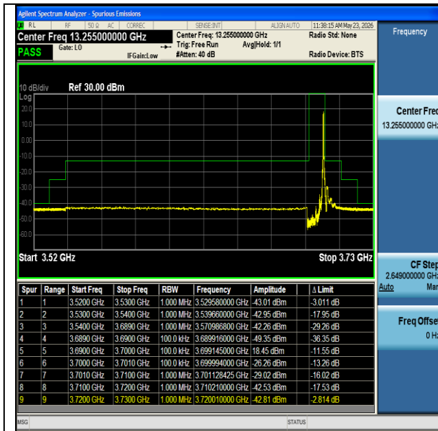
NTNV-n48-PC3-30-10-H-DFT-BPSK-Edge_1RB_Right-PASS
