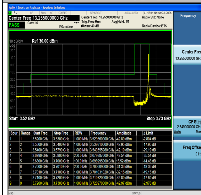
NTNV-n48-PC3-30-20-H-CP-QPSK-Edge_1RB_Right-PASS
