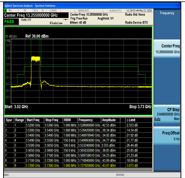
NTNV-n48-PC3-30-15-L-DFT-BPSK-Outer_Full-PASS
