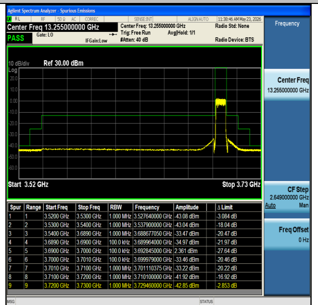
NTNV-n48-PC3-30-10-H-CP-QPSK-Outer_Full-PASS
