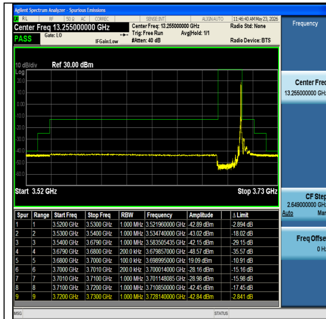
NTNV-n48-PC3-30-20-H-DFT-BPSK-Edge_1RB_Right-PASS
