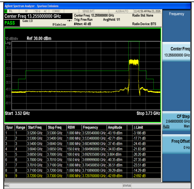
NTNV-n48-PC3-30-15-H-DFT-BPSK-Outer_Full-PASS
