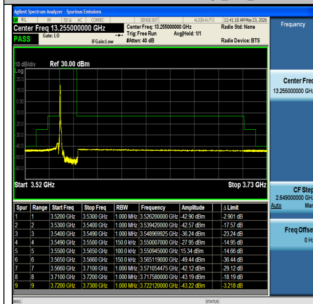
NTNV-n48-PC3-30-15-L-CP-QPSK-Edge_1RB_Left-PASS
