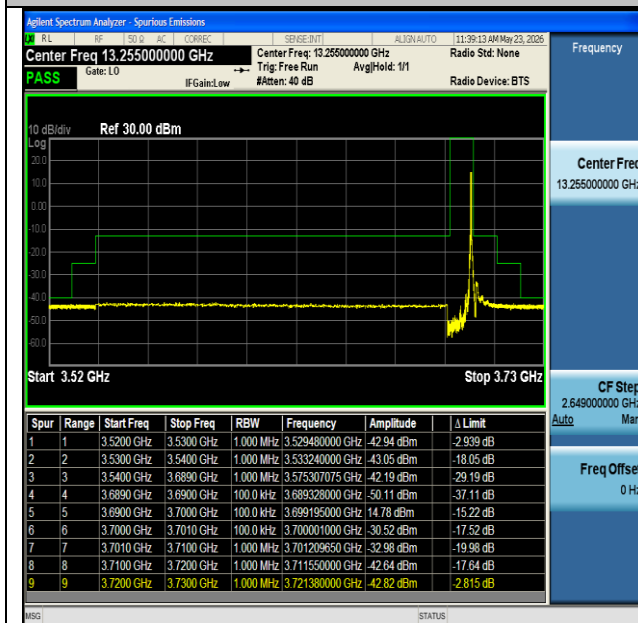
NTNV-n48-PC3-30-10-H-CP-QPSK-Edge_1RB_Right-PASS
