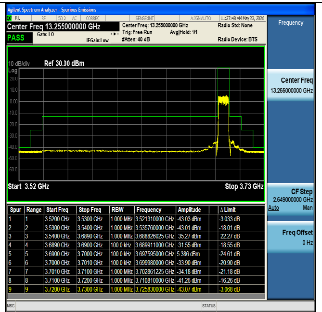
NTNV-n48-PC3-30-10-H-DFT-BPSK-Outer_Full-PASS
