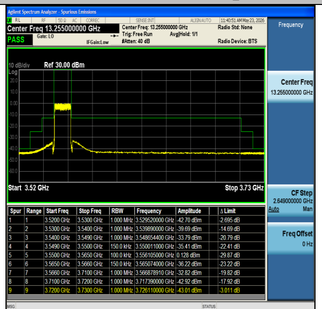
NTNV-n48-PC3-30-15-L-CP-QPSK-Outer_Full-PASS
