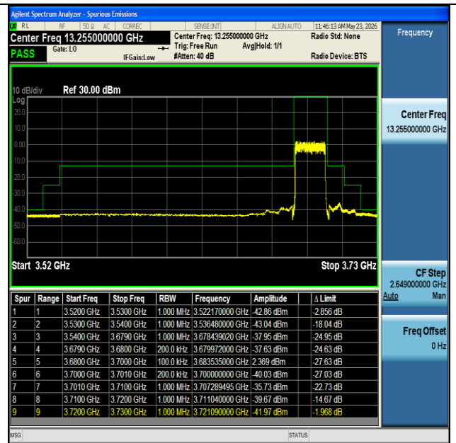
NTNV-n48-PC3-30-20-H-DFT-BPSK-Outer_Full-PASS
