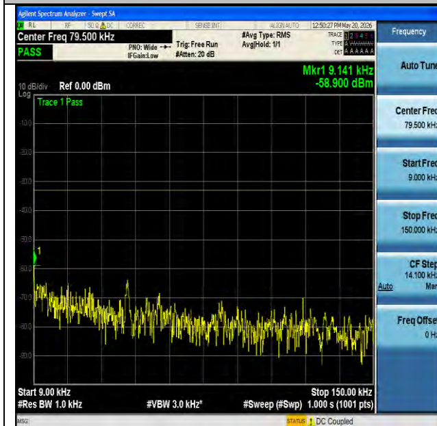
NTVN-n5-PC3-15-20-L-CP-QPSK-Edge_1RB_Left-0.009-0.15- PASS
