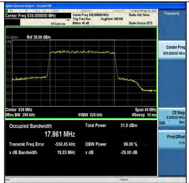
NTNV-n5-PC3-15-20-H-DFT-16QAM-Outer_Full-Ant1-PASS
