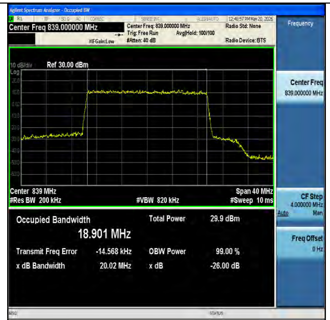
NTVN-n5-PC3-15-20-H-CP-16QAM-Outer_Full-Ant1-PASS
