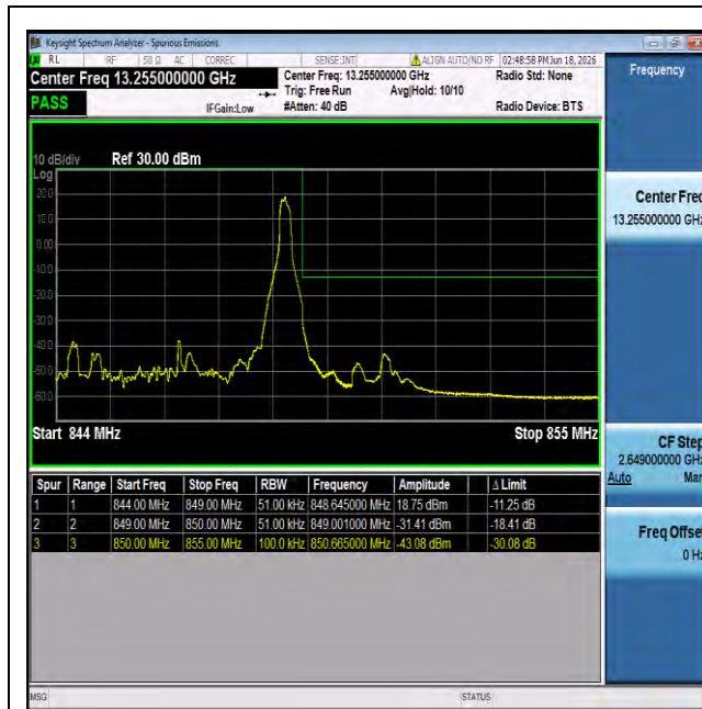
NTNV-n5-PC3-15-5-H-DFT-BPSK-Edge_1RB_Right-PASS
