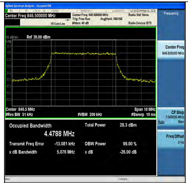
NTNV-n5-PC3-15-5-H-CP-64QAM-Outer_Full-Ant1-PASS
