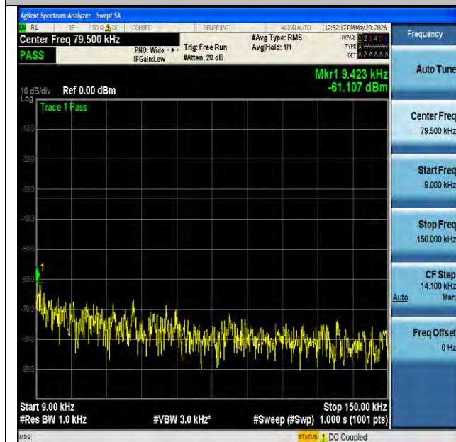
NTNV-n5-PC3-15-20-M-CP-QPSK-Edge_1RB_Left-0.009-0.15- PASS
