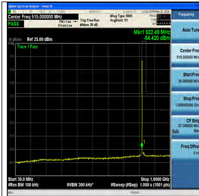
NTNV-n5-PC3-15-20-L-CP-QPSK-Edge_1RB_Left-30-1000-PASS
