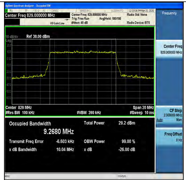
NTNV-n5-PC3-15-10-L-CP-16QAM-Outer_Full-Ant1-PASS
