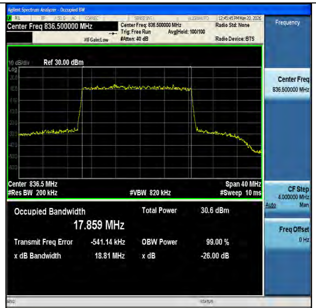
NTNV-n5-PC3-15-20-M-DFT-64QAM-Outer_Full-Ant1-PASS
