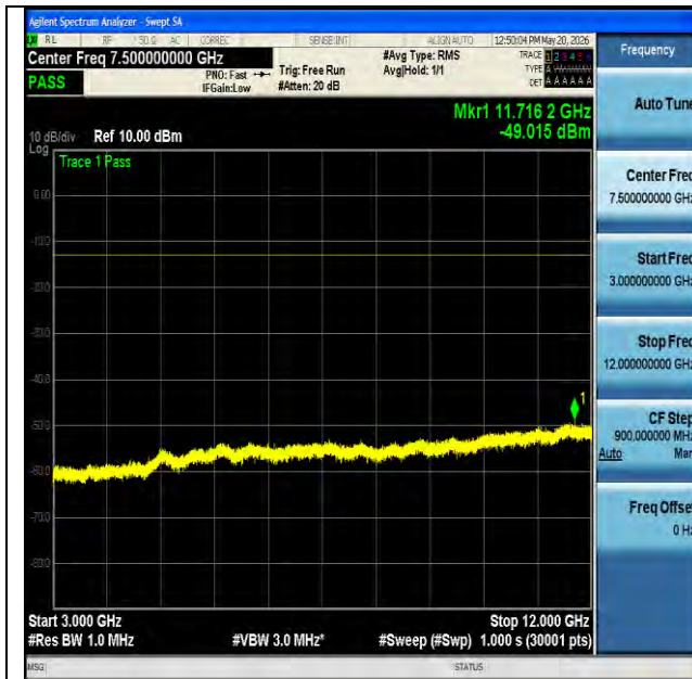
NTVN-n5-PC3-15-20-L-DFT-BPSK-Edge_1RB_Left-3000-12000- PASS
