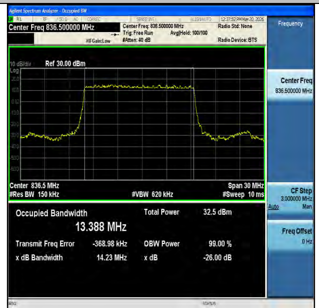
NTNV-n5-PC3-15-15-M-DFT-BPSK-Outer_Full-Ant1-PASS
