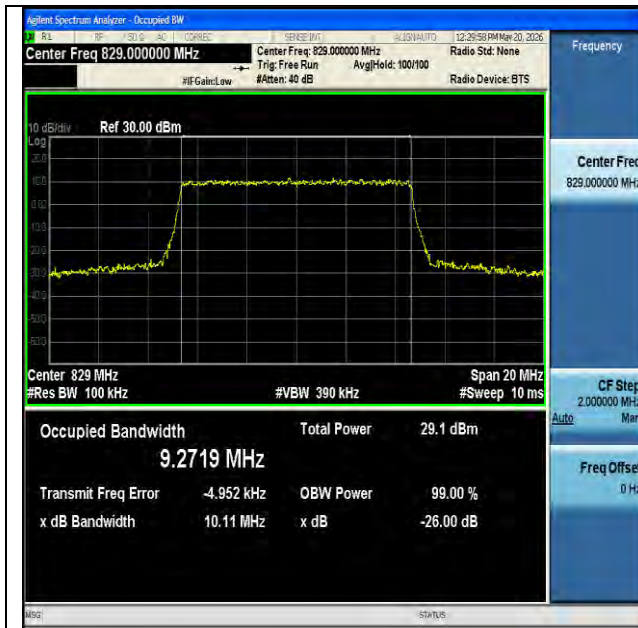
NTNV-n5-PC3-15-10-L-CP-QPSK-Outer_Full-Ant1-PASS
