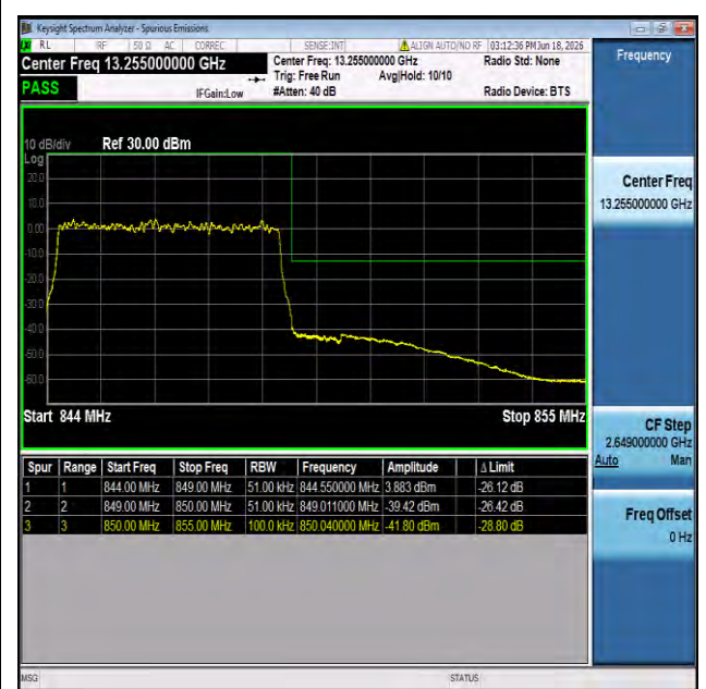
NTNV-n5-PC3-15-5-H-CP-QPSK-Outer_Full-PASS
