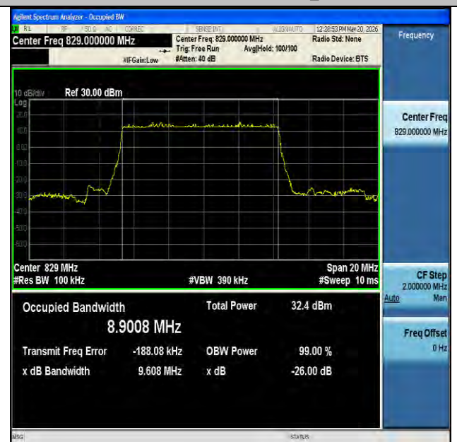
NTNV-n5-PC3-15-10-L-DFT-BPSK-Outer_Full-Ant1-PASS
