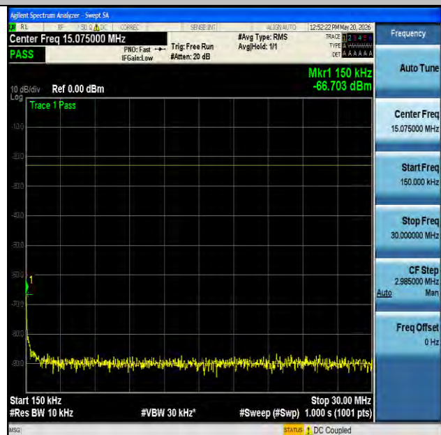
NTNV-n5-PC3-15-20-M-CP-QPSK-Edge_1RB_Left-0.15-30-PASS
