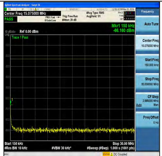
NTVN-n5-PC3-15-20-L-CP-QPSK-Edge_1RB_Left-0.15-30-PASS
