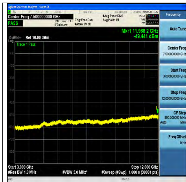
NTNV-n5-PC3-15-20-M-DFT-BPSK-Edge_1RB_Left-3000-12000- PASS
