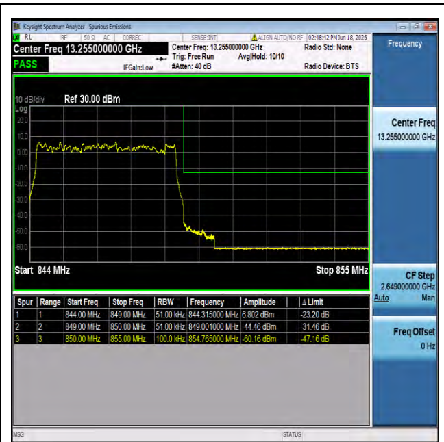
NTNV-n5-PC3-15-5-H-DFT-BPSK-Outer_Full-PASS
