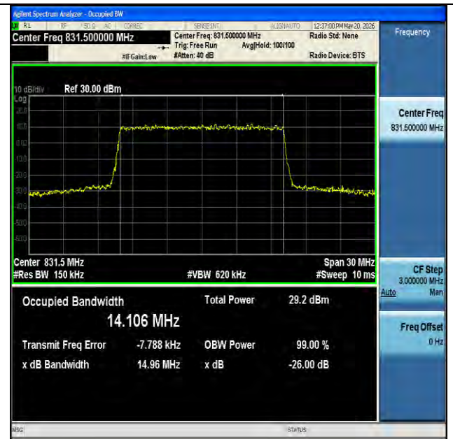
NTNV-n5-PC3-15-15-L-CP-64QAM-Outer_Full-Ant1-PASS
