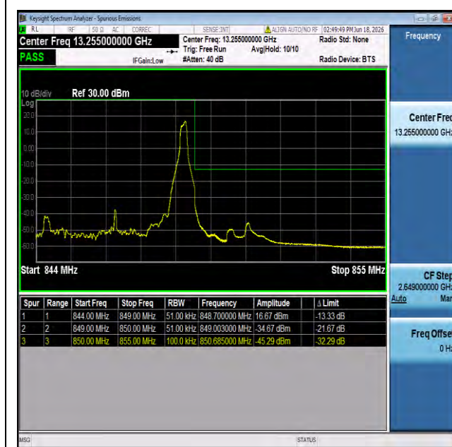
NTNV-n5-PC3-15-5-H-CP-QPSK-Edge_1RB_Right-PASS
