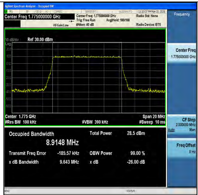
NTNV-n66-PC3-15-10-H-DFT-256QAM-Outer_Full-Ant1-PASS
