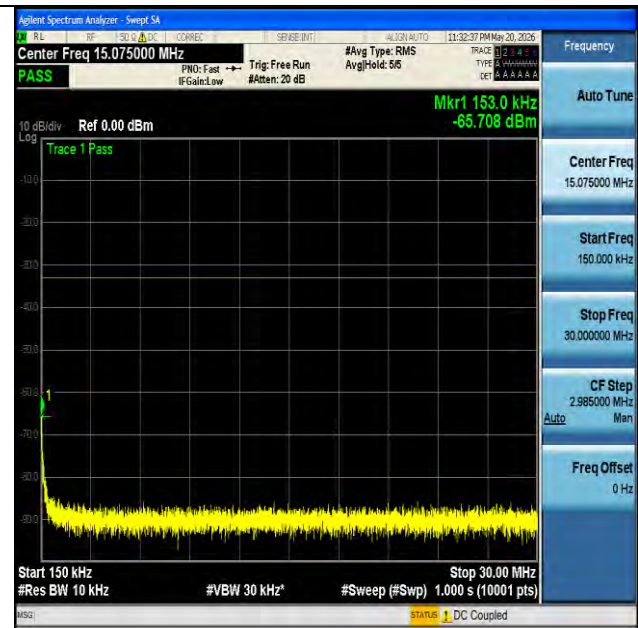
NTNV-n66-PC3-15-20-H-DFT-BPSK-Edge_1RB_Left-0.15-30- PASS
