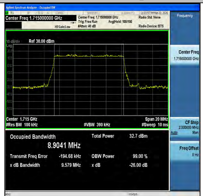
NTNV-n66-PC3-15-10-L-DFT-BPSK-Outer_Full-Ant1-PASS
