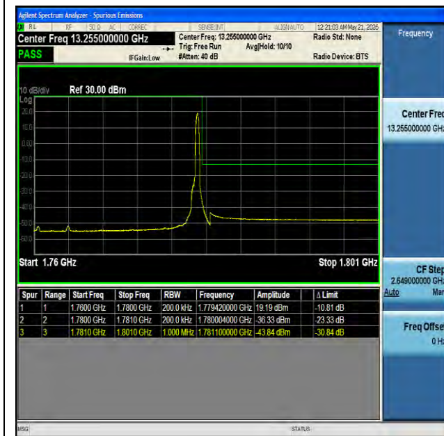
NTNV-n66-PC3-15-20-H-CP-QPSK-Edge_1RB_Right-PASS
