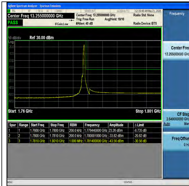
NTNV-n66-PC3-15-20-H-DFT-BPSK-Edge_1RB_Right-PASS
