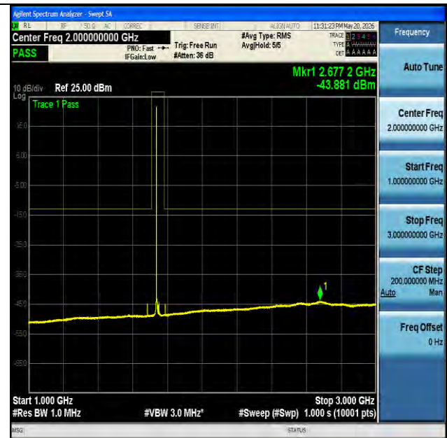
NTNV-n66-PC3-15-20-M-CP-QPSK-Edge_1RB_Left-1000-3000- PASS
