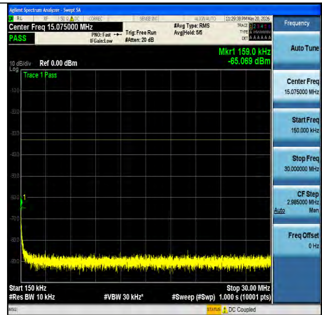
NTNV-n66-PC3-15-20-M-DFT-BPSK-Edge_1RB_Left-0.15-30- PASS
