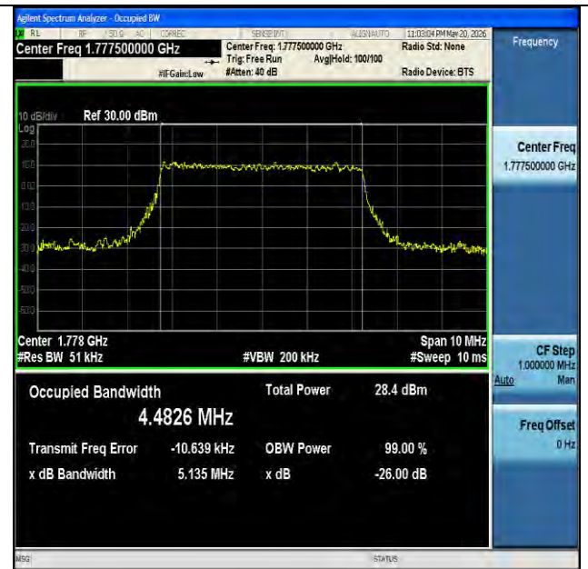
NTNV-n66-PC3-15-5-H-CP-64QAM-Outer_Full-Ant1-PASS
