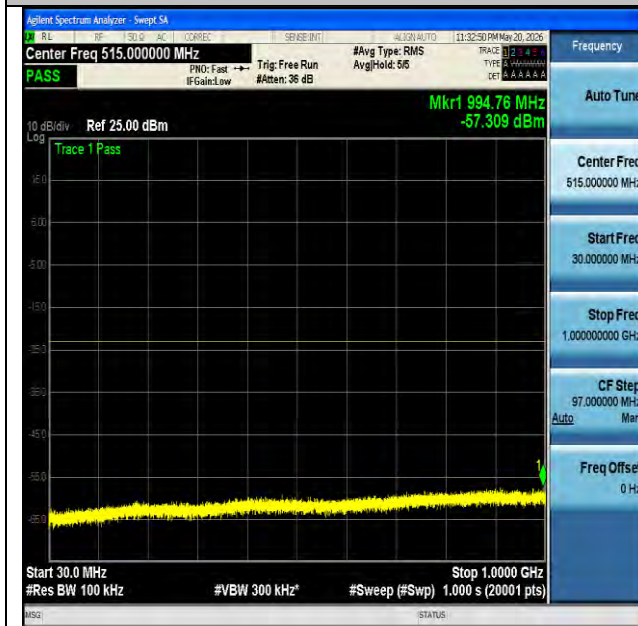
NTNV-n66-PC3-15-20-H-DFT-BPSK-Edge_1RB_Left-30-1000- PASS
