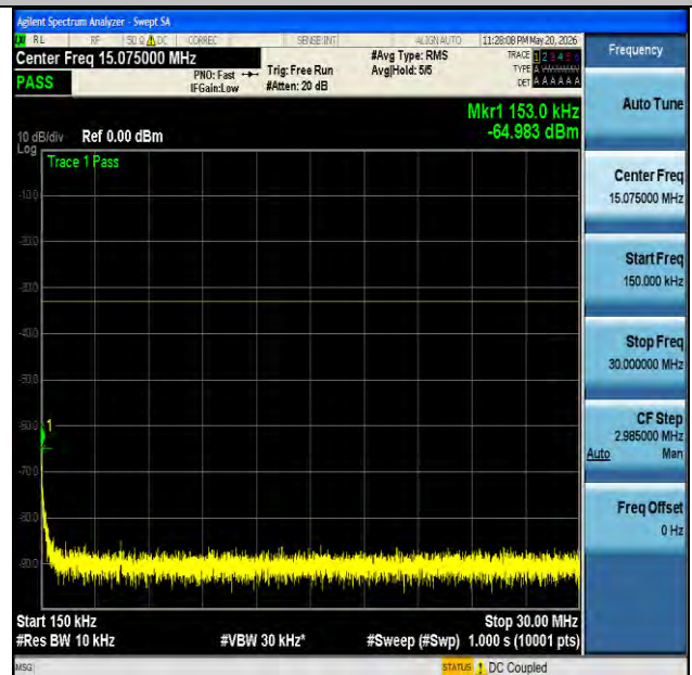
NTNV-n66-PC3-15-20-L-CP-QPSK-Edge_1RB_Left-0.15-30- PASS
