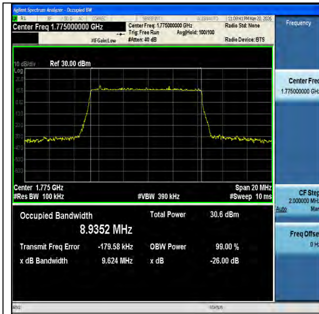
NTNV-n66-PC3-15-10-H-DFT-64QAM-Outer_Full-Ant1-PASS
