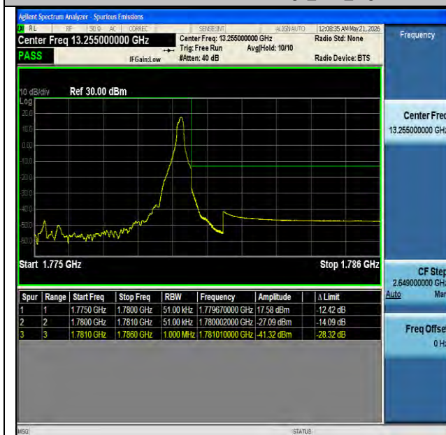
NTNV-n66-PC3-15-5-H-CP-QPSK-Edge_1RB_Right-PASS
