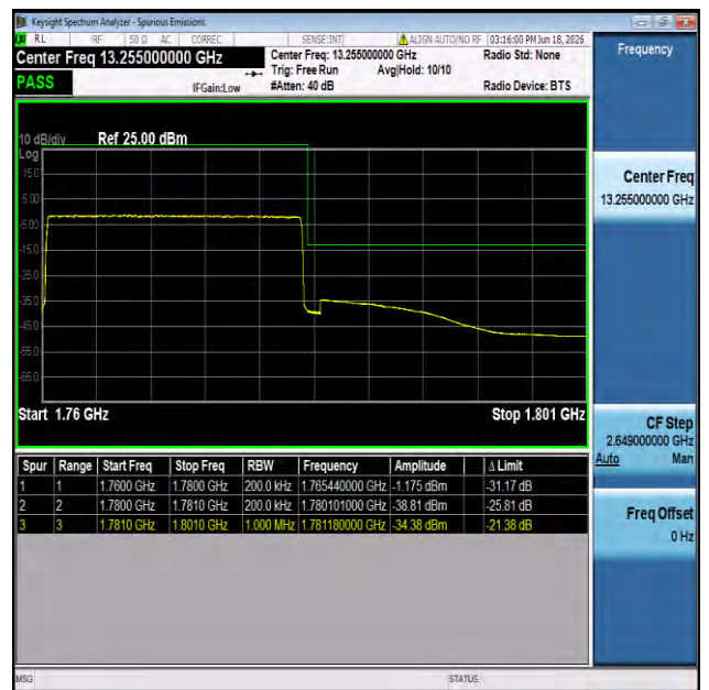
NTNV-n66-PC3-15-20-H-CP-QPSK-Outer_Full-PASS
