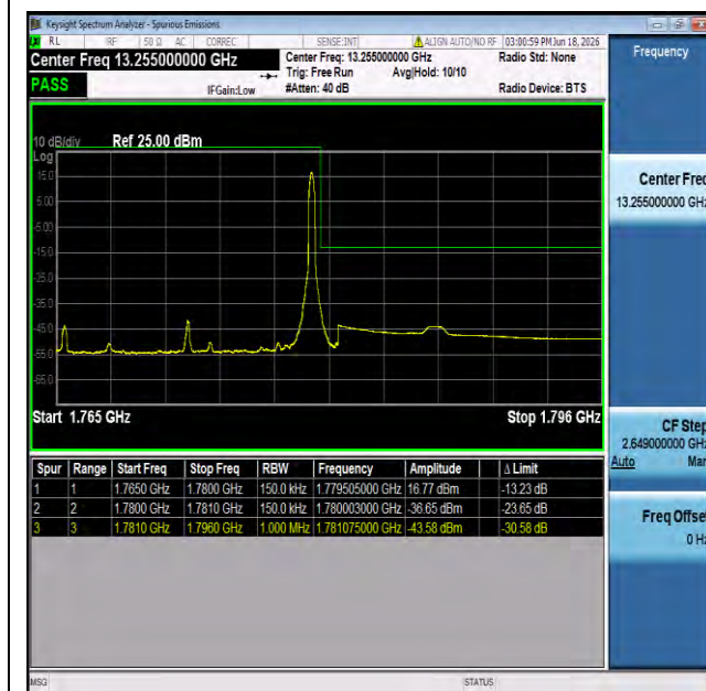
NTNV-n66-PC3-15-15-H-CP-QPSK-Edge_1RB_Right-PASS
