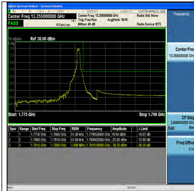
NTNV-n66-PC3-15-5-H-DFT-BPSK-Edge_1RB_Right-PASS
