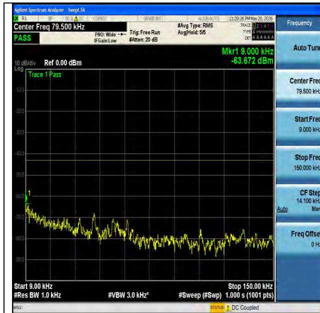
NTNV-n66-PC3-15-20-M-DFT-BPSK-Edge_1RB_Left-0.009-0.15- PASS
