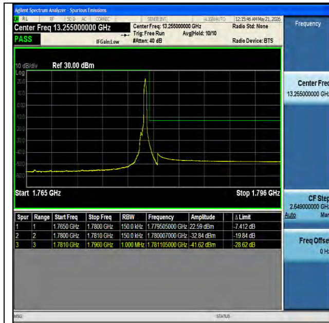
NTNV-n66-PC3-15-15-H-DFT-BPSK-Edge_1RB_Right-PASS
