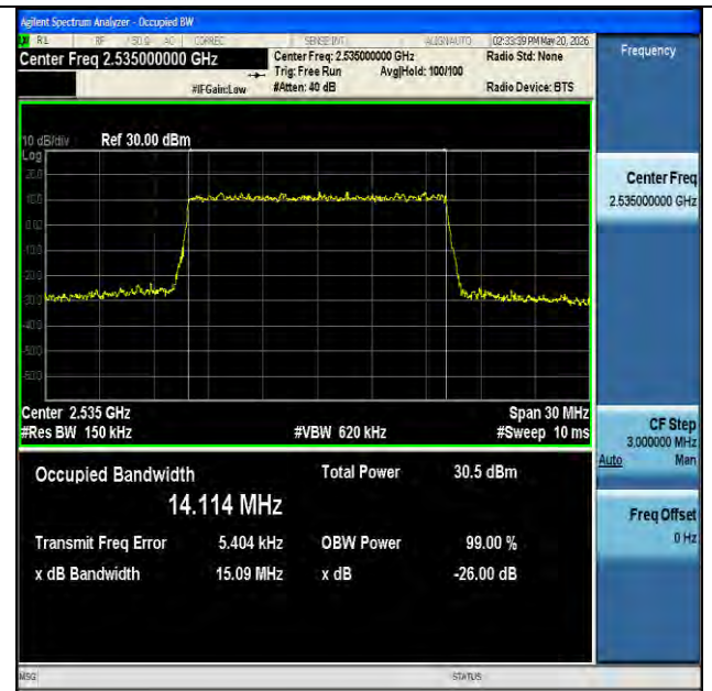
NTVN-n7-PC3-15-15-M-CP-16QAM-Outer_Full-Ant1-PASS
