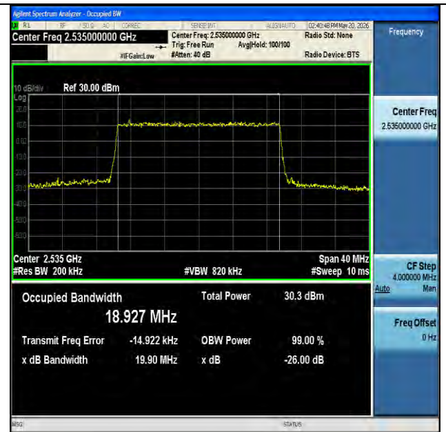
NTNV-n7-PC3-15-20-M-CP-64QAM-Outer_Full-Ant1-PASS
