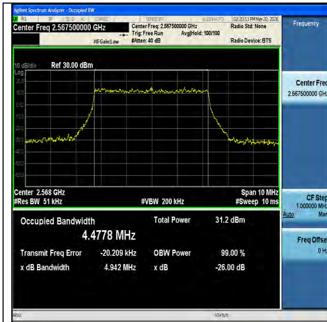
NTVN-n7-PC3-15-5-H-DFT-16QAM-Outer_Full-Ant1-PASS
