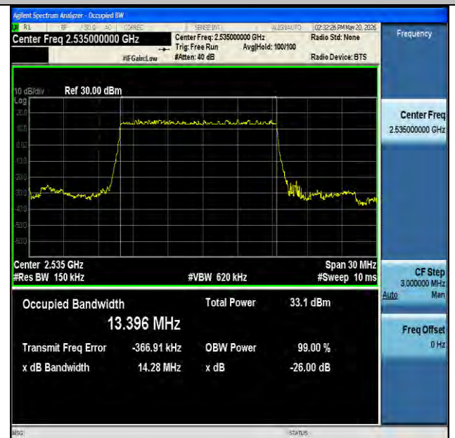
NTVN-n7-PC3-15-15-M-DFT-BPSK-Outer_Full-Ant1-PASS
