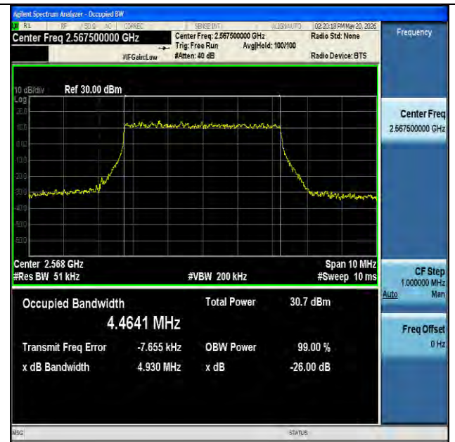
NTVN-n7-PC3-15-5-H-DFT-64QAM-Outer_Full-Ant1-PASS
