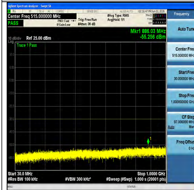
NTNV-n7-PC3-15-20-M-DFT-BPSK-Edge_1RB_Left-30-1000- PASS
