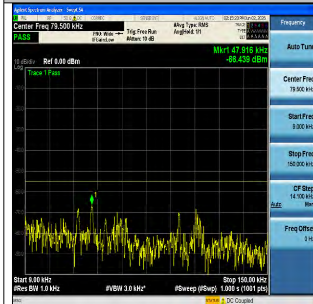
NTNV-n7-PC3-15-20-L-CP-QPSK-Edge_1RB_Left-0.009-0.15- PASS
