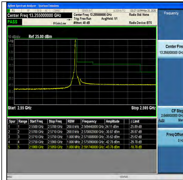
NTNV-n7-PC3-15-20-H-DFT-BPSK-Edge_1RB_Right-PASS
