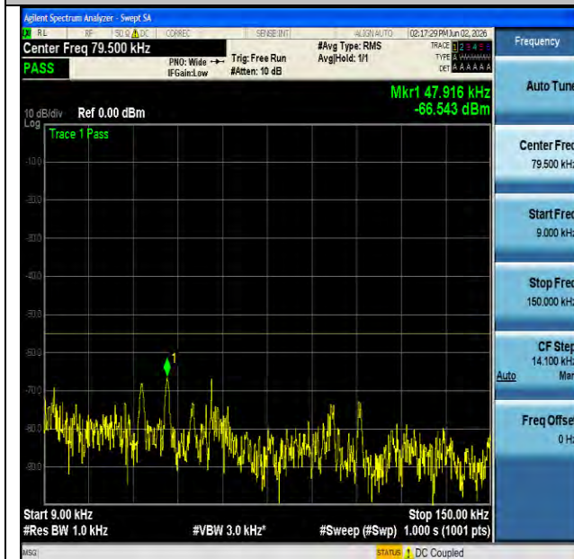
NTNV-n7-PC3-15-20-M-CP-QPSK-Edge_1RB_Left-0.009-0.15- PASS
