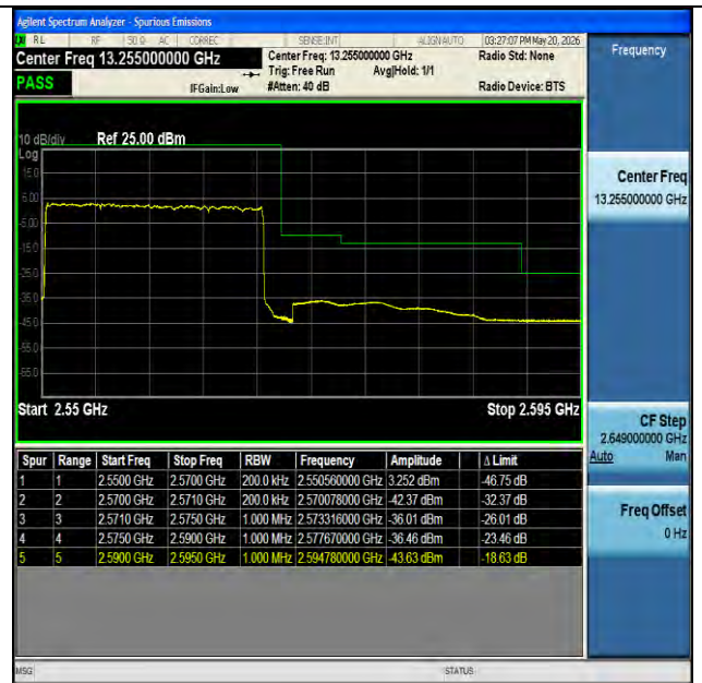
NTNV-n7-PC3-15-20-H-DFT-BPSK-Outer_Full-PASS
