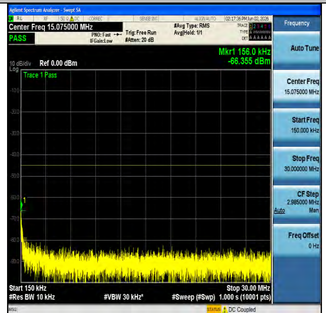
NTNV-n7-PC3-15-20-M-CP-QPSK-Edge_1RB_Left-0.15-30-PASS
