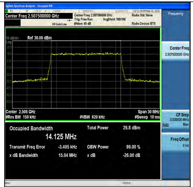
NTVN-n7-PC3-15-15-L-CP-64QAM-Outer_Full-Ant1-PASS
