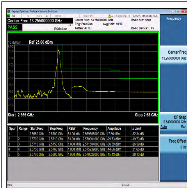
NTNV-n7-PC3-15-5-H-DFT-BPSK-Edge_1RB_Right-PASS
