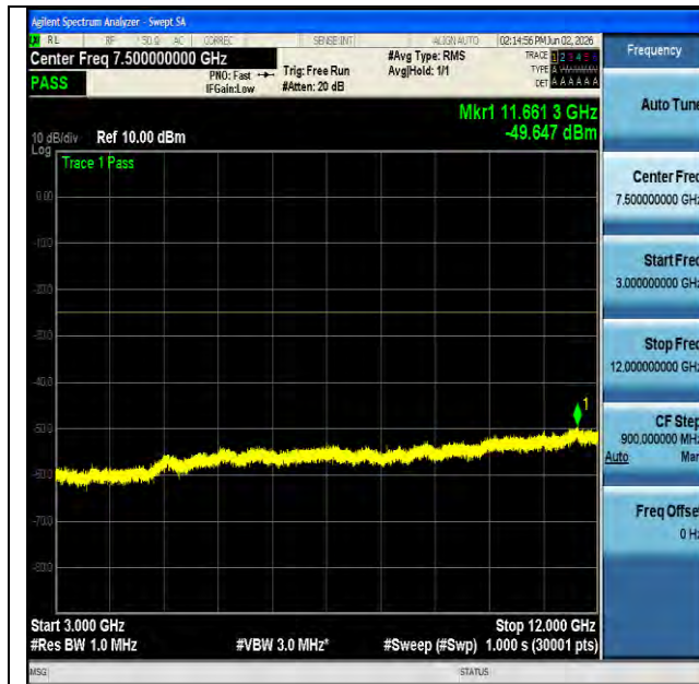
NTNV-n7-PC3-15-20-L-DFT-BPSK-Edge_1RB_Left-3000-12000- PASS
