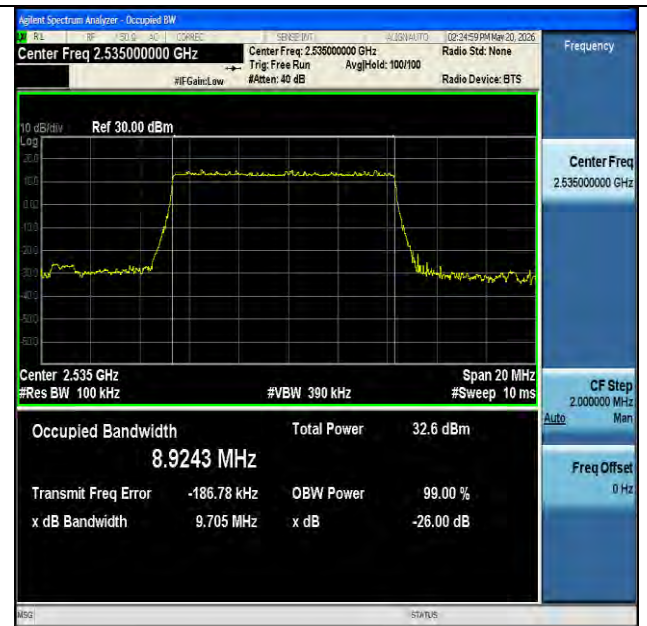
NTNV-n7-PC3-15-10-M-DFT-QPSK-Outer_Full-Ant1-PASS
