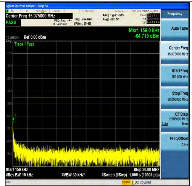
NTNV-n7-PC3-15-20-M-DFT-BPSK-Edge_1RB_Left-0.15-30- PASS
