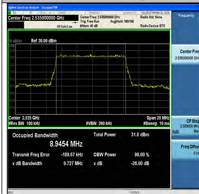
NTNV-n7-PC3-15-10-M-DFT-16QAM-Outer_Full-Ant1-PASS
