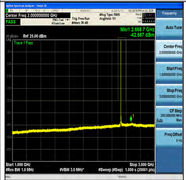
NTNV-n7-PC3-15-20-M-DFT-BPSK-Edge_1RB_Left-1000-3000- PASS
