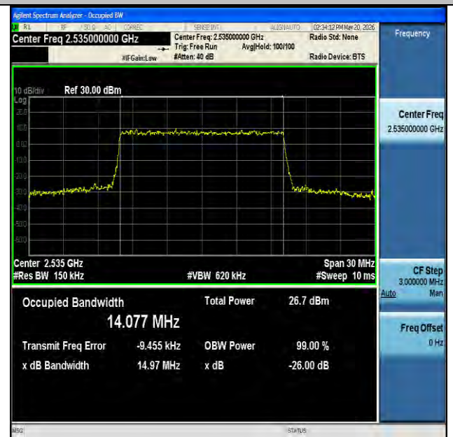
NTVN-n7-PC3-15-15-M-CP-256QAM-Outer_Full-Ant1-PASS
