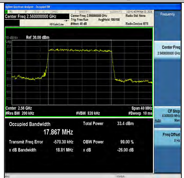
NTNV-n7-PC3-15-20-H-DFT-BPSK-Outer_Full-Ant1-PASS
