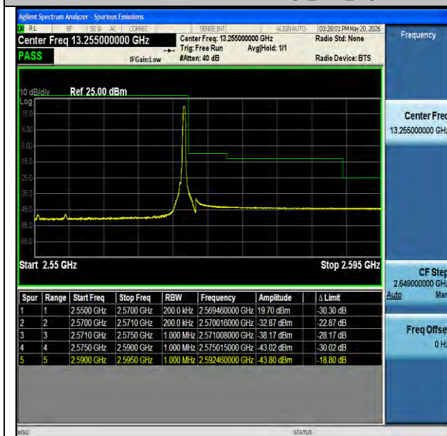
NTNV-n7-PC3-15-20-H-CP-QPSK-Edge_1RB_Right-PASS
