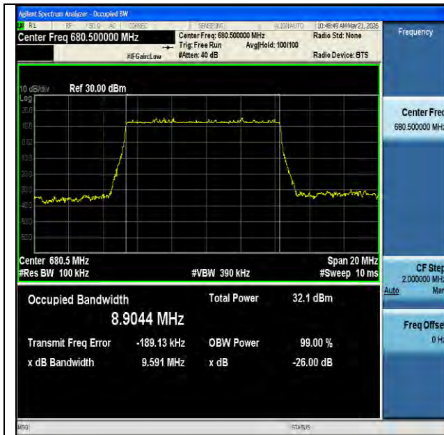
NTNV-n71-PC3-15-10-M-DFT-BPSK-Outter_Full-Ant1-PASS
