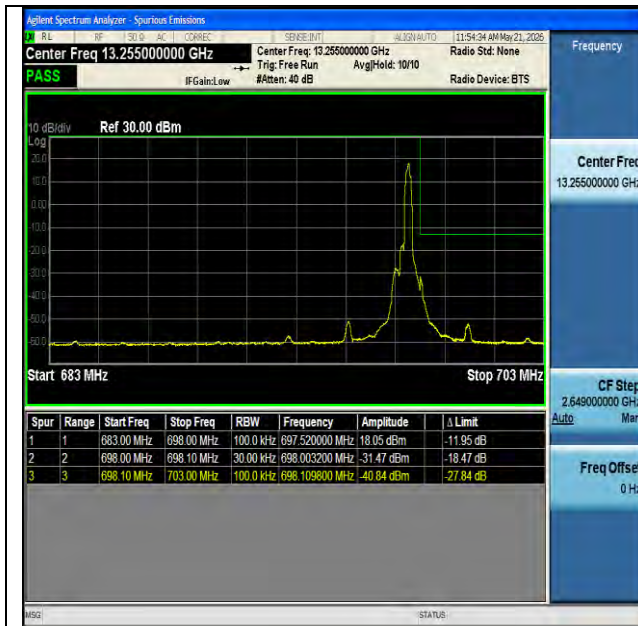
NTNV-n71-PC3-15-15-H-DFT-BPSK-Edge_1RB_Right-PASS
