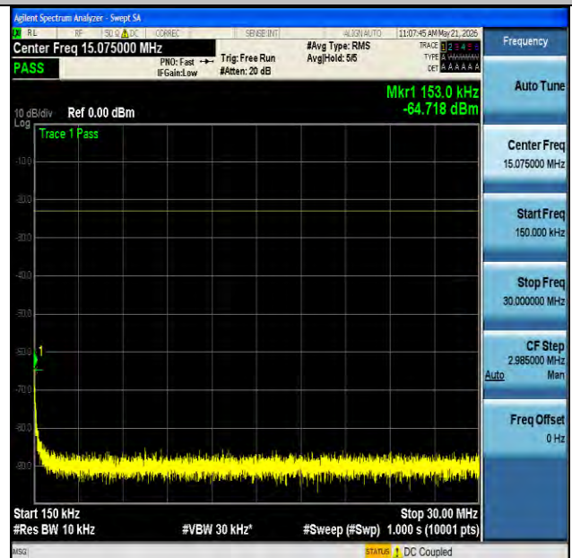
NTNV-n71-PC3-15-15-H-CP-QPSK-Edge_1RB_Left-0.15-30-PASS
