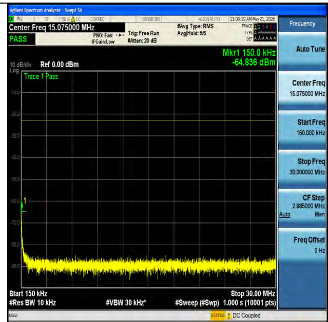
NTNV-n71-PC3-15-20-L-DFT-BPSK-Edge_1RB_Left-0.15-30- PASS
