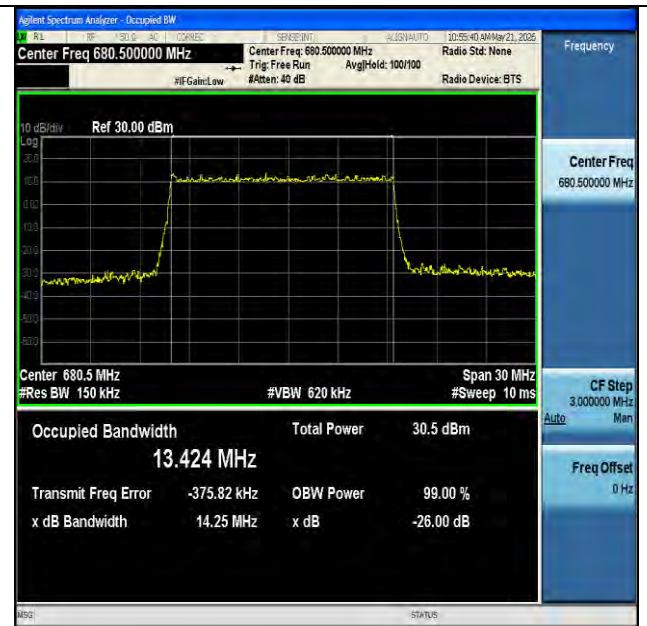
NTNV-n71-PC3-15-15-M-DFT-16QAM-Outet_Full-Ant1-PASS
