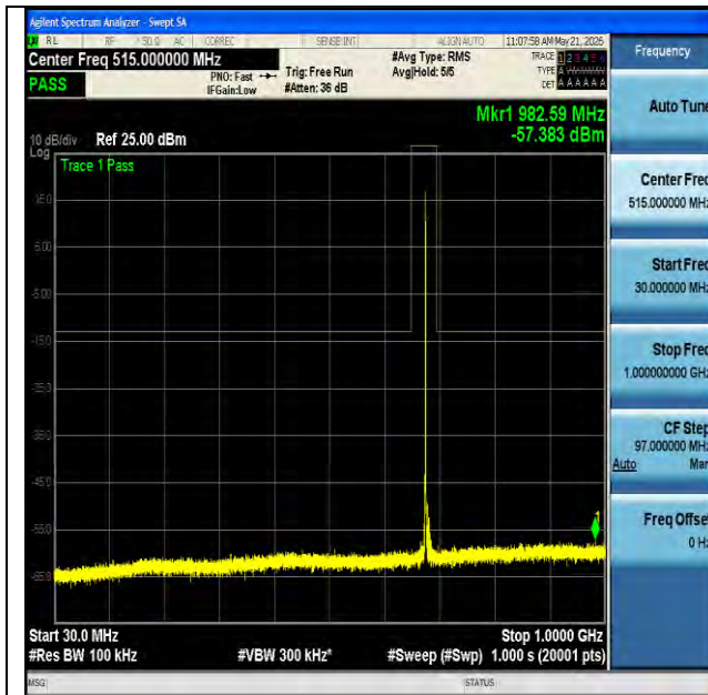
NTNV-n71-PC3-15-15-H-CP-QPSK-Edge_1RB_Left-30-1000- PASS
