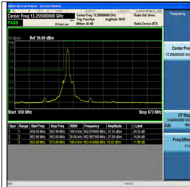
NTNV-n71-PC3-15-10-L-DFT-BPSK-Edge_1RB_Left-PASS
