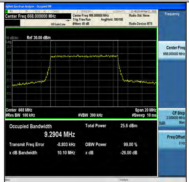
NTVN-n71-PC3-15-10-L-CP-256QAM-Outer_Full-Ant1-PASS
