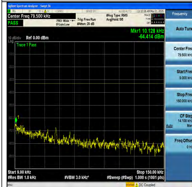
NTNV-n71-PC3-15-20-L-CP-QPSK-Edge_1RB_Left-0.009-0.15- PASS
