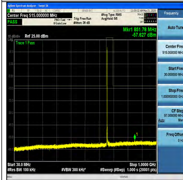
NTNV-n71-PC3-15-20-L-DFT-BPSK-Edge_1RB_Left-30-1000- PASS
