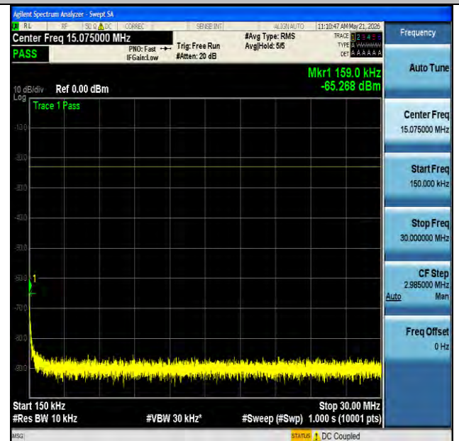
NTNV-n71-PC3-15-20-L-CP-QPSK-Edge_1RB_Left-0.15-30- PASS
