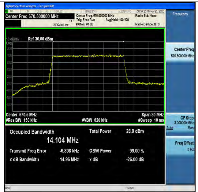
NTNV-n71-PC3-15-15-L-CP-64QAM-Outer_Full-Ant1-PASS
