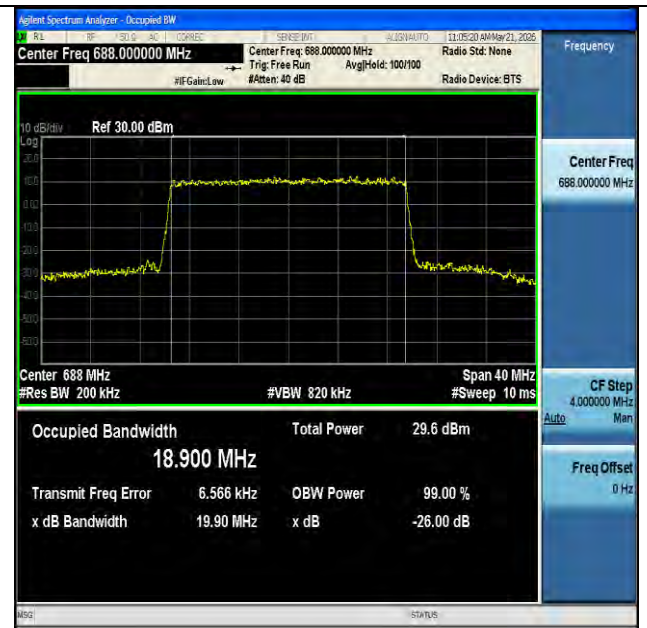
NTNV-n71-PC3-15-20-H-CP-16QAM-Outer_Full-Ant1-PASS
