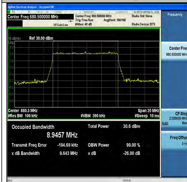
NTNV-n71-PC3-15-10-M-DFT-16QAM-Outter_Full-Ant1-PASS
