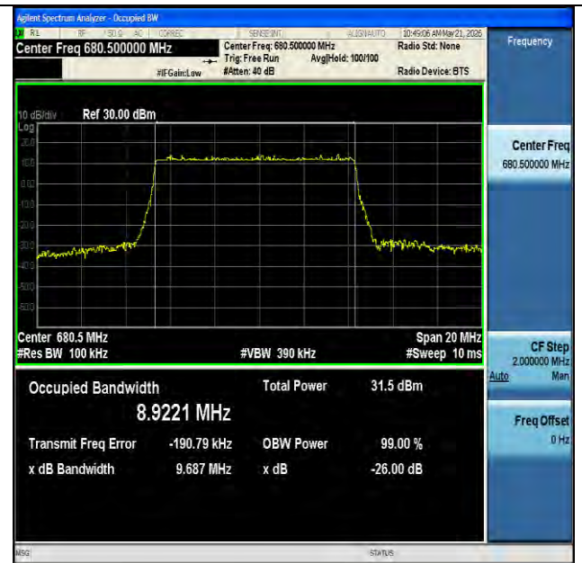
NTNV-n71-PC3-15-10-M-DFT-QPSK-Outter_Full-Ant1-PASS
