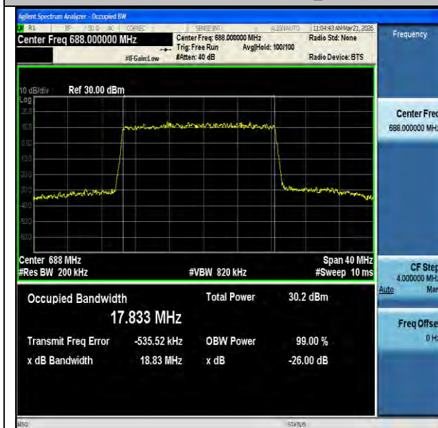
NTNV-n71-PC3-15-20-H-DFT-64QAM-Outet_Full-Ant1-PASS
