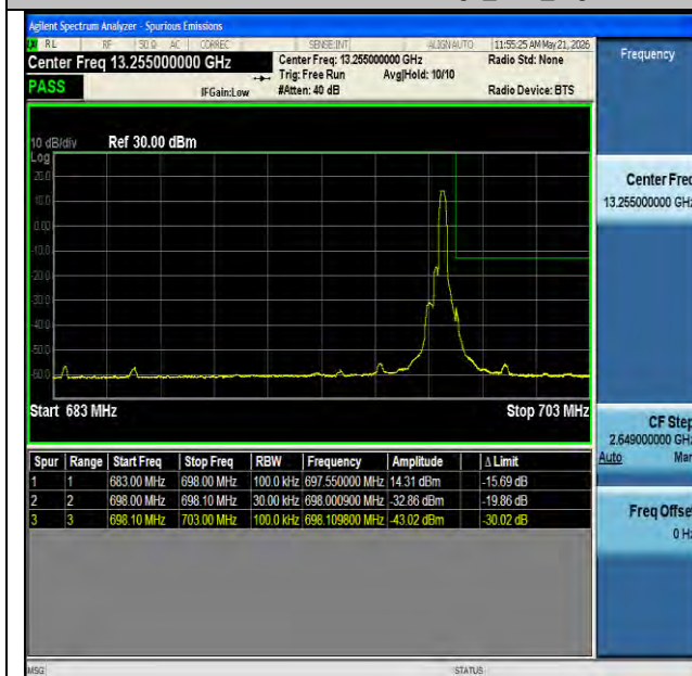
NTNV-n71-PC3-15-15-H-CP-QPSK-Edge_1RB_Right-PASS
