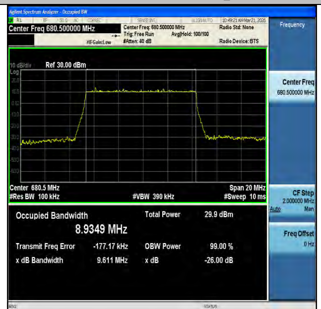
NTNV-n71-PC3-15-10-M-DFT-64QAM-Outter_Full-Ant1-PASS
