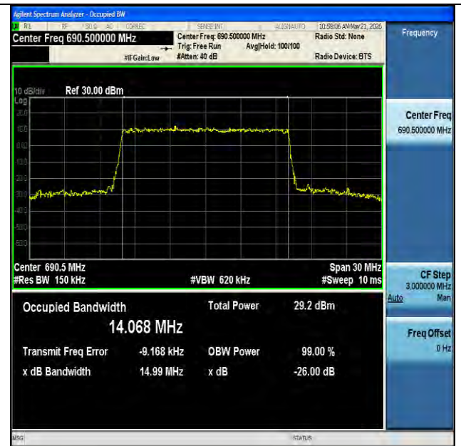
NTNV-n71-PC3-15-15-H-CP-QPSK-Outer_Full-Ant1-PASS
