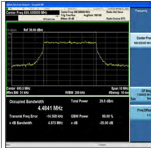
NTNV-n71-PC3-15-5-H-DFT-16QAM-Outer_Full-Ant1-PASS
