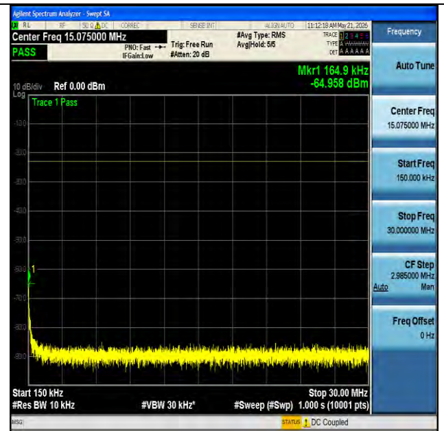
NTNV-n71-PC3-15-20-M-DFT-BPSK-Edge_1RB_Left-0.15-30- PASS
