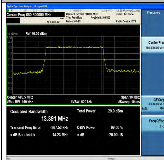
NTNV-n71-PC3-15-15-M-DFT-64QAM-Outet_Full-Ant1-PASS
