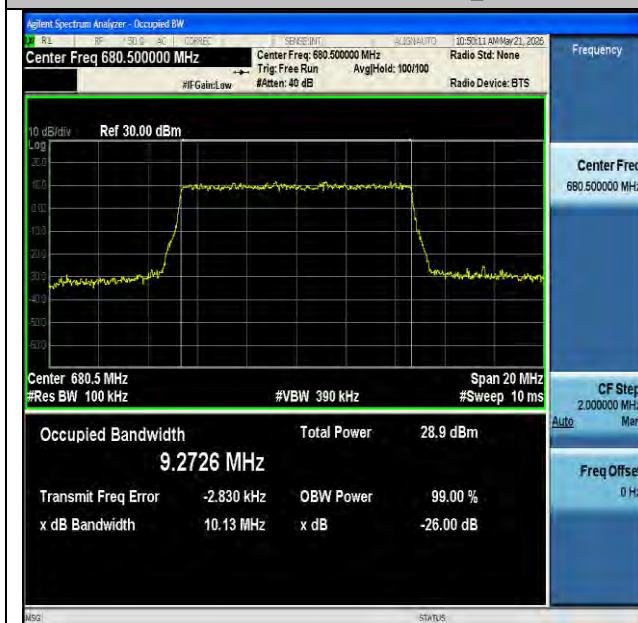
NTNV-n71-PC3-15-10-M-CP-16QAM-Outer_Full-Ant1-PASS
