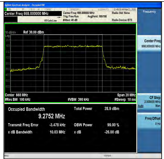
NTVN-n71-PC3-15-10-L-CP-16QAM-Outer_Full-Ant1-PASS
