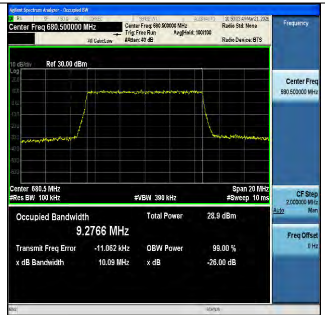
NTNV-n71-PC3-15-10-M-CP-QPSK-Outer_Full-Ant1-PASS
