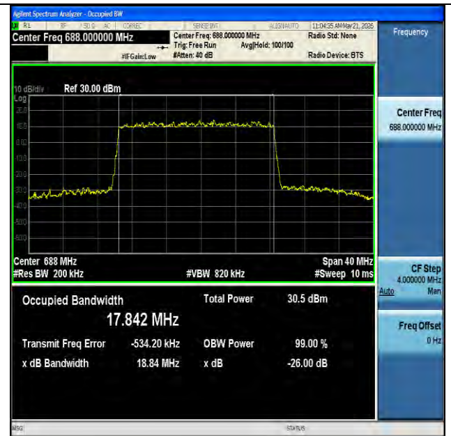
NTNV-n71-PC3-15-20-H-DFT-16QAM-Outet_Full-Ant1-PASS
