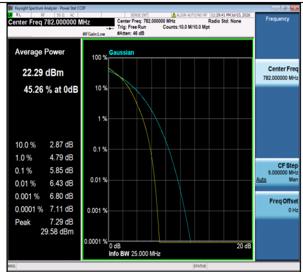
Band13-10MHz-16QAM-23230-50RB#0-PASS
