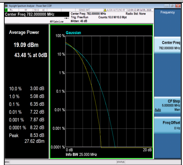
Band13-10MHz-256QAM-23230-50RB#0-PASS
