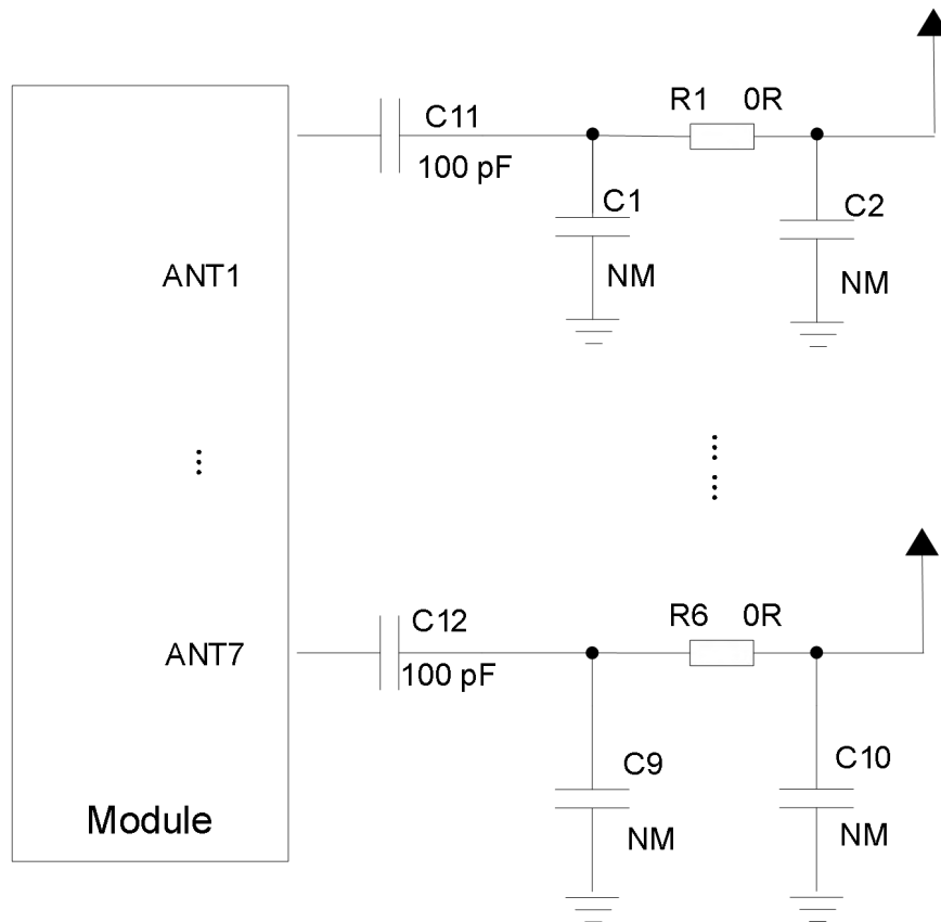
Figure 37: Reference Design of Cellular Antennas
