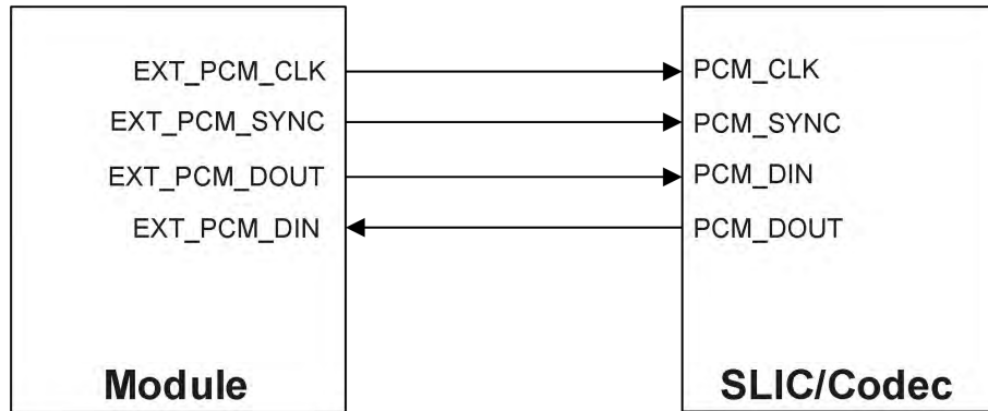
Figure 27: Reference Circuit of PCM Interface for SLIC or Codec
