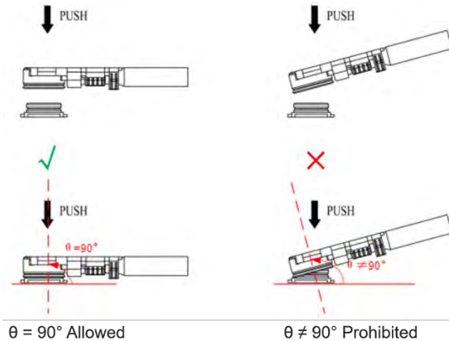
Figure 45: Plug in a Coaxial Cable Plug
