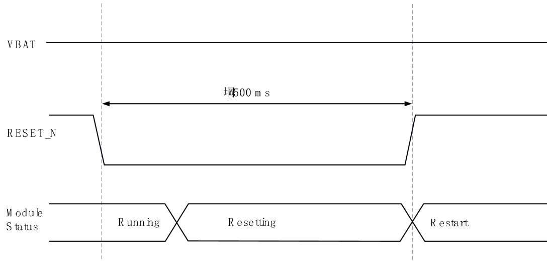
Figure 16: Reset Timing
