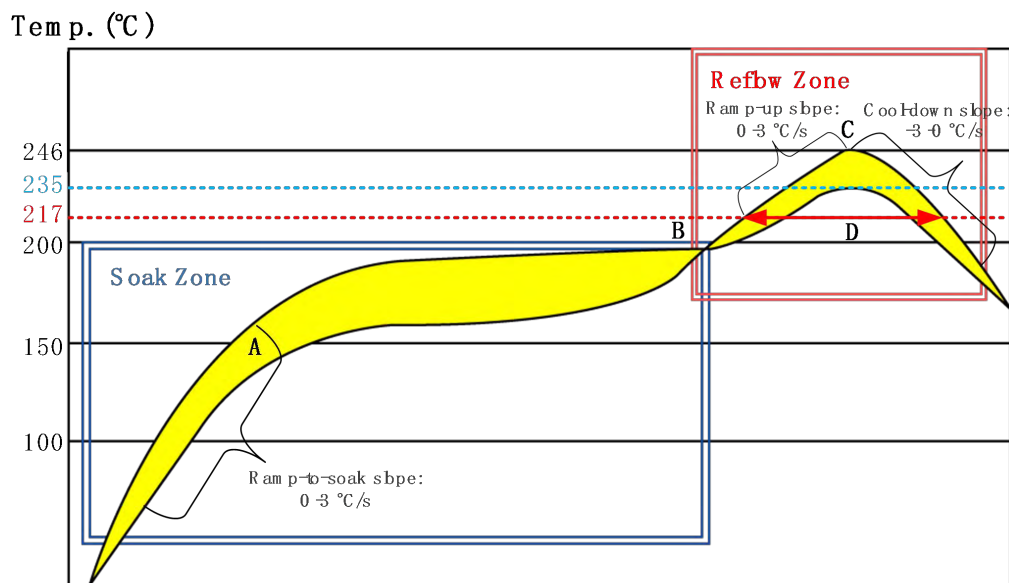
Figure 53: Recommended Reflow Soldering Thermal Profile
