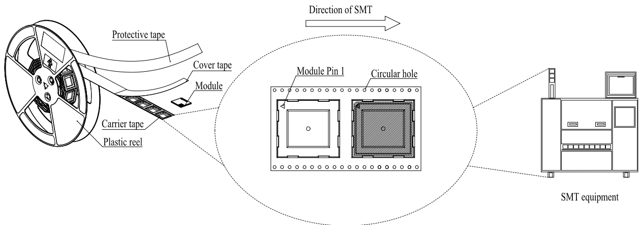
Figure 56: Mounting Direction
