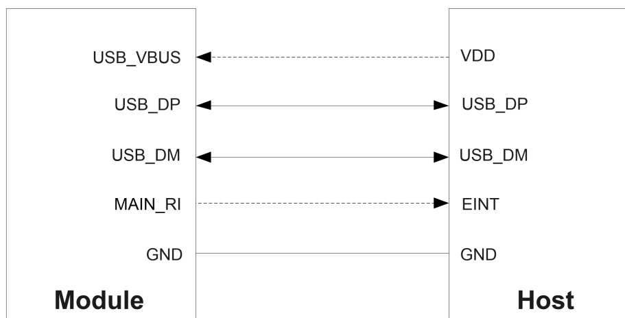
Figure 5: Block Diagram of Application with MAIN_RI Function in Sleep Mode
