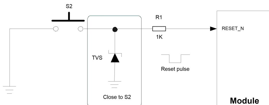
Figure 15: Reference Design of Reset with Keystroke
