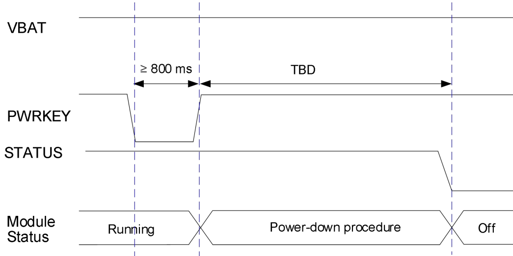
Figure 13: Turn-off Timing with PWRKEY
