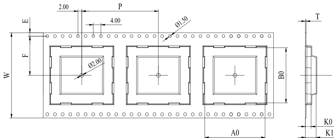
Figure 54: Carrier Tape Dimension Drawing (Unit: mm)
