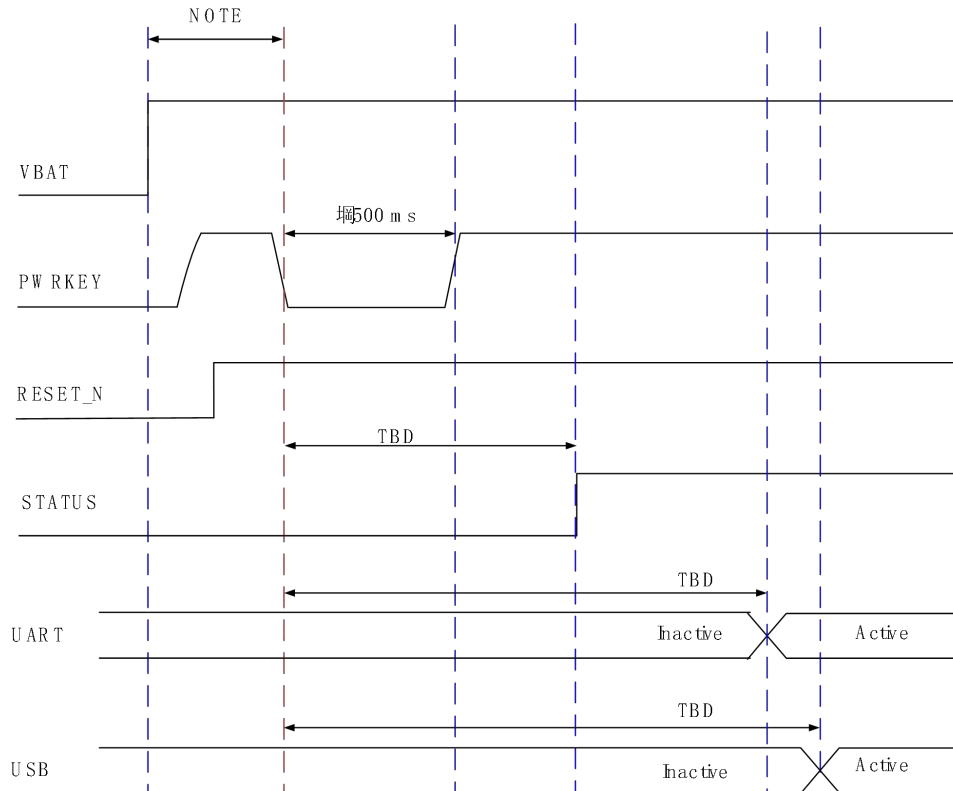
Figure 12: Turn-on Timing with PWRKEY
