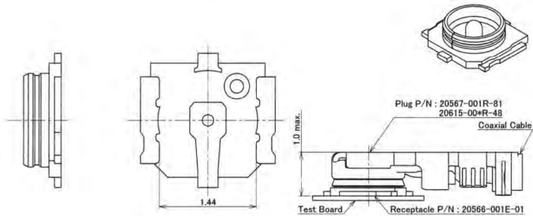
Figure 43: Dimensions of the Receptacles (Unit: mm)
