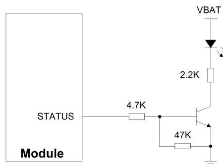
Figure 36: Reference Design of STATUS
