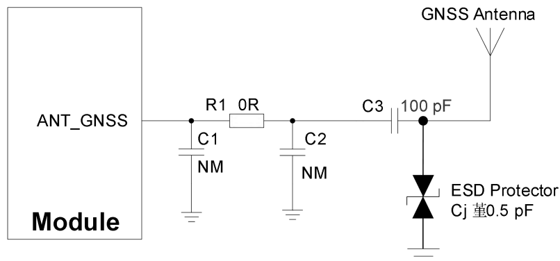
Figure 38: Reference Design of GNSS Antenna
