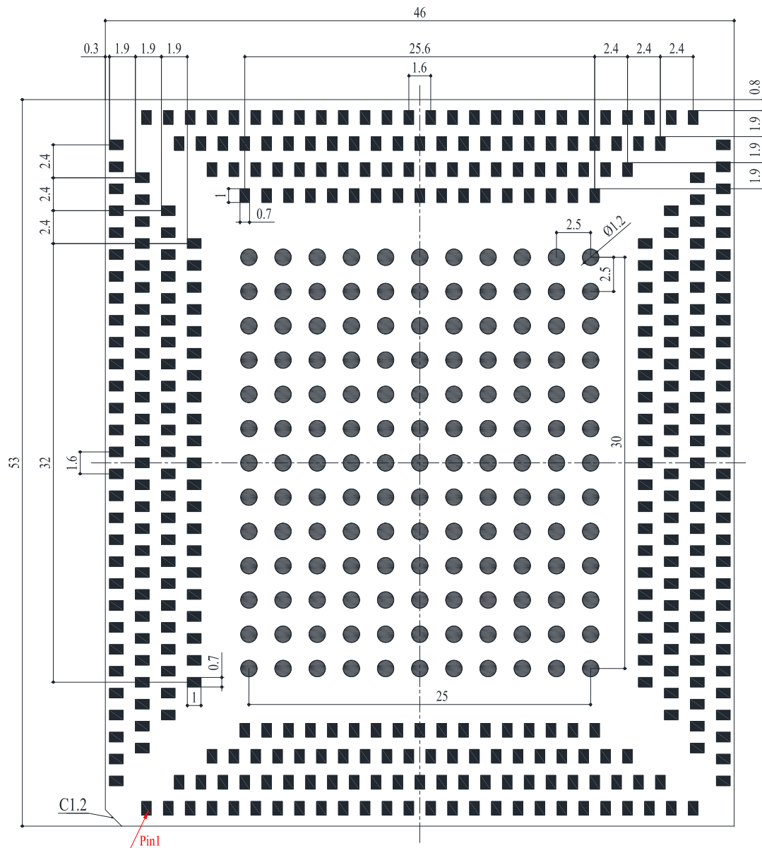
Figure 51: Recommended Footprint
