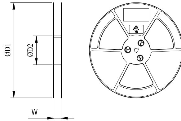
Figure 55: Plastic Reel Dimension Drawing
