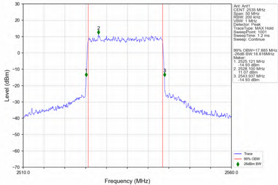
n7_15kHz_SISO_NTNV_20MHz_DFT-s-OFDM_64 QAM_2535MHz_Outer_Full_Ant1
