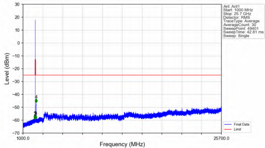
n7_15kHz_SISO_NTNV_15MHz_CP-OFDM QPSK_2535MHz_Edge_1RB_Left_Ant1
