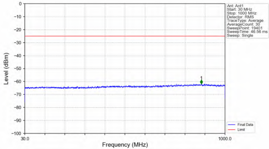
n7_15kHz_SISO_NTNV_15MHz_CP-OFDM QPSK_2535MHz_Edge_1RB_Left_Ant1
