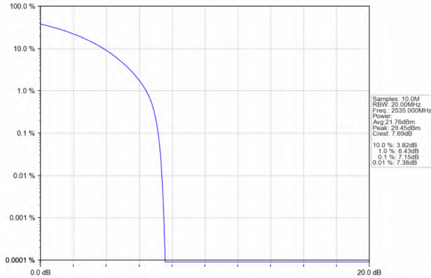
n7_15kHz_SISO_NTNV_20MHz_CP-OFDM QPSK_2535MHz_Outer_Full_Ant1
