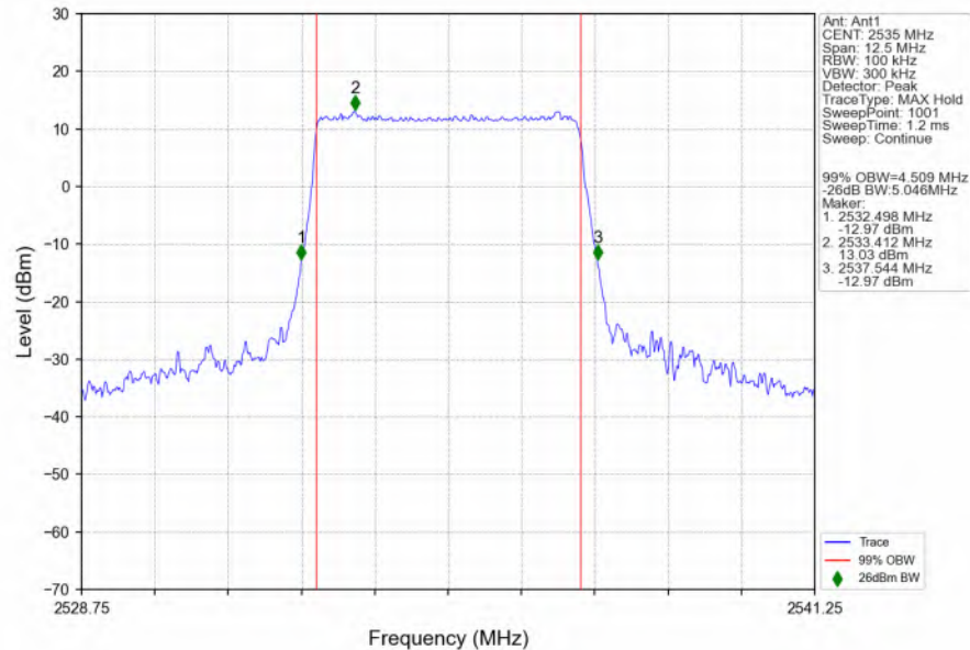
n7_15kHz_SISO_NTNV_5MHz_DFT-s-OFDM_64_QAM_2535MHz_Outer_Full_Ant1
