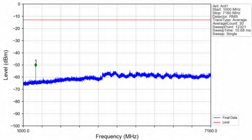
n12_15kHz_SISO_NTNV_5MHz_CP-OFDM_QPSK_707.5MHz_Edge_1RB_Left_Ant1
