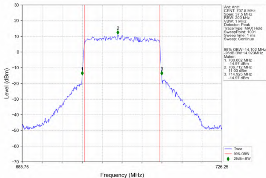
n12_15kHz_SISO_NTNV_15MHz_CP-OFDM 64 QAM_707.5MHz_Outer_Full_Ant1
