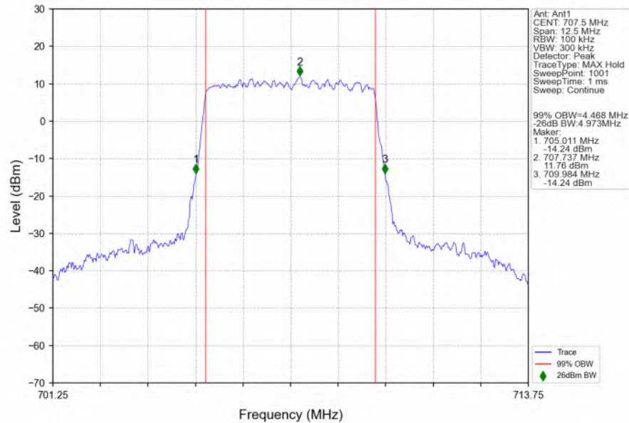
n12_15kHz_SISO_NTNV_5MHz_CP-OFDM 64 QAM_707.5MHz_Outer_Full_Ant1
