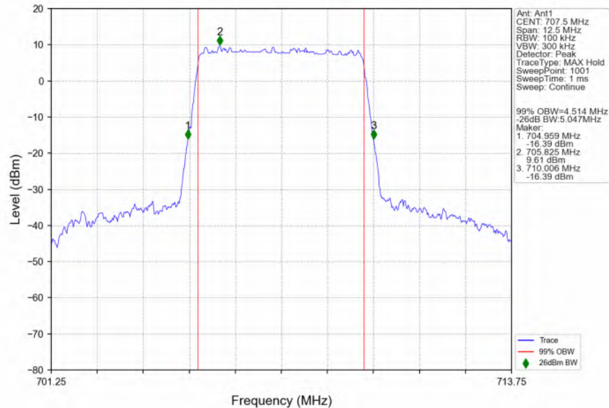
n12_15kHz_SISO_NTNV_5MHz_CP-OFDM_QPSK_707.5MHz_Outer_Full_Ant1
