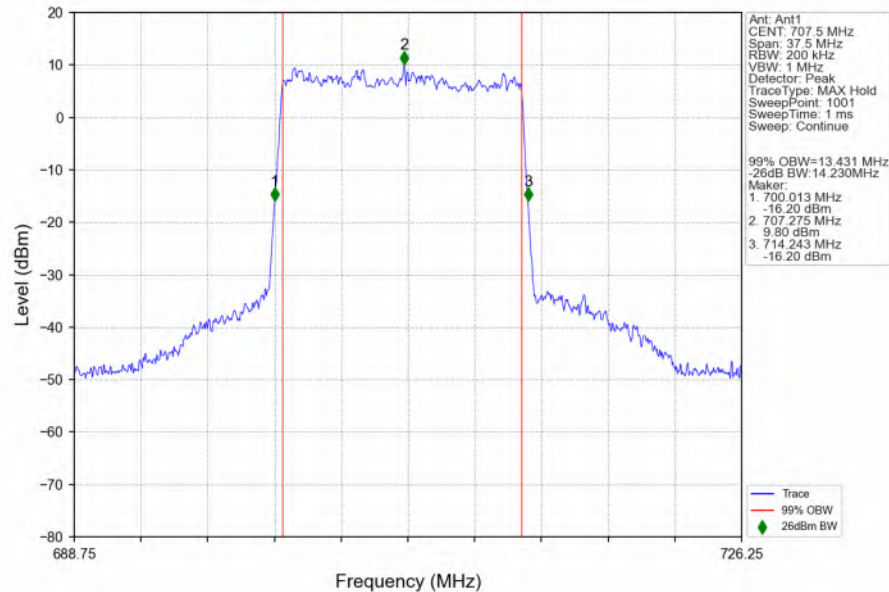
n12_15kHz_SISO_NTNV_15MHz_CP-OFDM QPSK_707.5MHz_Outer_Full_Ant1
