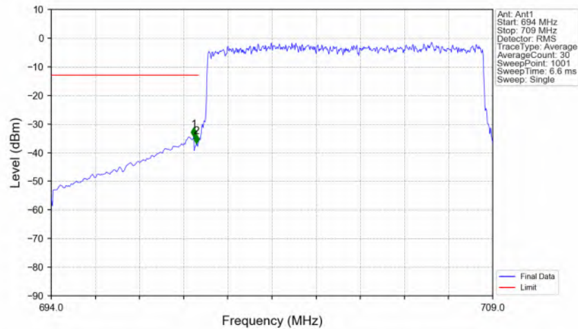
n12_15kHz_SISO_NTNV_10MHz_CP-OFDM QPSK_704MHz_Outer_Full_Ant1
