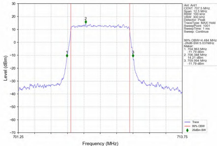
n12_15kHz_SISO_NTNV_5MHz_CP-OFDM_QPSK_707.5MHz_Outer_Full_Ant1
