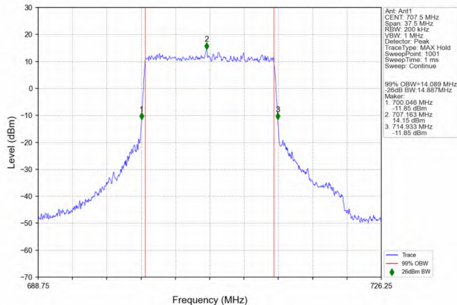
n12_15kHz_SISO_NTNV_15MHz_CP-OFDM QPSK_707.5MHz_Outer_Full_Ant1
