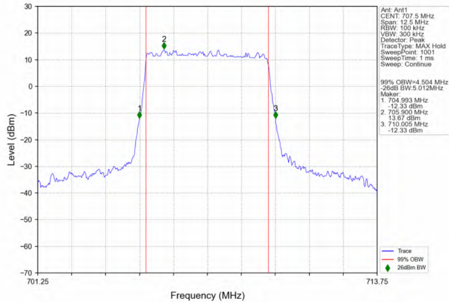
n12_15kHz_SISO_NTNV_5MHz_DFT-s-OFDM 64 QAM 707.5MHz_Outer_Full_Ant1
