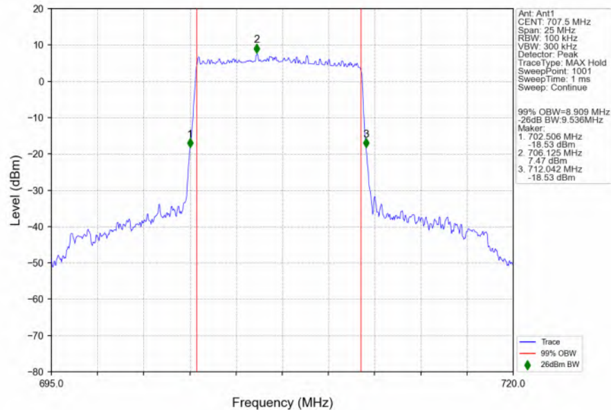
n12_15kHz_SISO_NTNV_10MHz_CP-OFDM QPSK_707.5MHz_Outer_Full_Ant1
