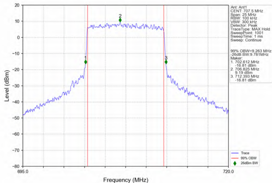
n12_15kHz_SISO_NTNV_10MHz_CP-OFDM 64 QAM_707.5MHz_Outer_Full_Ant1
