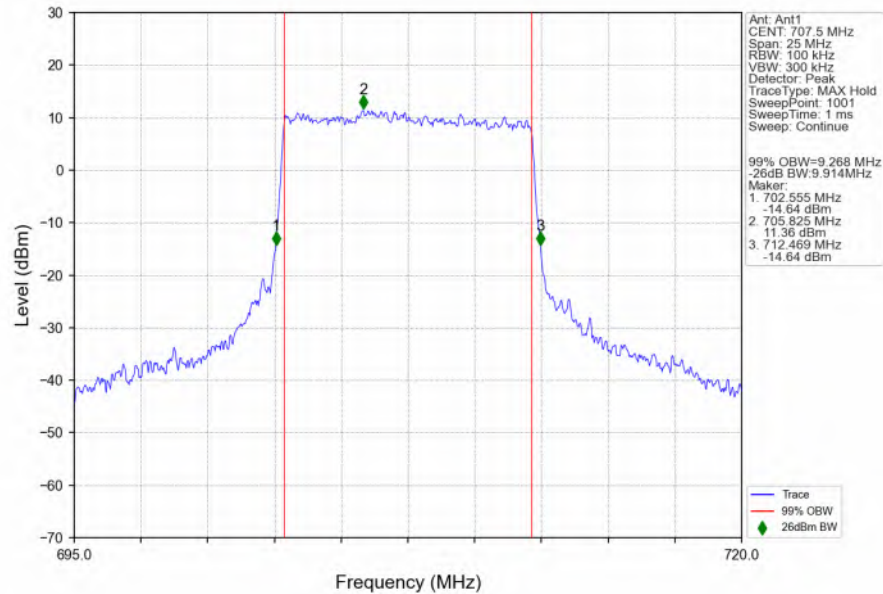
n12_15kHz_SISO_NTNV_10MHz_CP-OFDM QPSK_707.5MHz_Outer_Full_Ant1
