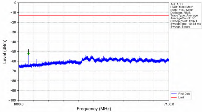
n12_15kHz_SISO_NTNV_10MHz_CP-OFDM QPSK_704MHz_Edge_1RB_Left_Ant1
