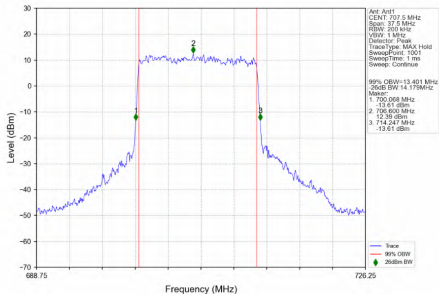
n12_15kHz_SISO_NTNV_15MHz_DFT-s-OFDM 64 QAM_707.5MHz_Outer_Full_Ant1
