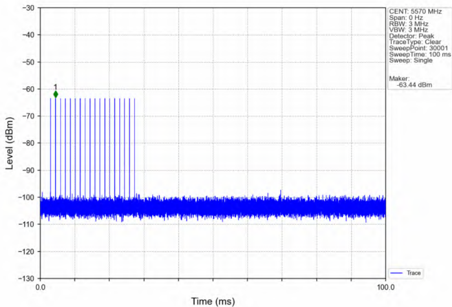
Signal Calibration_802.11ax(HEW160)_2C_5570MHz_RadarType0_Trial0
