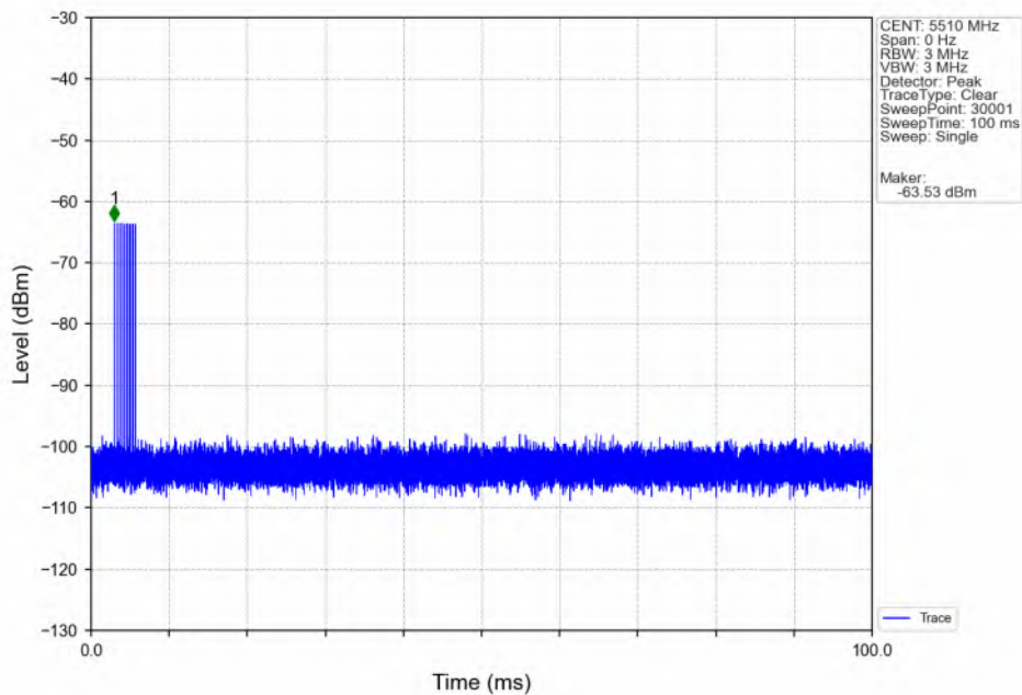
Signal Calibration_802.11ax(HEW40)_2C_5510MHz_RadarType6_Trial0
