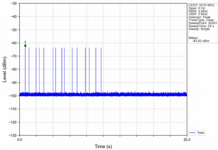
Signal Calibration_802.11ax(HEW40)_2C_5510MHz_RadarType6_Trial0
