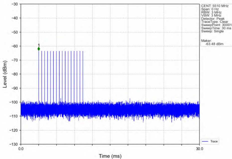
Signal Calibration_802.11ax(HEW40)_2C_5510MHz_RadarType4_Trial0
