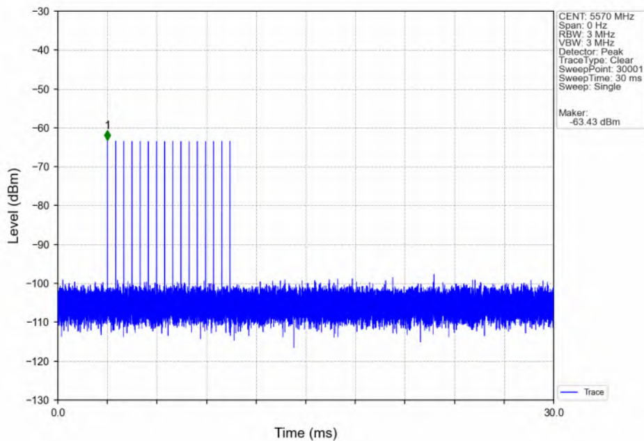
Signal Calibration_802.11ax(HEW160)_2C_5570MHz_RadarType4_Trial0
