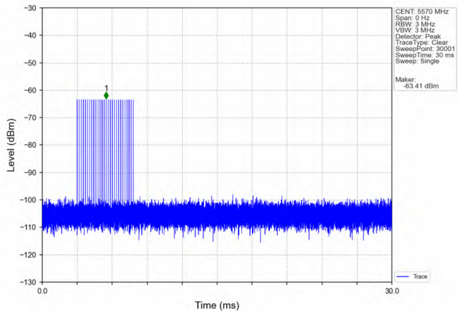
Signal Calibration_802.11ax(HEW160)_2C_5570MHz_RadarType2_Trial0
