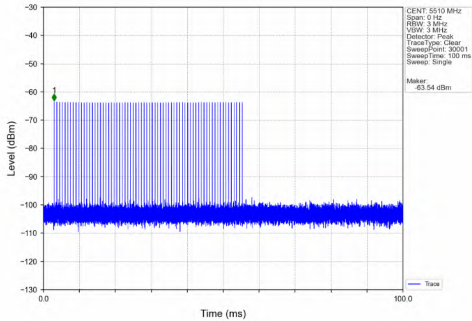
Signal Calibration_802.11ax(HEW40)_2C_5510MHz_RadarType2_Trial0
