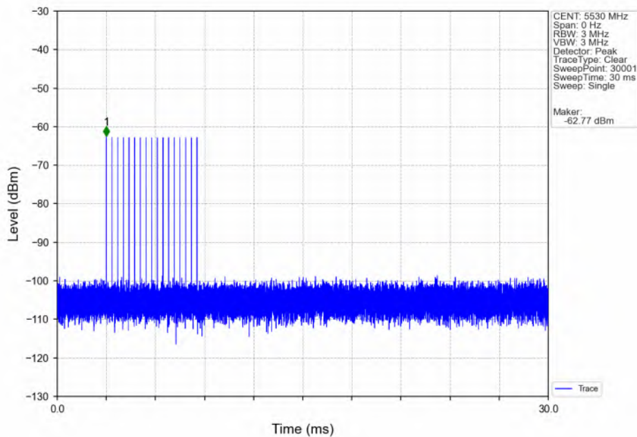
Signal Calibration_802.11ax(HEW80)_2C_5530MHz_RadarType3_Trial0
