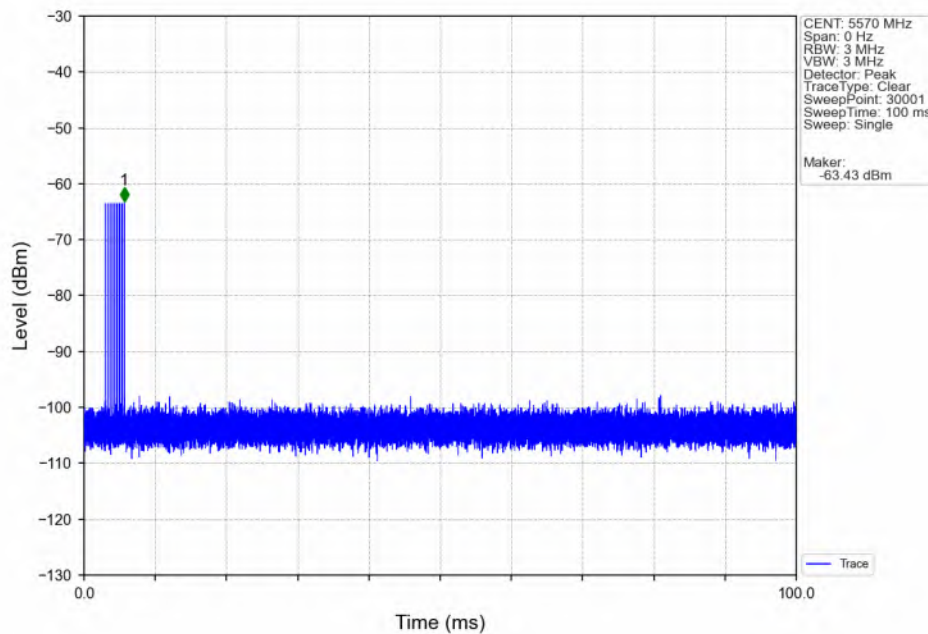
Signal Calibration_802.11ax(HEW160)_2C_5570MHz_RadarType6_Trial0
