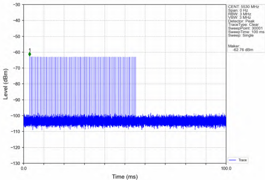
Signal Calibration_802.11ax(HEW80)_2C_5530MHz_RadarType1_Trial0
