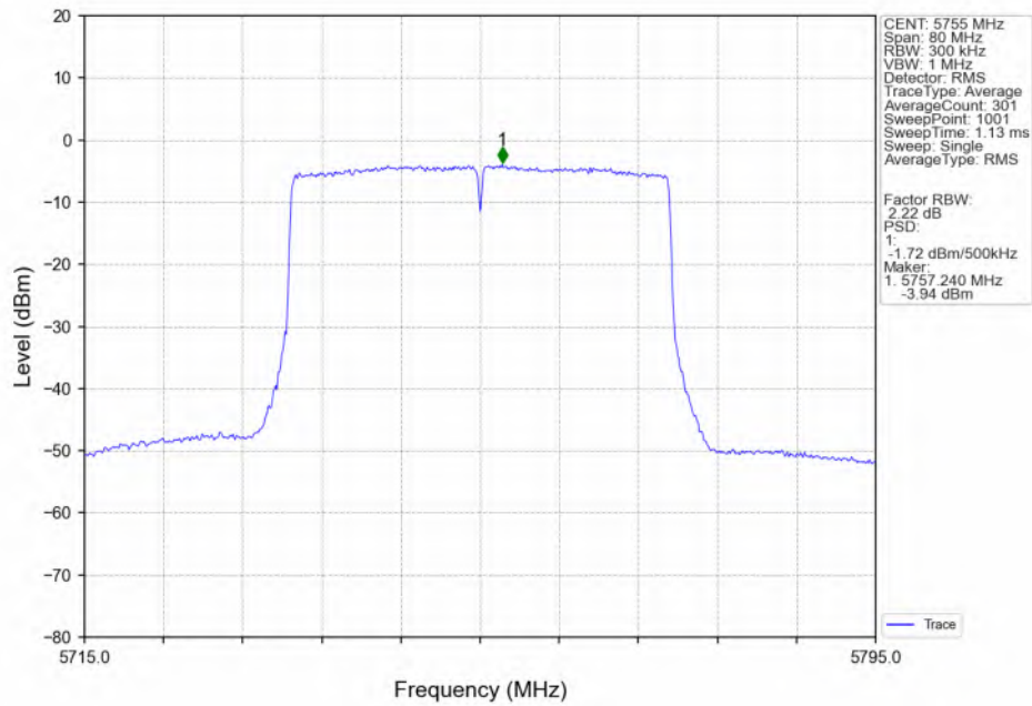
802.11ax(HEW40)_LCH_5755MHz_SU / MIMO_NTNV
