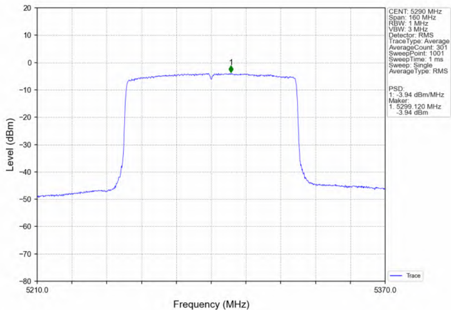
802.11ax(HEW80)_MCH_5290MHz_SU / Ant2_NTNV
