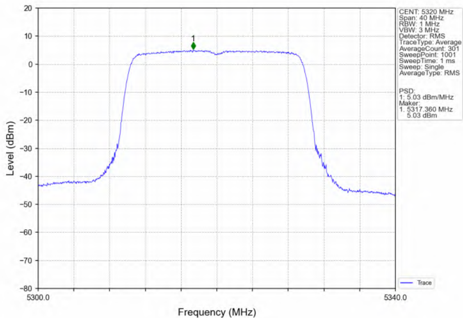
802.11ax(HEW20)_HCH_5320MHz_SU / Ant2_NTNV
