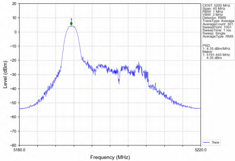
802.11ax(HEW20)_MCH_5200MHz_RU26_MIMO_NTNV
