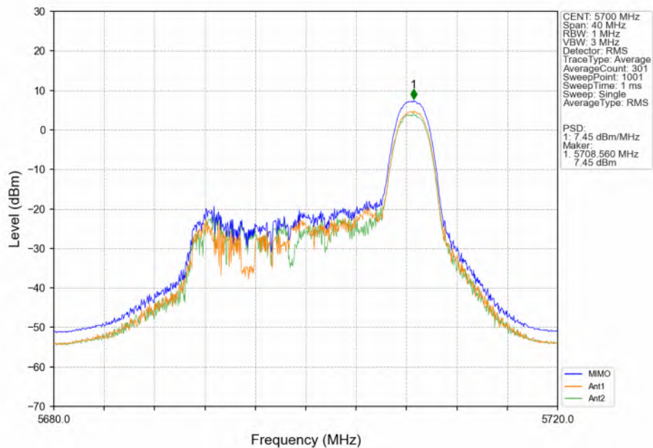
802.11ax(HEW20)_HCH_5700MHz_RU26_MIMO_NTNV
