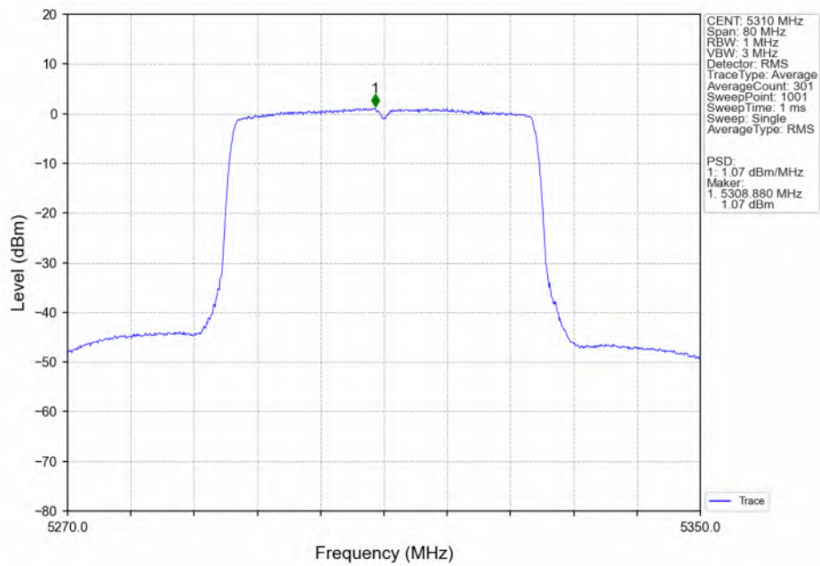
802.11ax(HEW40) HCH_5310MHz_SU / Ant2_NTNV
