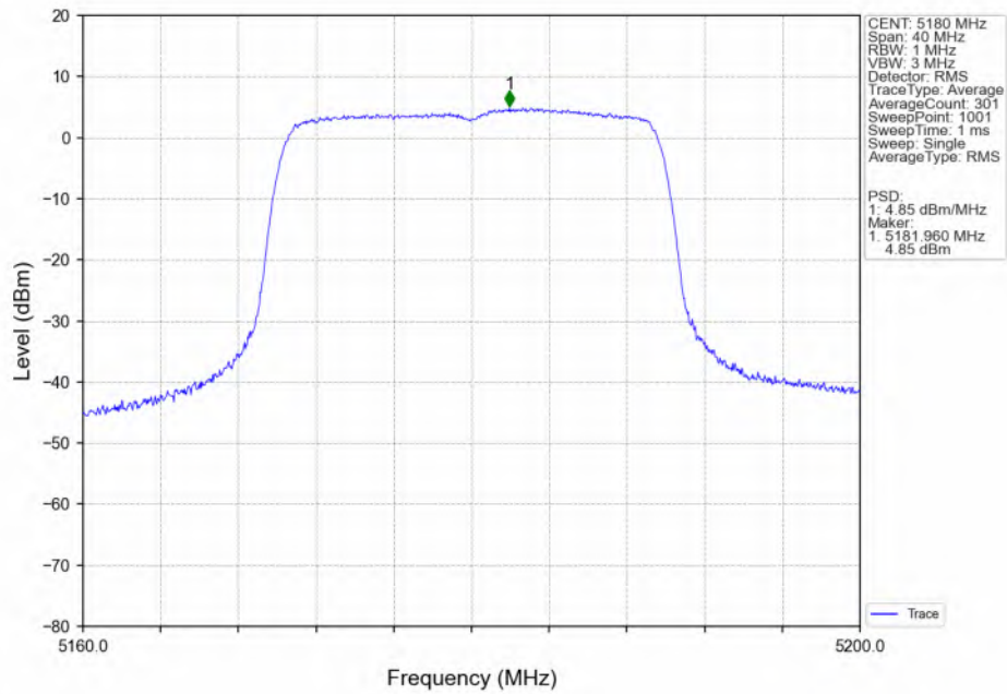
802.11ax(HEW20)_LCH_5180MHz_SU / Ant2_NTNV
