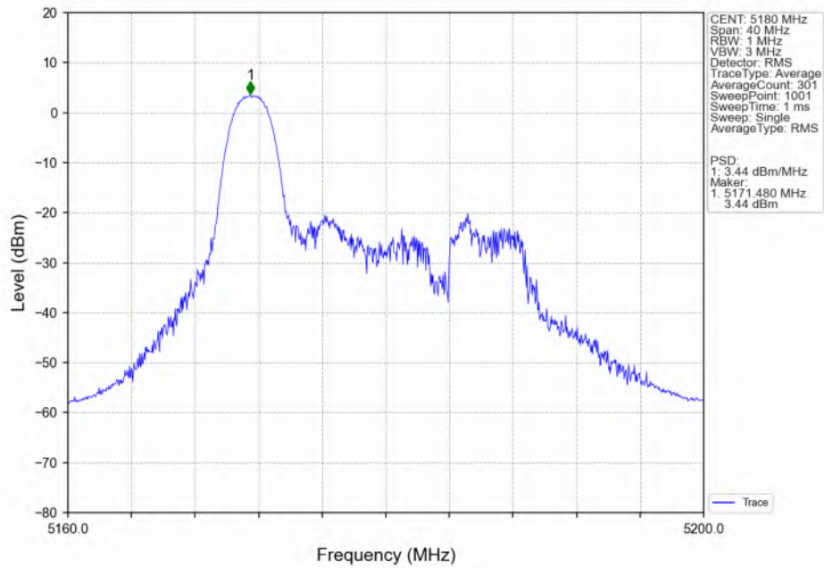
802.11ax(HEW20)_LCH_5180MHz_RU26_MIMO_NTNV
