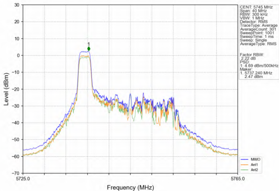
802.11ax(HEW20)_LCH_5745MHz_RU26_MIMO_NTNV
