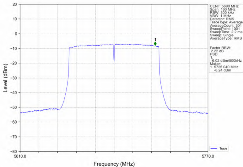
802.11ac(VHT80)_HCH_5690MHz_Ant2_NTNV
