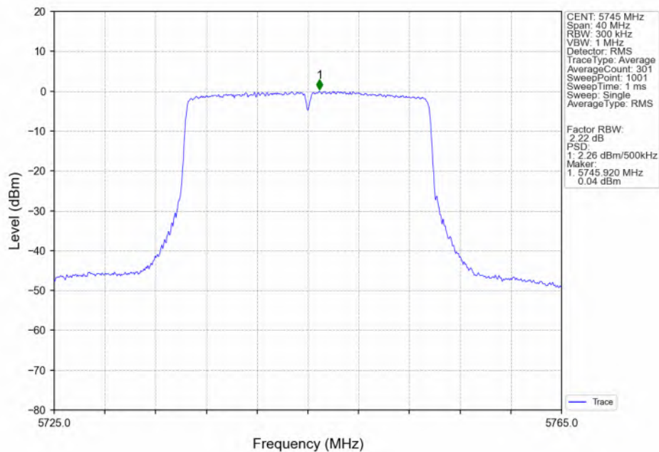
802.11ax(HEW20)_LCH_5745MHz_SU / Ant2_NTNV
