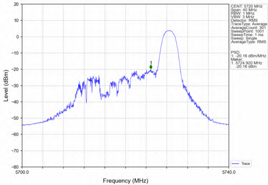
802.11ax(HEW20)_HCH_5720MHz_RU26_MIMO_NTNV
