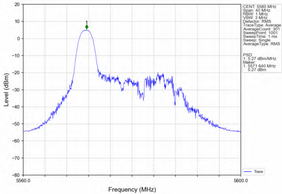
802.11ax(HEW20)_MCH_5580MHz_RU26_MIMO_NTNV
