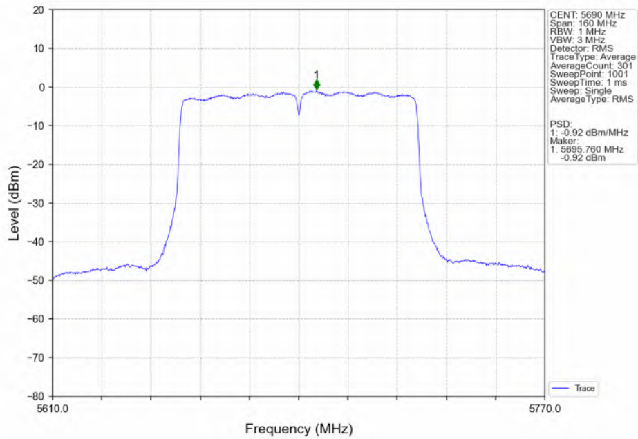
802.11ac(VHT80)_HCH_5690MHz_Ant2_NTNV
