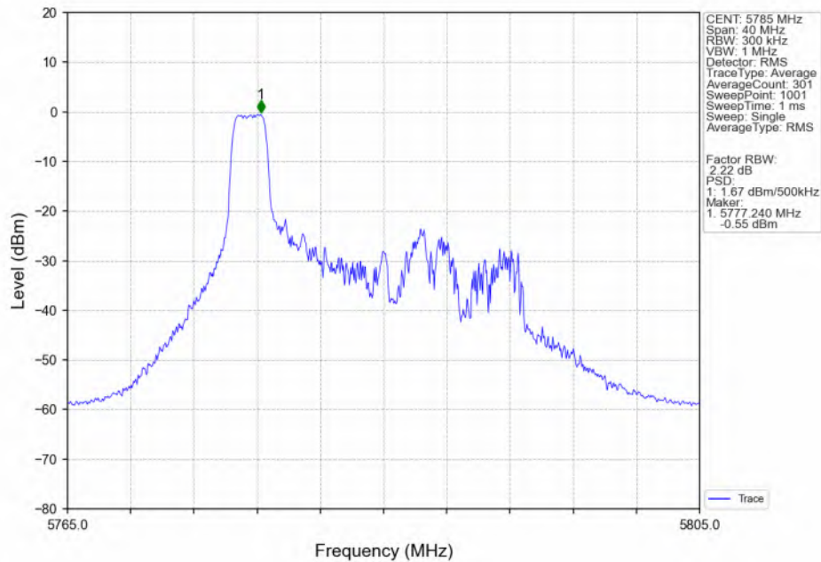
802.11ax(HEW20)_MCH_5785MHz_RU26_MIMO_NTNV
