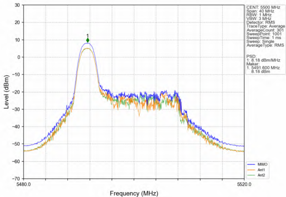
802.11ax(HEW20)_LCH_5500MHz_RU26_MIMO_NTNV
