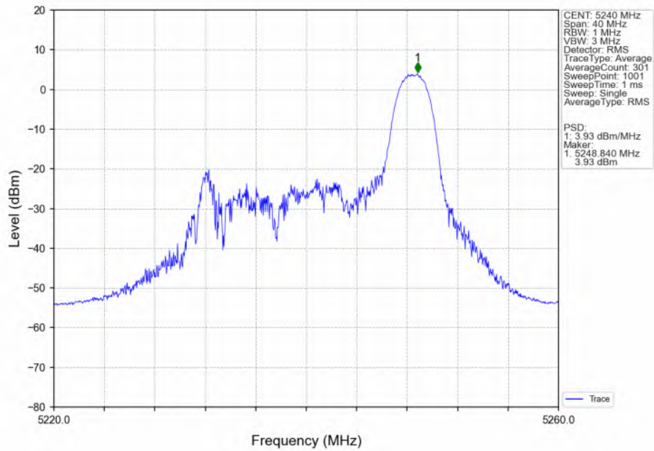
802.11ax(HEW20)_HCH_5240MHz_RU26_MIMO_NTNV
