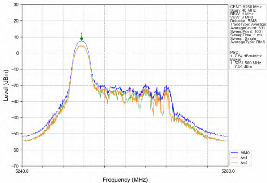
802.11ax(HEW20)_LCH_5260MHz_RU26_MIMO_NTNV
