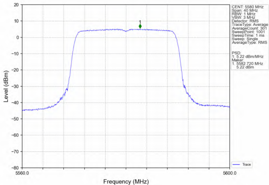
802.11ax(HEW20)_MCH_5580MHz_SU / Ant2_NTNV
