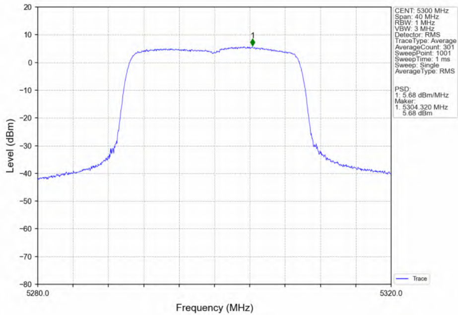
802.11ax(HEW20)_MCH_5300MHz_SU / Ant2_NTNV
