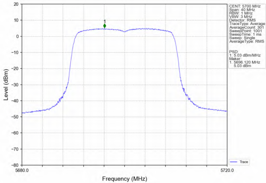
802.11ax(HEW20) HCH_5700MHz_SU / Ant2_NTNV
