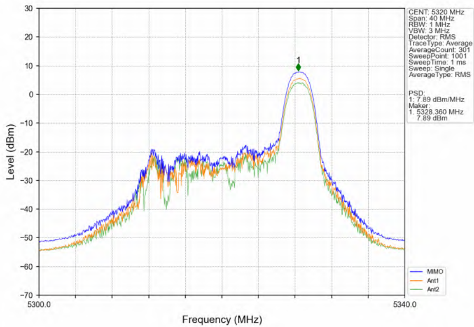
802.11ax(HEW20)_HCH_5320MHz_RU26_MIMO_NTNV
