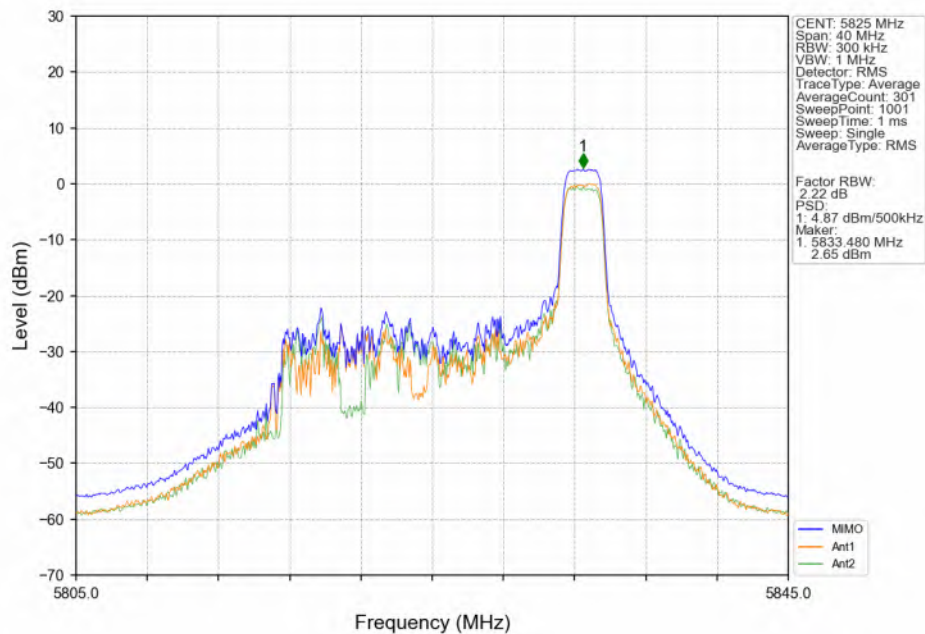
802.11ax(HEW20)_HCH_5825MHz_RU26_MIMO_NTNV
