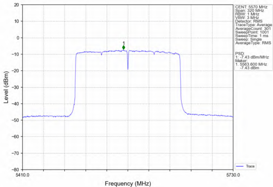
802.11ax(HEW160)_MCH_5570MHz_SU / _Ant2_NTNV
