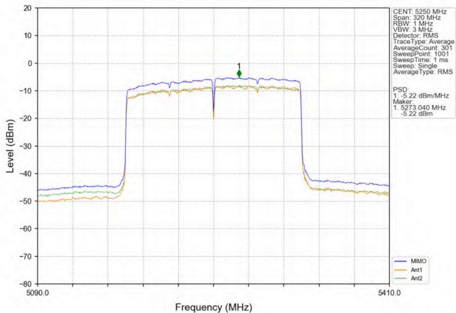
802.11ax(HEW160)_MCH_5250MHz_SU / MIMO_NTNV
