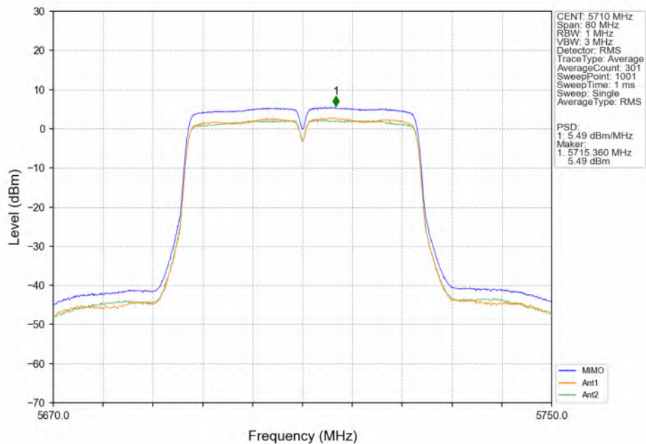
802.11n(HT40)_HCH_5710MHz_MIMO_NTNV
