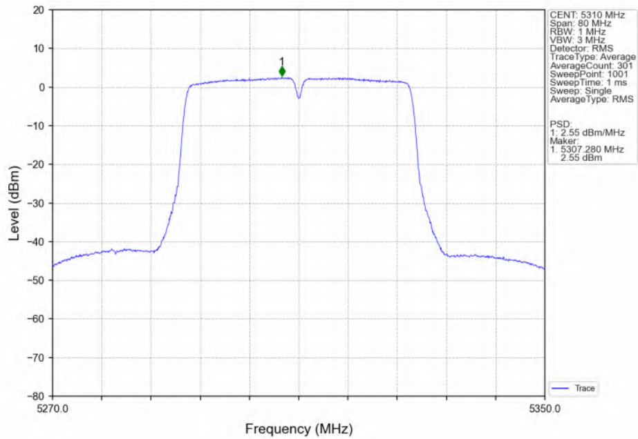
802.11n(HT40)_HCH_5310MHz_MIMO_NTNV
