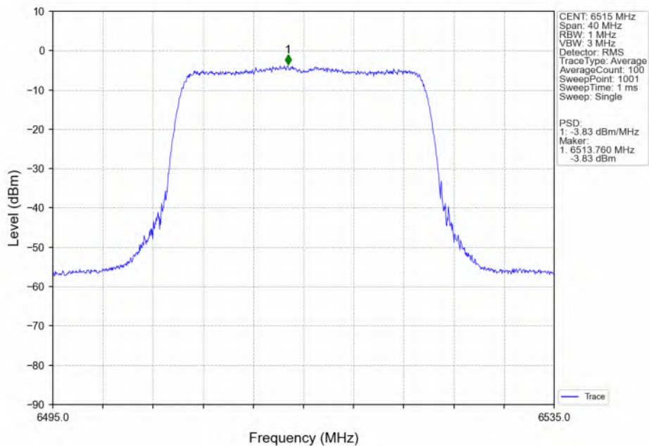
802.11ax(HEW20)_HCH_6515MHz_SU / Ant2_NTNV
