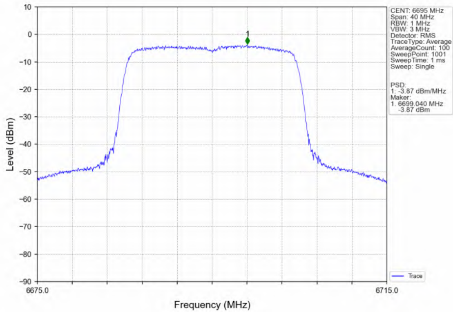
802.11ax(HEW20)_MCH_6695MHz_SU / Ant2_NTNV
