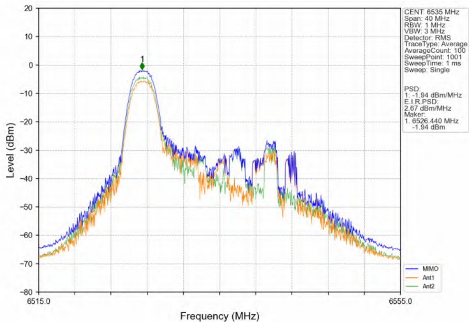
802.11ax(HEW20)_LCH_6535MHz_RU26_MIMO_NTNV
