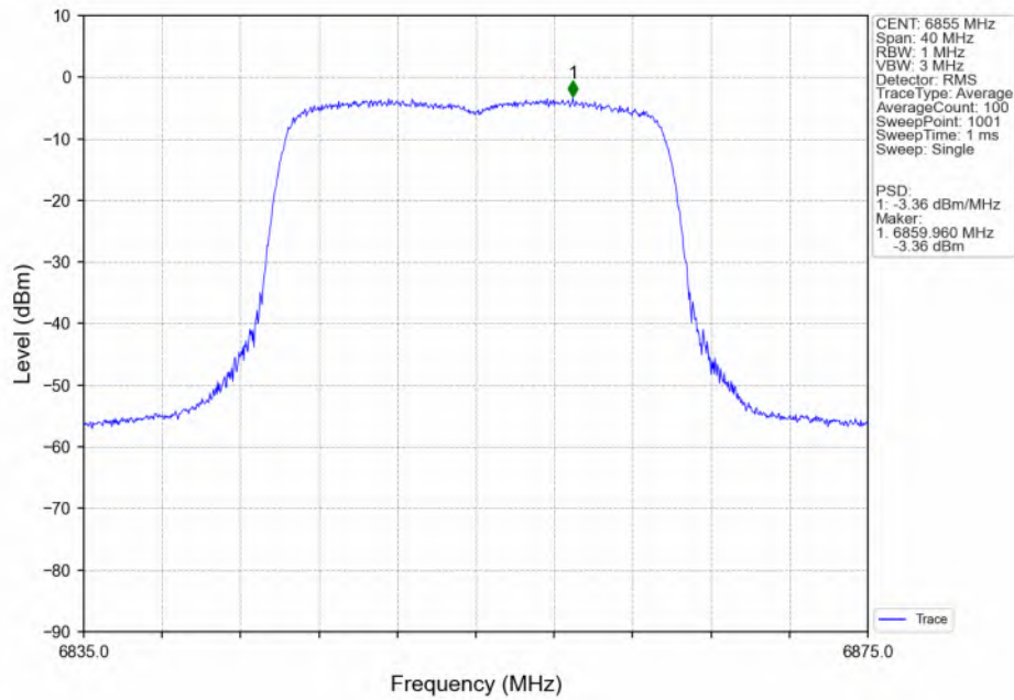
802.11ax(HEW20)_HCH_6855MHz_SU / Ant2_NTNV
