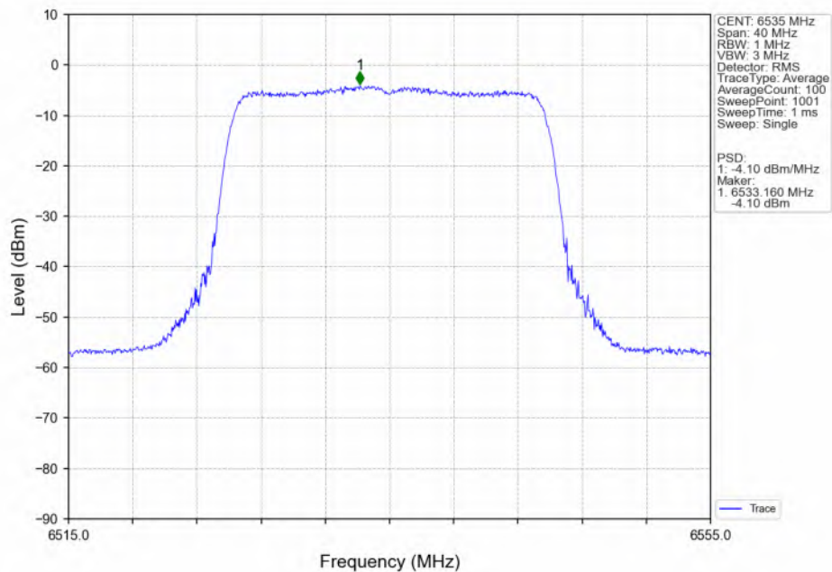
802.11ax(HEW20)_LCH_6535MHz_SU / Ant2_NTNV
