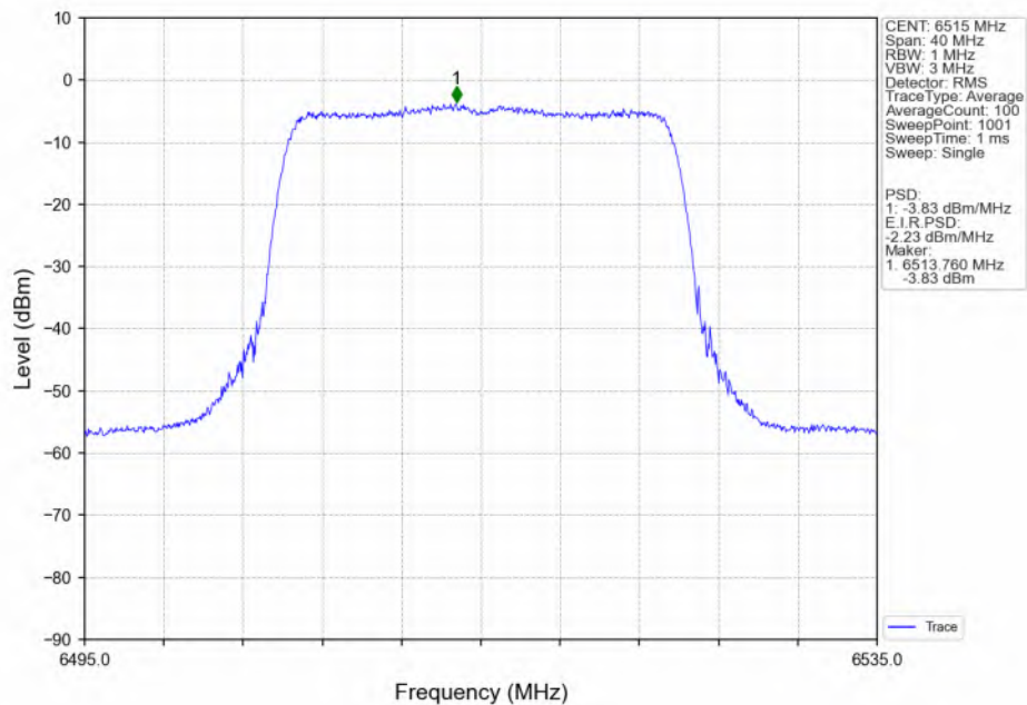
802.11ax(HEW20) HCH_6515MHz_SU / Ant2_NTNV
