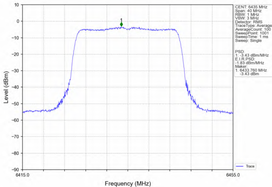
802.11ax(HEW20)_LCH_6435MHz_SU / Ant2_NTNV
