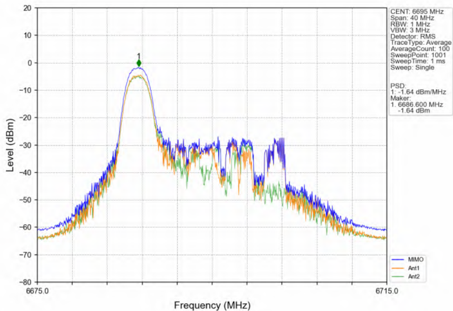
802.11ax(HEW20)_MCH_6695MHz_RU26_MIMO_NTNV
