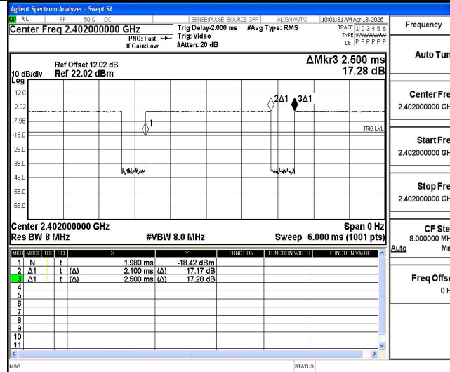
NTNV-BLE_1M-Ant1-2402
