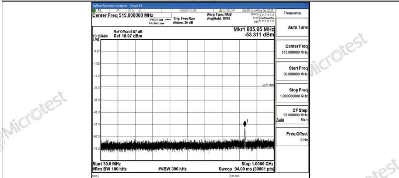
DH5_Ant1_2441_30~1000
