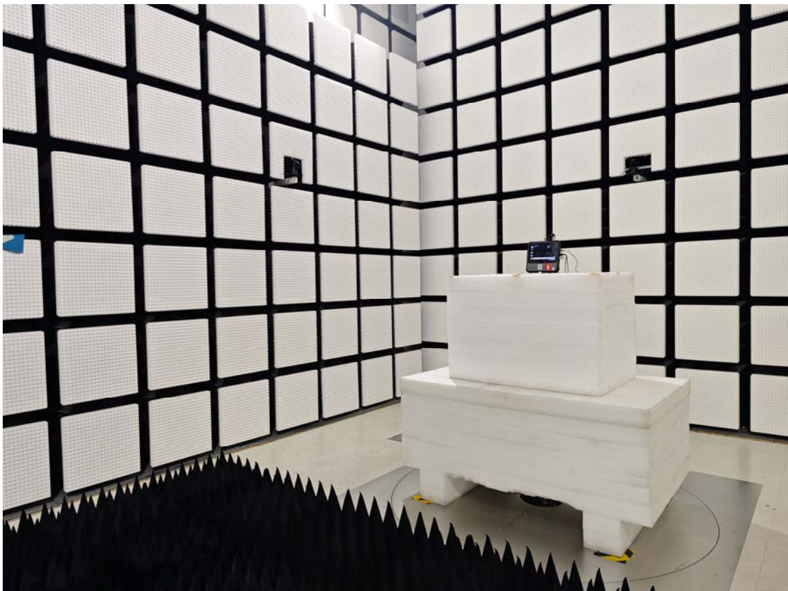
Radiated Emission Above 18-25GHz View
