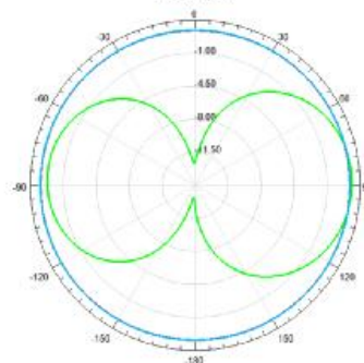
Gain Plot 2
