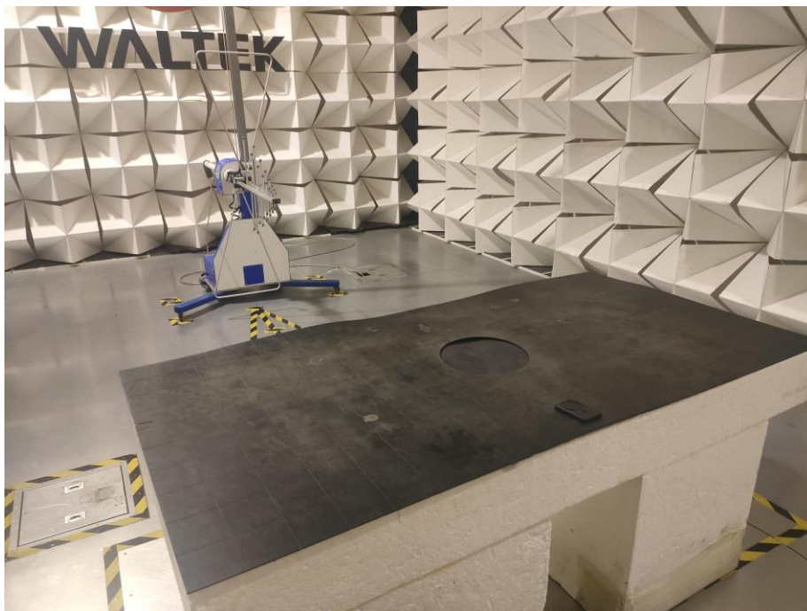
setup for BLE For above 1GHz Test Site 1#
