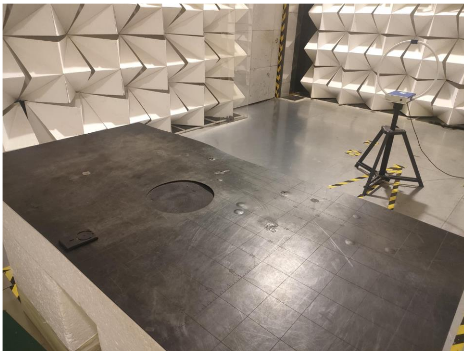
setup for BLE For 30MHz-1000MHz Test Site 2#
