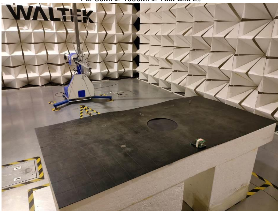
setup for WPT
