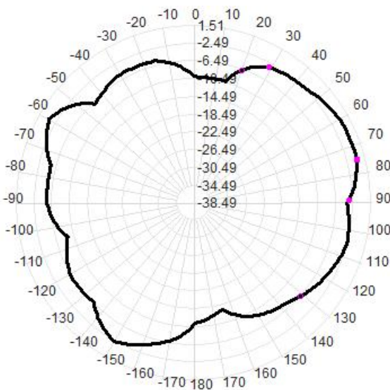
2440MHz 2D-Theta Pattern
