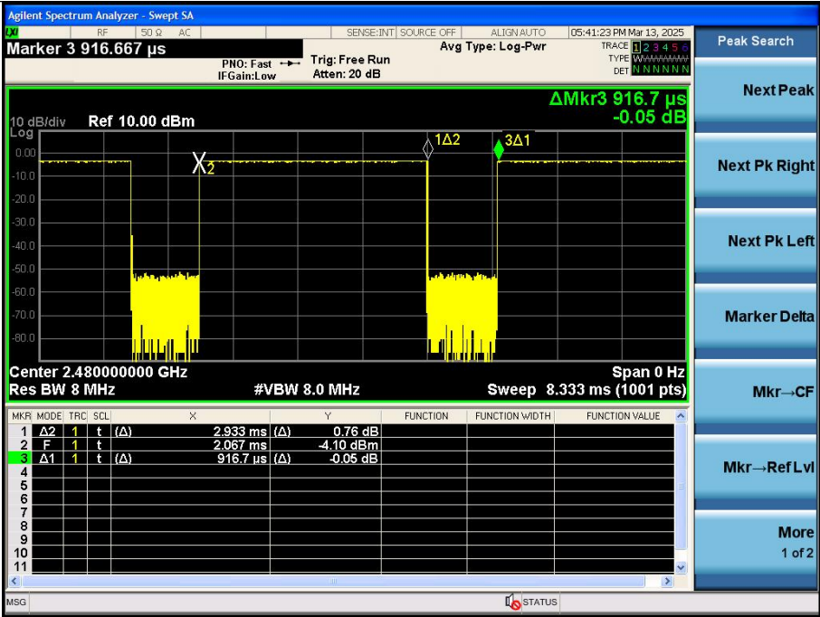
Channel 78
