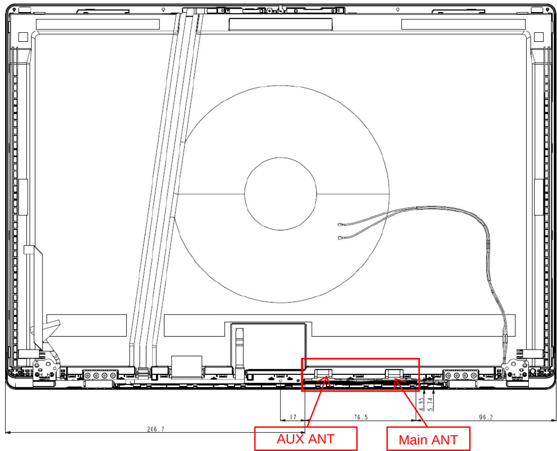
Figure 49 WLAN Combo Antenna View
