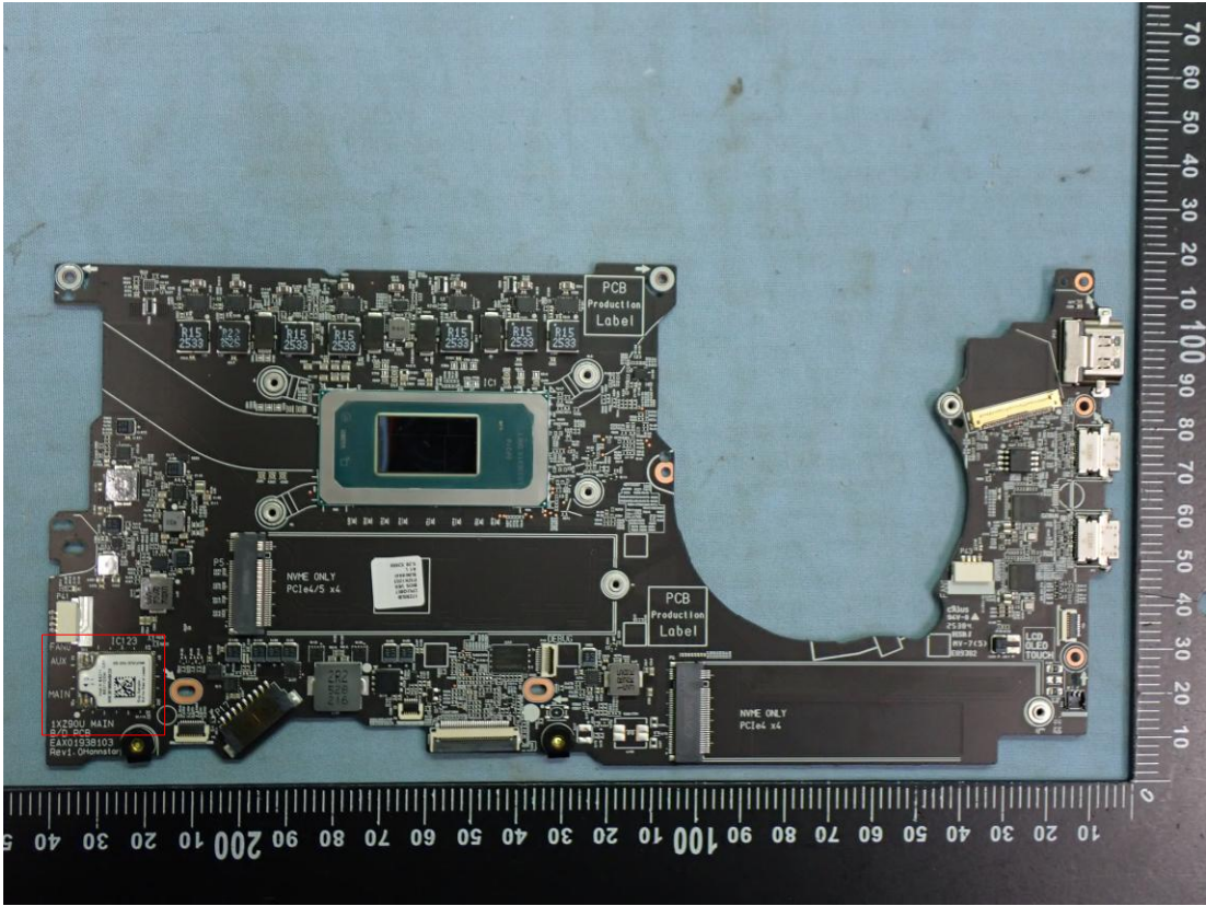
Figure 44 Main Board, Front View (WLAN Combo Card Location)
