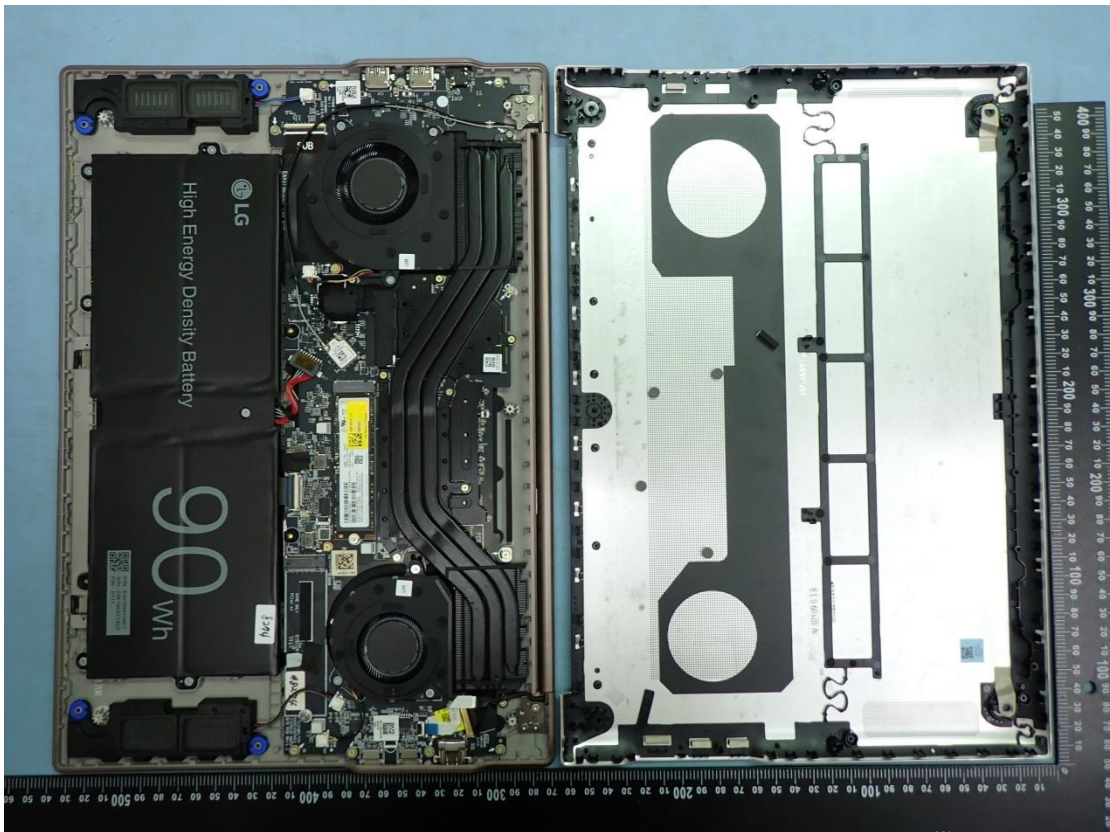
Figure 23 Internal View
