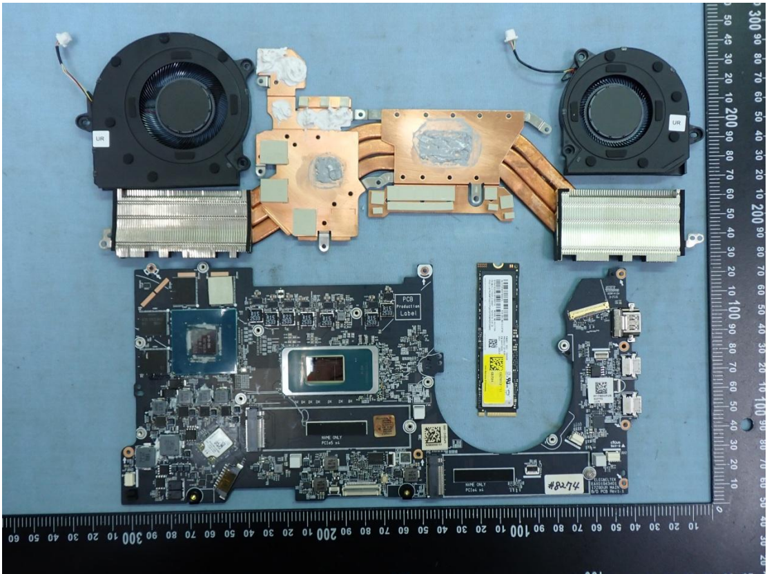
Figure 25 Internal View
