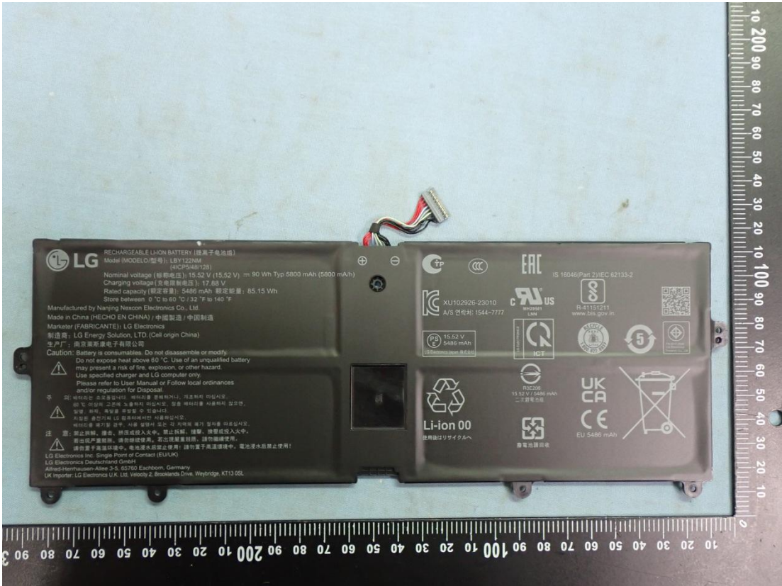
Figure 27 Battery, Back View
