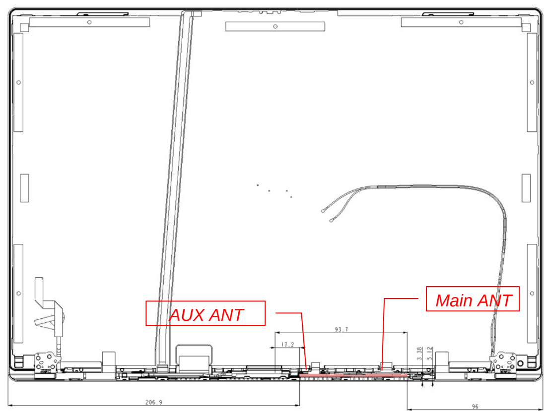
Figure 34 WLAN Combo Antenna Position
