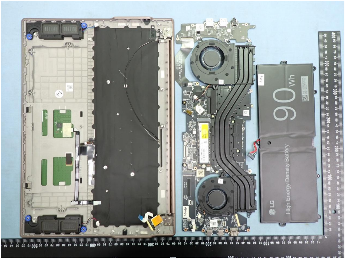
Figure 24 Internal View (Removed Component)
