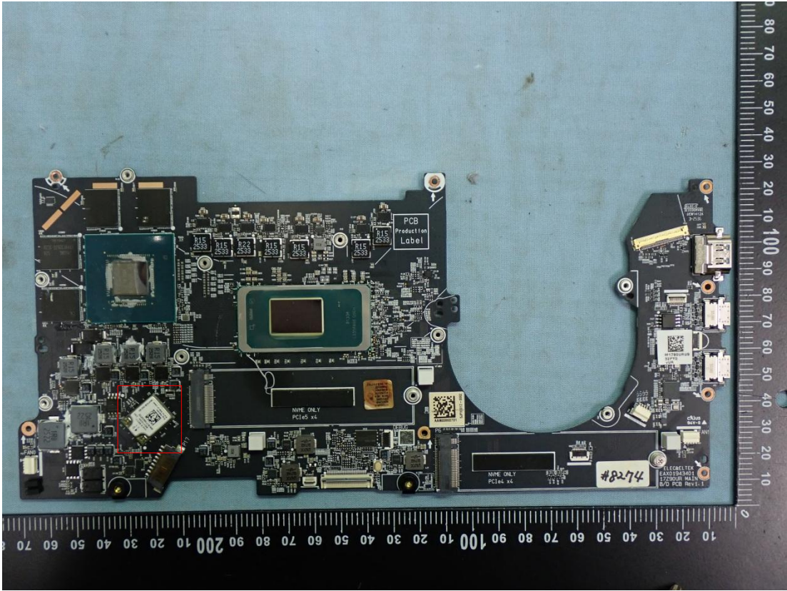
Figure 30 Main Board, Front View (WLAN Combo Card Location)
