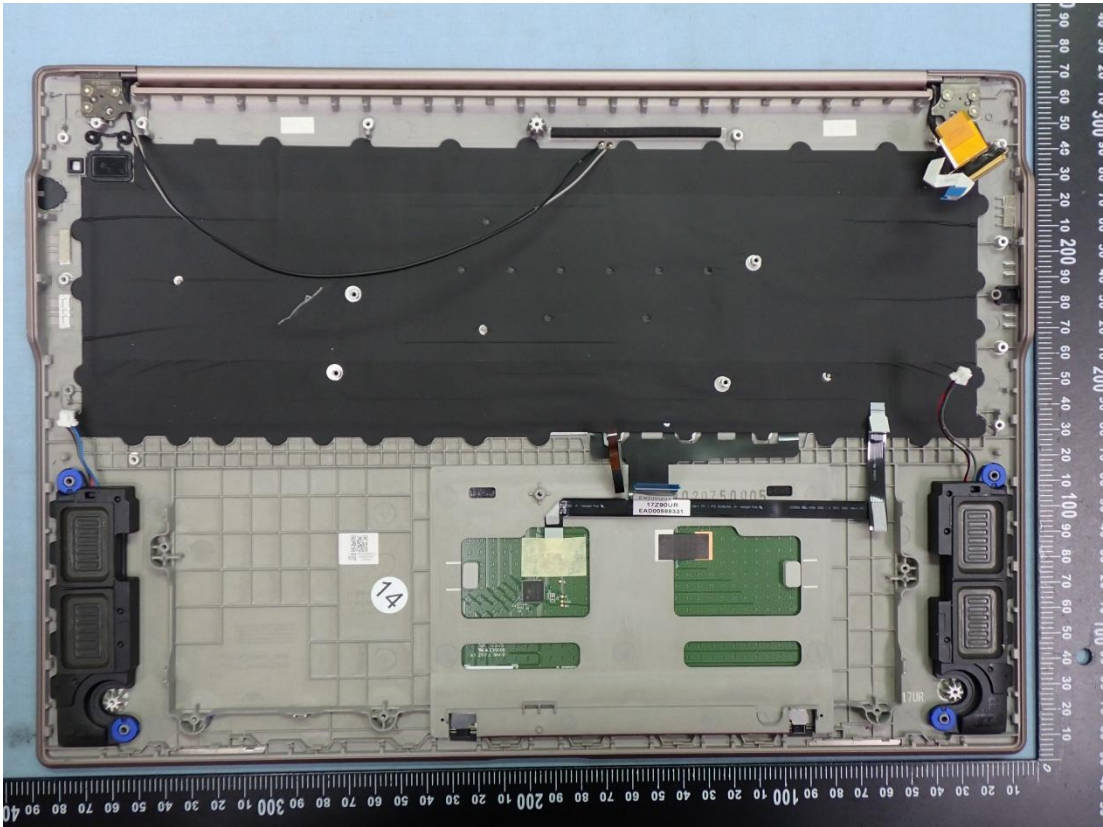
Figure 43 Internal View
