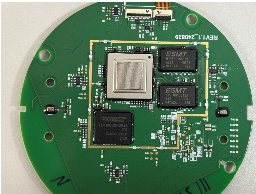
Main Board Shield can open – Rear
