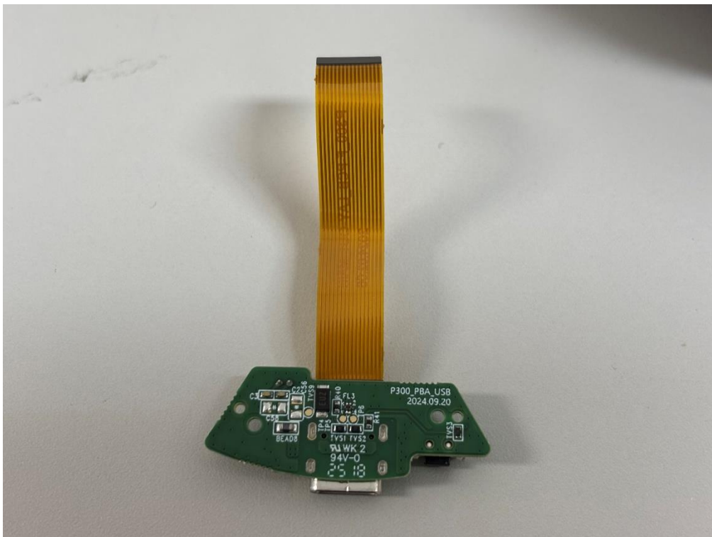
C type power Board – Rear
