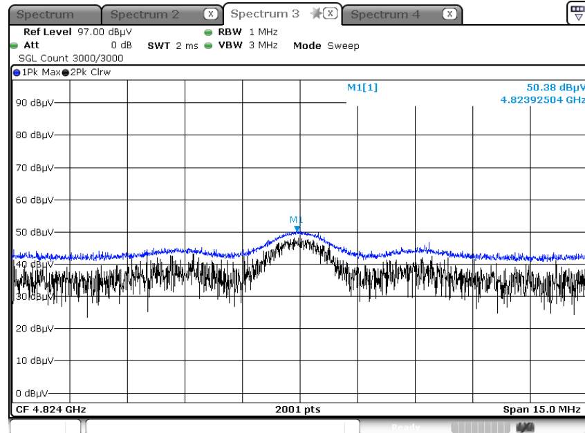
Radiated Spurious Emissions plot – Peak Result (802.11b 1 Mbps, Ch.1 2nd Harmonic, Z-V)
