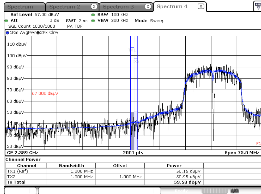
Radiated Restricted Band Edges plot – Average Result (802.11g 6Mbps, Ch.1, Z-V) (Avg Integration method Used)
