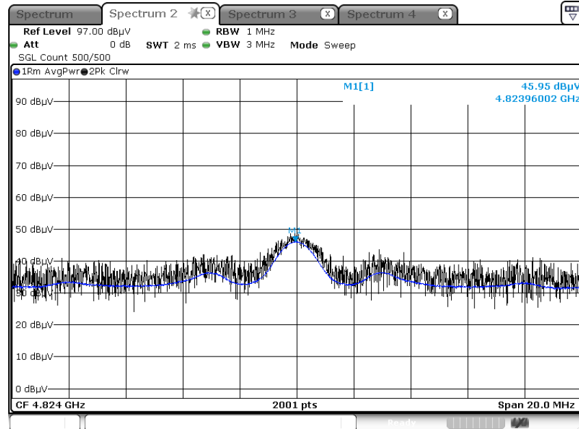
Radiated Spurious Emissions plot – Average Result (802.11b 1 Mbps, Ch.1 2nd Harmonic, Z-V)
