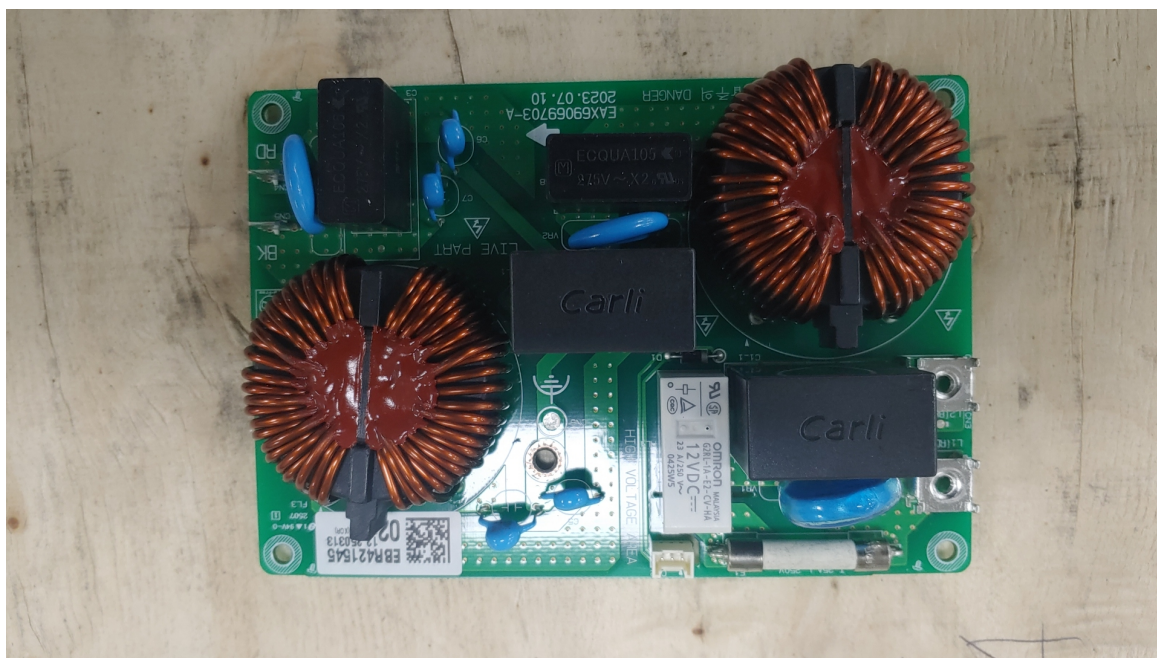
< Noise filter PCB (front) >
