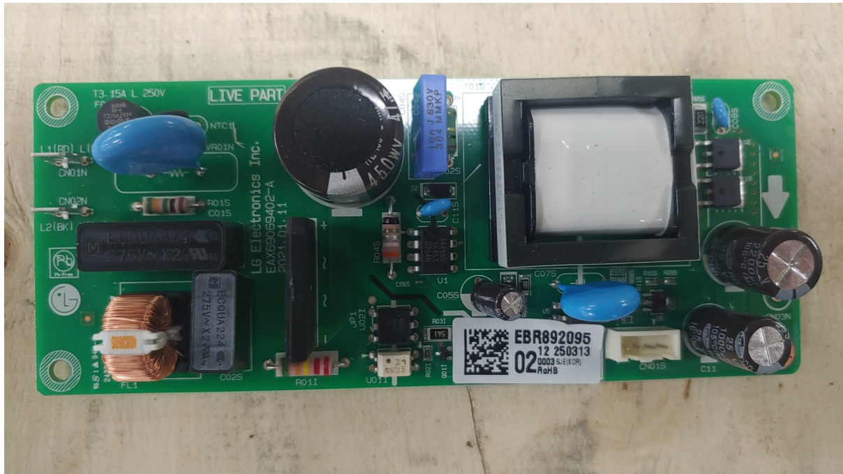
< Power PCB (front) >
