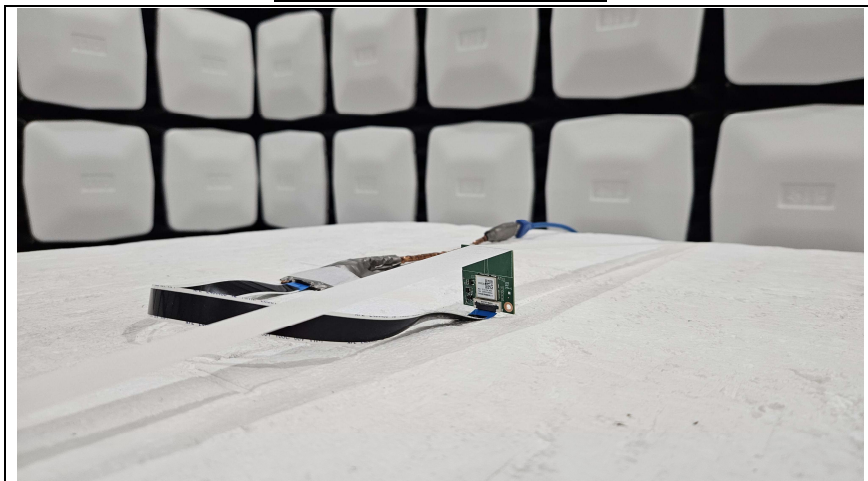
EUT Position: Y-axis
