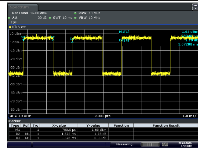
11ac_VHT40
