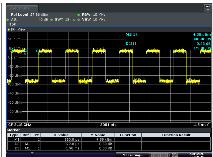
11ax_HE20
