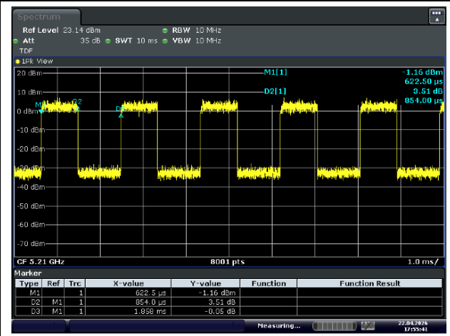
11ac_VHT80
