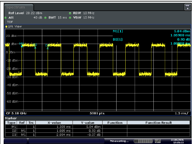
11ac_VHT20
