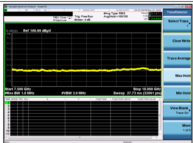
7.5 GHz ~ 18 GHz
