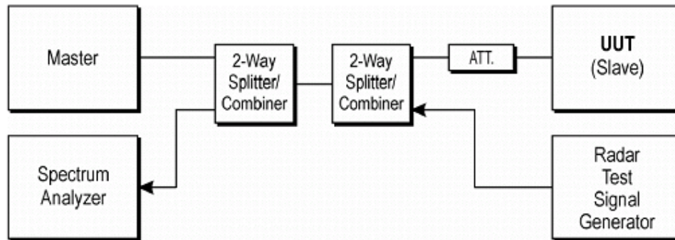
Figure 7-1. Test Setup
