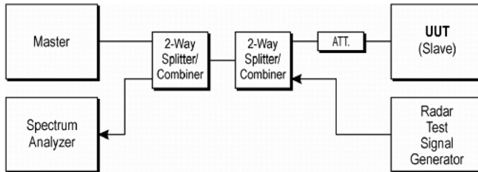
Figure 7-1. Test Setup
